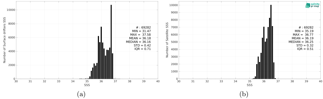
Figure 2: Histograms of SSS from Surface drifters (a) and SMAP SSS L4 OI v2 - 7 Days (ESR) (b) considering all match-up pairs per bins of 0.1 over the OTT zone Pi-MEP region and for the full satellite product period.
