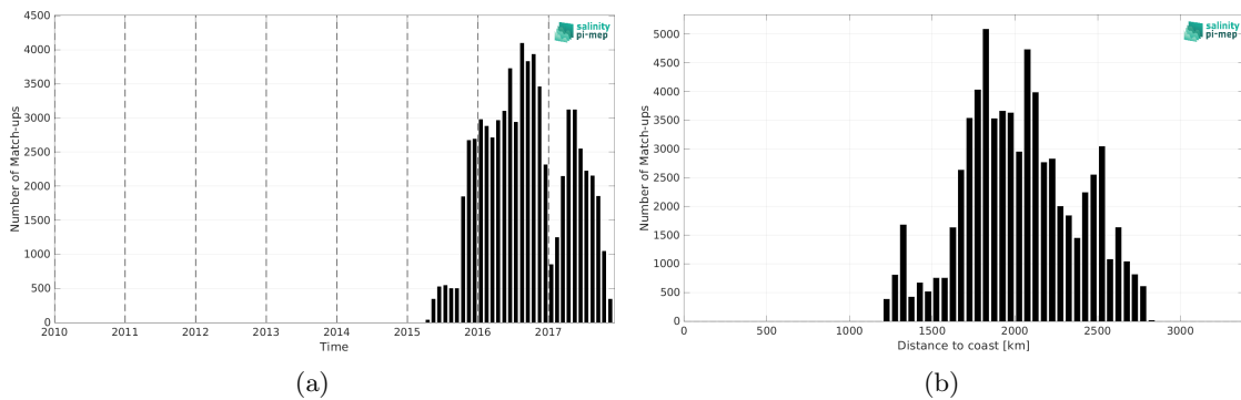
Figure 1: Number of match-ups between Surface drifters and SMAP SSS L4 OI v2 - 7 Days (ESR) SSS as a function of time (a) and as function of the distance to coast (b) over the OTT zone Pi-MEP region and for the full satellite product period.
