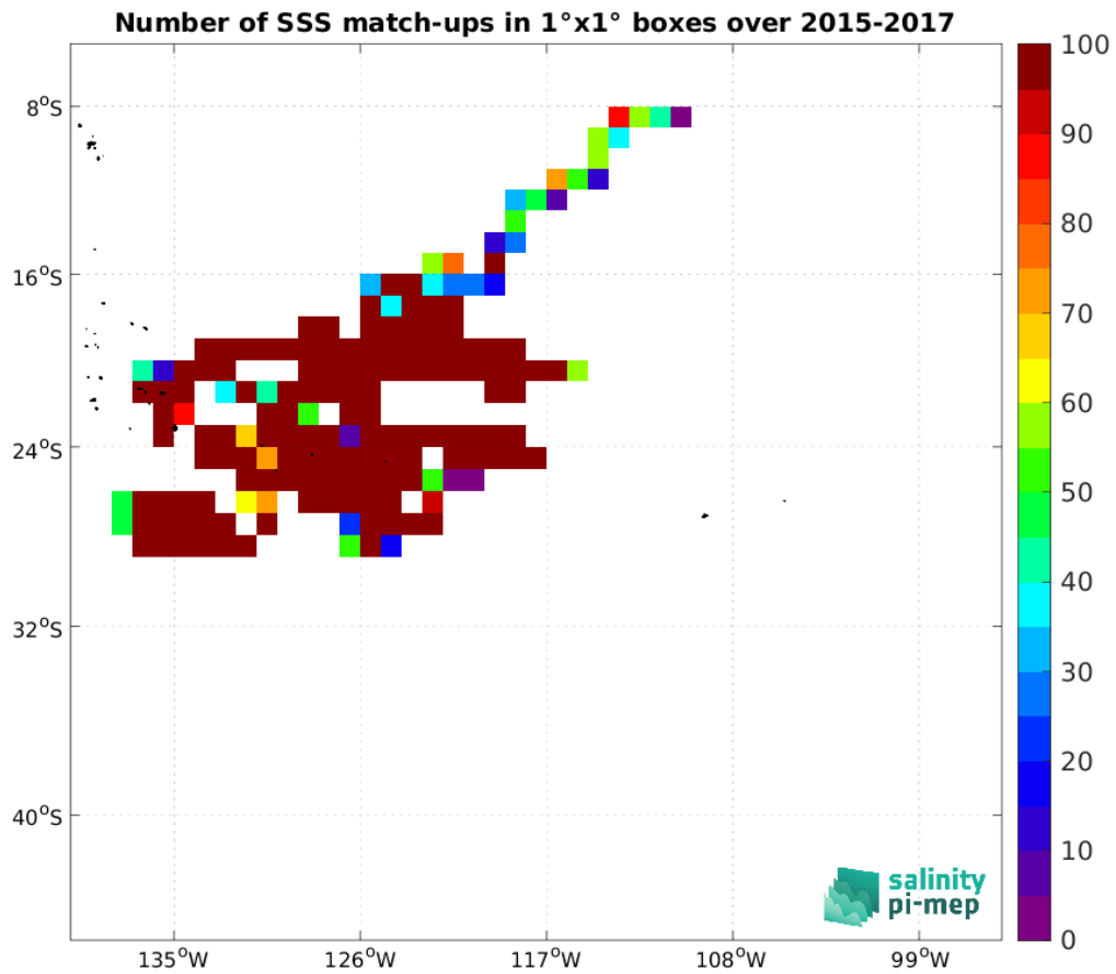
Figure 3: Number of SSS match-ups between Surface drifters SSS and the SMAP SSS L4 OI v2 - 7 Days (ESR) SSS product for the OTT zone Pi-MEP region over 1^\circ \times 1^\circ boxes and for the full satellite product period.
