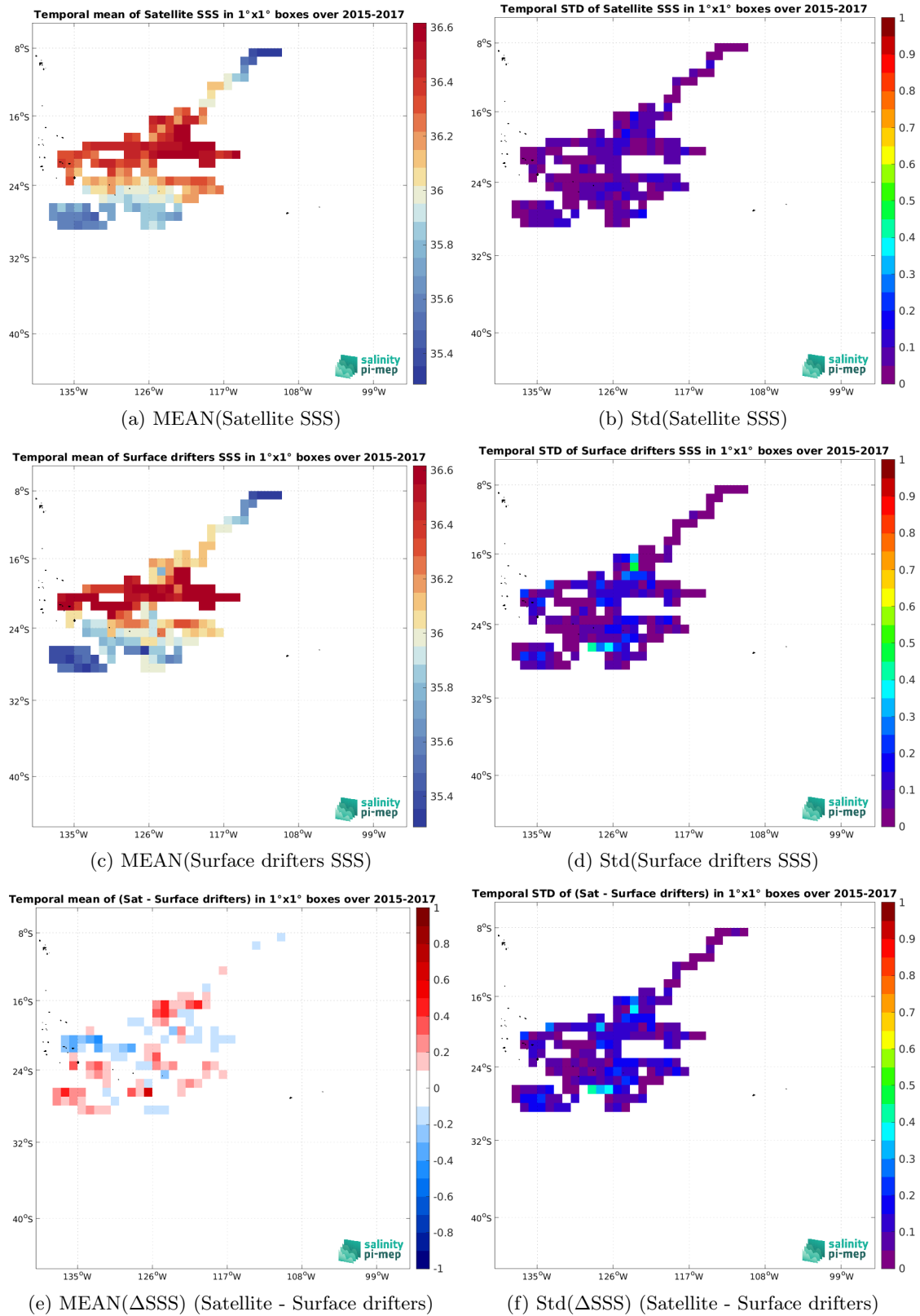
Figure 5: Temporal mean (left) and Std (right) of SSS from SMAP SSS L4 OI v2 - 7 Days (ESR) (top), Surface drifters (middle), and of \Delta SSS (Satellite - Surface drifters). Only match-up pairs are used to generate these maps.
