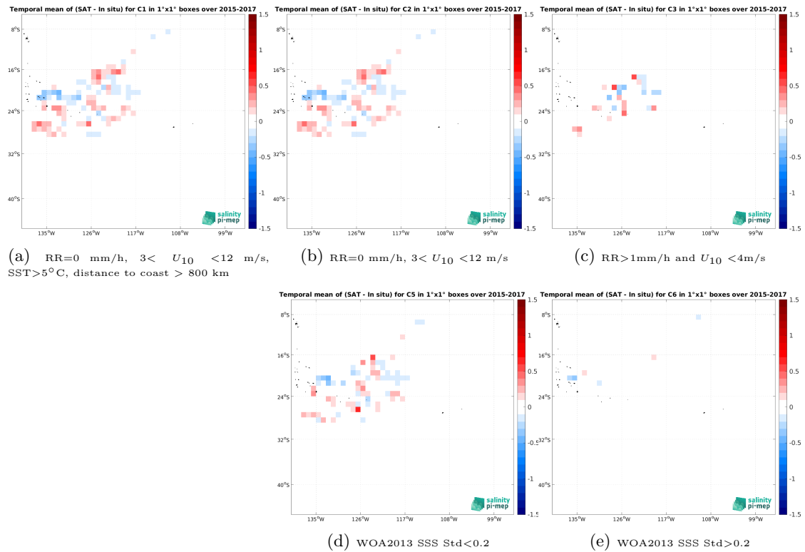
Figure 11: Temporal mean gridded over spatial boxes of size 1^\circ \times 1^\circ of \Delta SSS (SMAP SSS L4 OI v2 - 7 Days (ESR) - Surface drifters) for 5 different subdatasets corresponding to:RR=0 mm/h, 3 < U_{10} < 12 m/s, SST > 5^\circ\text{C} , distance to coast > 800 km (a), RR=0 mm/h, 3 < U_{10} < 12 m/s (b), RR > 1 mm/h and U_{10} < 4 m/s (c), WOA2013 SSS Std < 0.2 (d), WOA2013 SSS Std > 0.2 (e).
