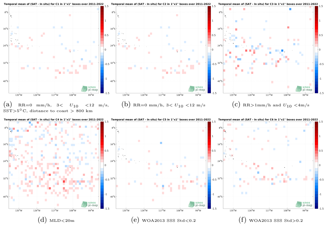
Figure 12: Temporal mean gridded over spatial boxes of size 1^\circ \times 1^\circ of \Delta SSS (SMAP SSS L4 OI v2 - 7 Days (ESR) - Argo) for 6 different subdatasets corresponding to:RR=0 mm/h, 3 < U_{10} < 12 m/s, SST >5^\circ C, distance to coast > 800 km (a), RR=0 mm/h, 3 < U_{10} < 12 m/s (b), RR >1 mm/h and U_{10} < 4 m/s (c),MLD <20 m (d),WOA2013 SSS Std <0.2 (e),WOA2013 SSS Std >0.2 (f).
