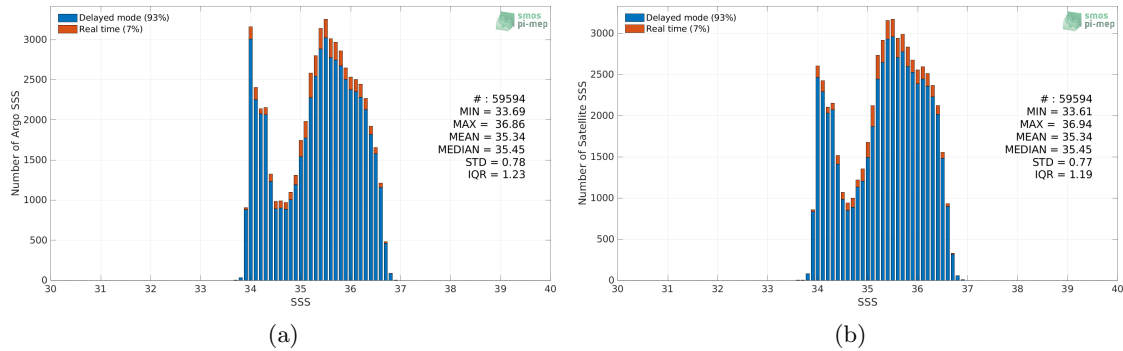
Figure 2: Histograms of SSS from Argo (a) and SMAP SSS L4 OI v2 - 7 Days (ESR) (b) considering all match-up pairs per bins of 0.1 over the OTT zone Pi-MEP region and for the full satellite product period.
