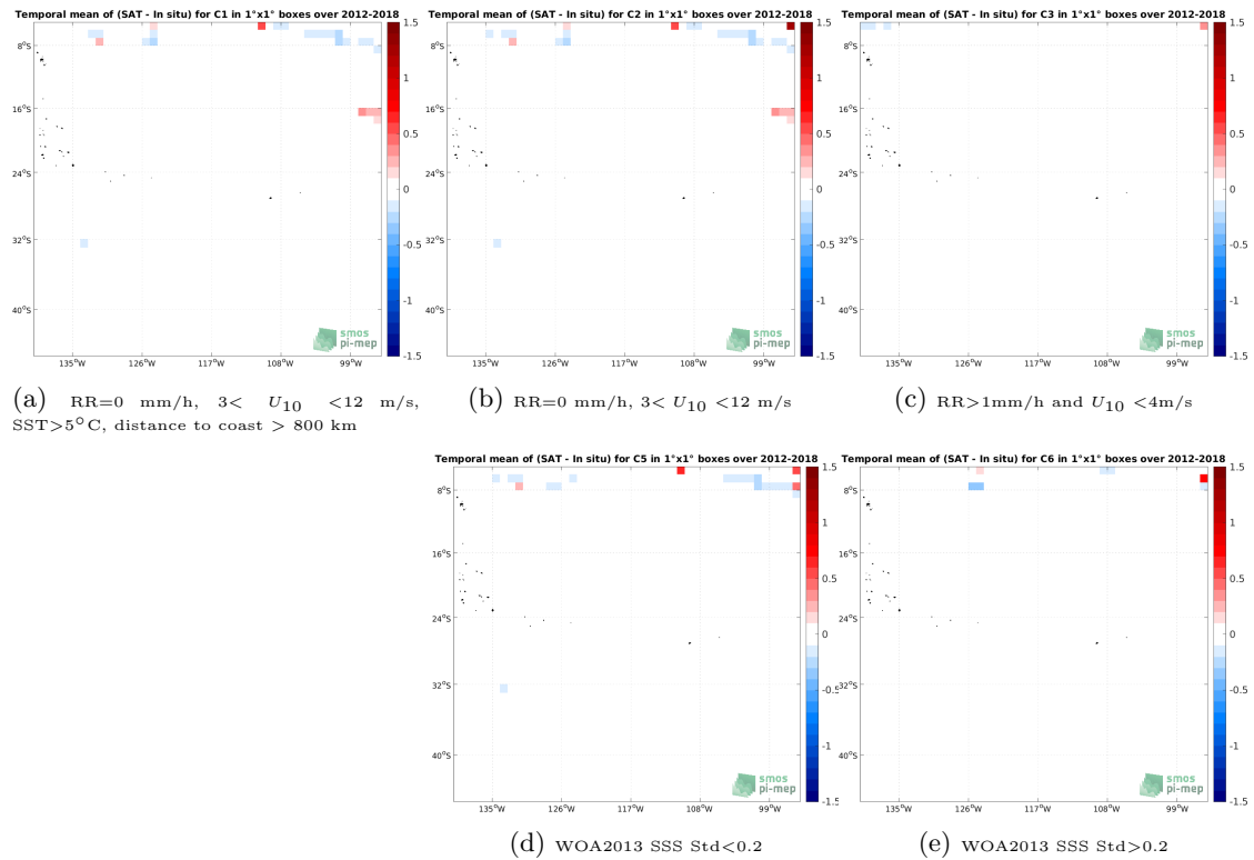
Figure 12: Temporal mean gridded over spatial boxes of size 1^\circ \times 1^\circ of \Delta SSS (SMAP SSS L4 OI v2 - Monthly (IPRC) - TSG (SAMOS)) for 5 different subdatasets corresponding to:RR=0 mm/h, 3 < U_{10} < 12 m/s, SST >5^\circ C, distance to coast > 800 km (a), RR=0 mm/h, 3 < U_{10} < 12 m/s (b), RR >1 mm/h and U_{10} < 4 m/s (c), WOA2013 SSS Std <0.2 (d), WOA2013 SSS Std >0.2 (e).
