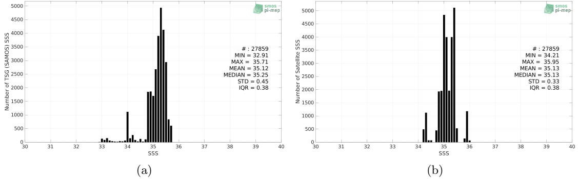
Figure 2: Histograms of SSS from TSG (SAMOS) (a) and SMAP SSS L4 OI v2 - Monthly (IPRC) (b) considering all match-up pairs per bins of 0.1 over the OTT zone Pi-MEP region and for the full satellite product period.
