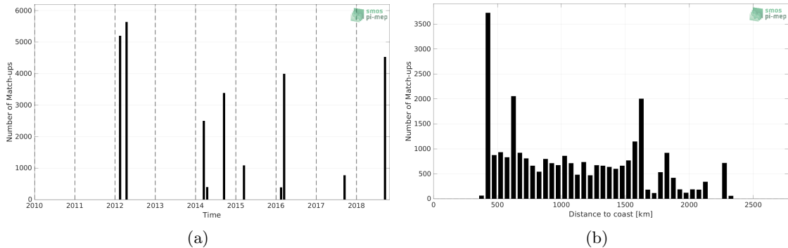
Figure 1: Number of match-ups between TSG (SAMOS) and SMAP SSS L4 OI v2 - Monthly (IPRC) SSS as a function of time (a) and as function of the distance to coast (b) over the OTT zone Pi-MEP region and for the full satellite product period.
