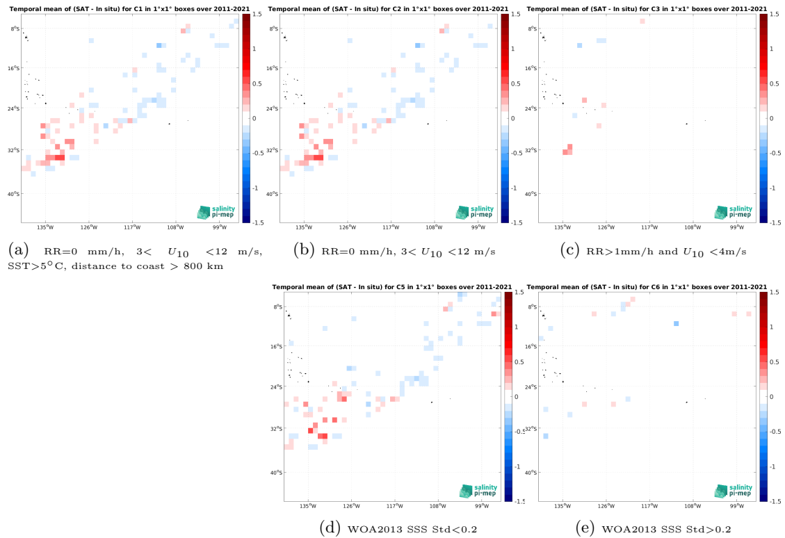
Figure 12: Temporal mean gridded over spatial boxes of size 1^\circ \times 1^\circ of \Delta SSS (SMAP SSS L4 OI v2 - Monthly (IPRC) - TSG (LEGOS-DM)) for 5 different subdatasets corresponding to:RR=0 mm/h, 3 < U_{10} < 12 m/s, SST >5^\circ C, distance to coast > 800 km (a), RR=0 mm/h, 3 < U_{10} < 12 m/s (b), RR >1 mm/h and U_{10} < 4 m/s (c), WOA2013 SSS Std <0.2 (d), WOA2013 SSS Std >0.2 (e).
