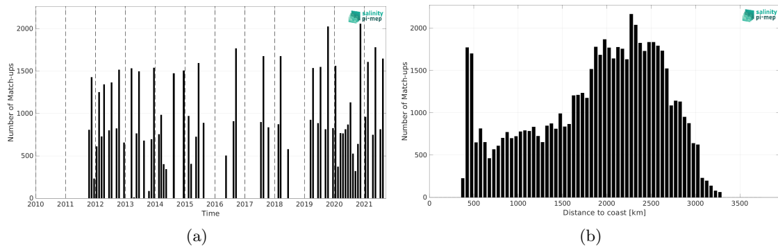
Figure 1: Number of match-ups between TSG (LEGOS-DM) and SMAP SSS L4 OI v2 - Monthly (IPRC) SSS as a function of time (a) and as function of the distance to coast (b) over the OTT zone Pi-MEP region and for the full satellite product period.
