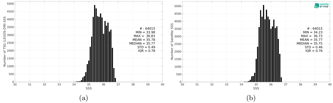
Figure 2: Histograms of SSS from TSG (LEGOS-DM) (a) and SMAP SSS L4 OI v2 - Monthly (IPRC) (b) considering all match-up pairs per bins of 0.1 over the OTT zone Pi-MEP region and for the full satellite product period.
