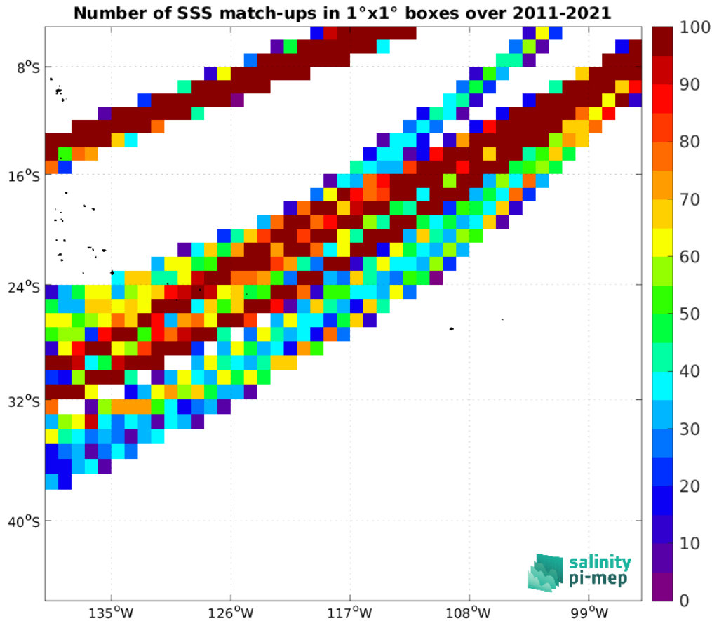
Figure 4: Number of SSS match-ups between TSG (LEGOS-DM) SSS and the SMAP SSS L4 OI v2 - Monthly (IPRC) SSS product for the OTT zone Pi-MEP region over 1^\circ \times 1^\circ boxes and for the full satellite product period.
