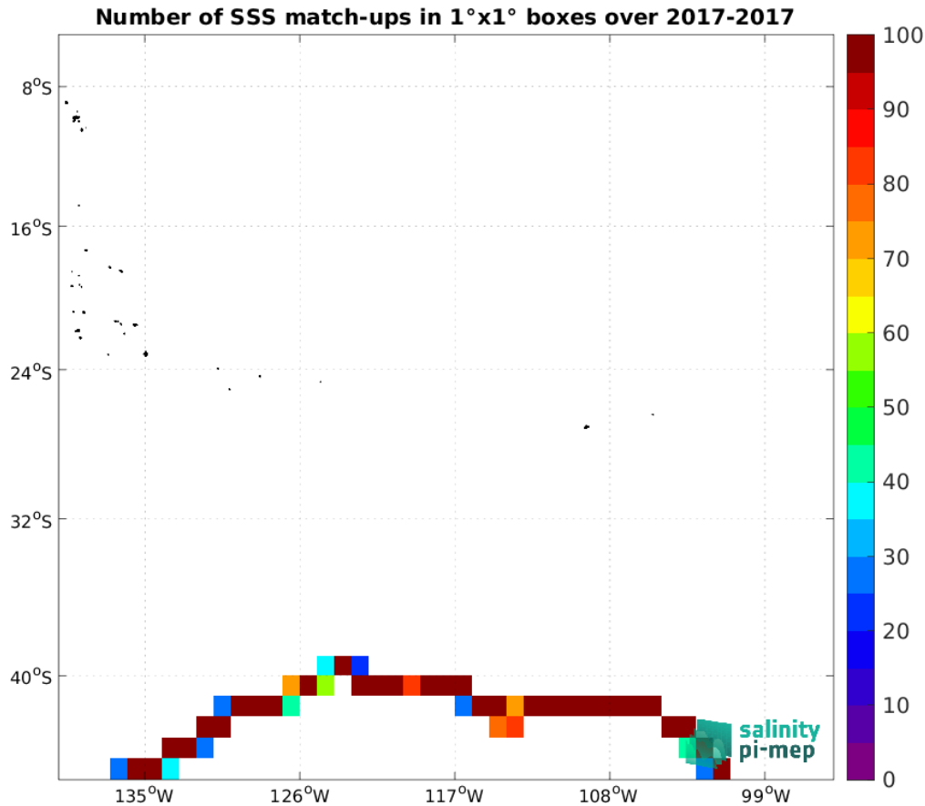
Figure 4: Number of SSS match-ups between TSG (GOSUD-Sailing-ship) SSS and the SMAP SSS L4 OI v2 - Monthly (IPRC) SSS product for the OTT zone Pi-MEP region over 1^\circ \times 1^\circ boxes and for the full satellite product period.
