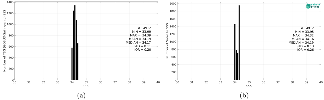
Figure 2: Histograms of SSS from TSG (GOSUD-Sailing-ship) (a) and SMAP SSS L4 OI v2 - Monthly (IPRC) (b) considering all match-up pairs per bins of 0.1 over the OTT zone Pi-MEP region and for the full satellite product period.
