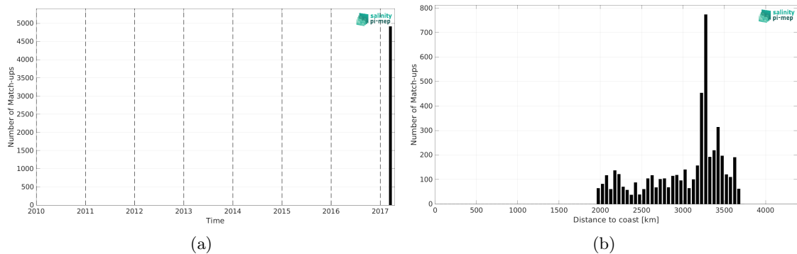
Figure 1: Number of match-ups between TSG (GOSUD-Sailing-ship) and SMAP SSS L4 OI v2 - Monthly (IPRC) SSS as a function of time (a) and as function of the distance to coast (b) over the OTT zone Pi-MEP region and for the full satellite product period.
