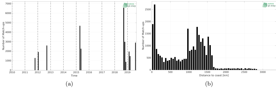
Figure 1: Number of match-ups between TSG (GOSUD-Research-vessel) and SMAP SSS L4 OI v2 - Monthly (IPRC) SSS as a function of time (a) and as function of the distance to coast (b) over the OTT zone Pi-MEP region and for the full satellite product period.
