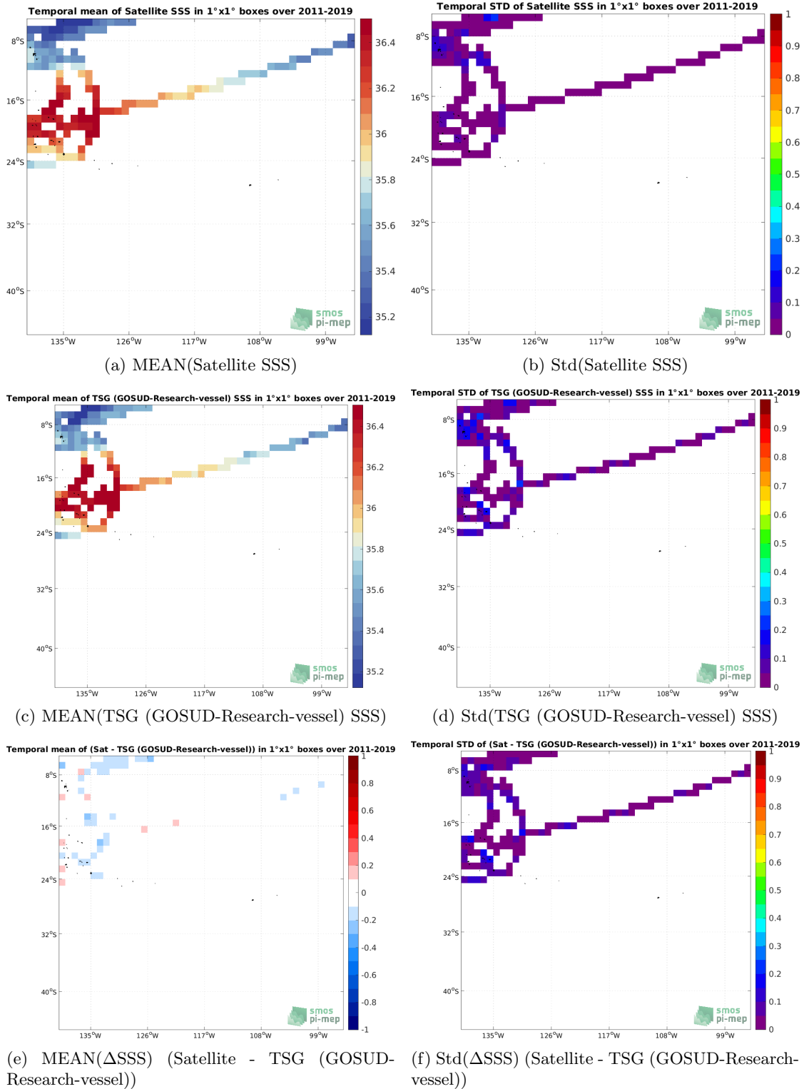
Figure 6: Temporal mean (left) and Std (right) of SSS from SMAP SSS L4 OI v2 - Monthly (IPRC) (top), TSG (GOSUD-Research-vessel) (middle), and of \Delta SSS (Satellite - TSG (GOSUD-Research-vessel)). Only match-up pairs are used to generate these maps.
