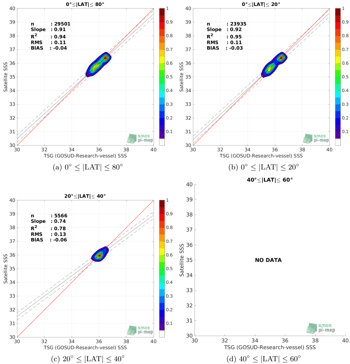
Figure 9: Contour maps of the concentration of SMAP SSS L4 OI v2 - Monthly (IPRC) SSS (y-axis) versus TSG (GOSUD-Research-vessel) SSS (x-axis) at match-up pairs for different latitude bands. For each plot, the red line shows x=y . The black thin and dashed lines indicate a linear fit through the data cloud and the \pm 95\% confidence levels, respectively. The number match-up pairs n , the slope and R^2 coefficient of the linear fit, the root mean square (RMS) and the mean bias between satellite and in situ data are indicated for each latitude band in each plots.
