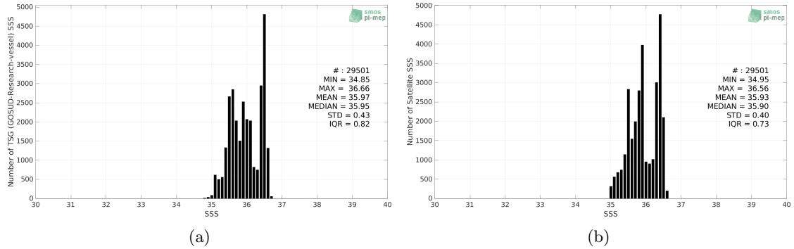
Figure 2: Histograms of SSS from TSG (GOSUD-Research-vessel) (a) and SMAP SSS L4 OI v2 - Monthly (IPRC) (b) considering all match-up pairs per bins of 0.1 over the OTT zone Pi-MEP region and for the full satellite product period.
