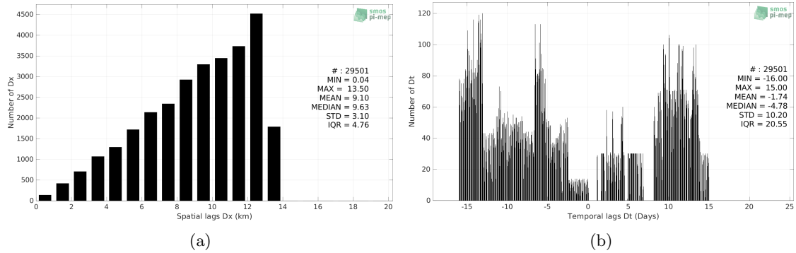
Figure 5: Histograms of the spatial (a) and temporal (b) lags between the location/time of the TSG (GOSUD-Research-vessel) measurement and the date of the corresponding SMAP SSS L4 OI v2 - Monthly (IPRC) SSS pixel.
