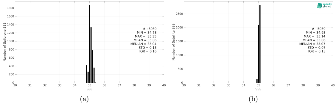
Figure 2: Histograms of SSS from Saildrone (a) and SMAP SSS L4 OI v2 - Monthly (IPRC) (b) considering all match-up pairs per bins of 0.1 over the OTT zone Pi-MEP region and for the full satellite product period.
