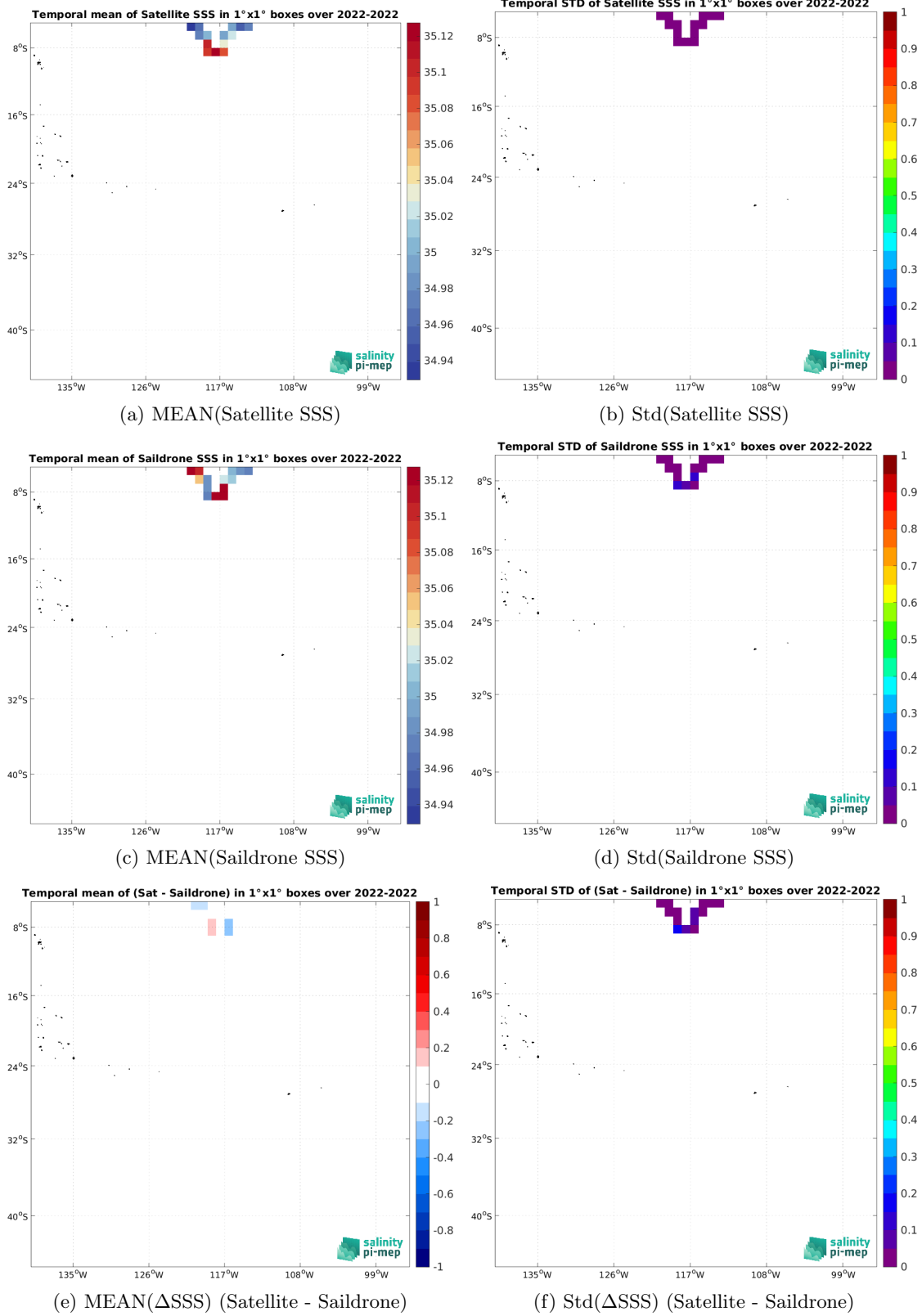
Figure 6: Temporal mean (left) and Std (right) of SSS from SMAP SSS L4 OI v2 - Monthly (IPRC) (top), Saildrone (middle), and of \Delta SSS (Satellite - Saildrone). Only match-up pairs are used to generate these maps.
