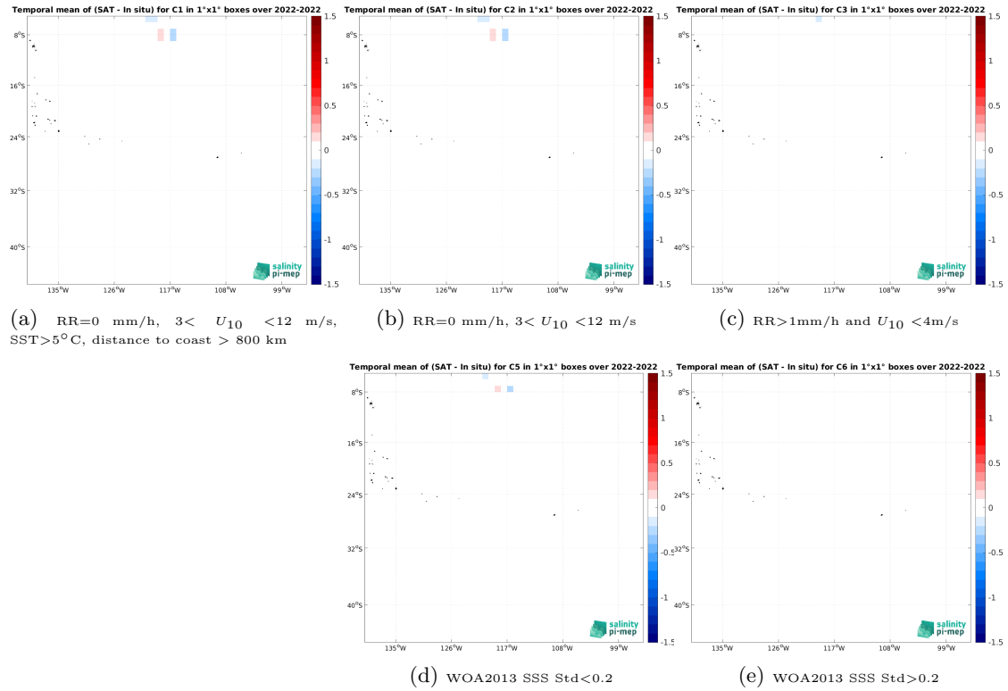
Figure 12: Temporal mean gridded over spatial boxes of size 1^\circ \times 1^\circ of \Delta SSS (SMAP SSS L4 OI v2 - Monthly (IPRC) - Saildrone) for 5 different subdatasets corresponding to: RR=0 mm/h, 3 < U_{10} < 12 m/s, SST > 5^\circ C , distance to coast > 800 km (a), RR=0 mm/h, 3 < U_{10} < 12 m/s (b), RR > 1 mm/h and U_{10} < 4 m/s (c), WOA2013 SSS Std < 0.2 (d), WOA2013 SSS Std > 0.2 (e).
