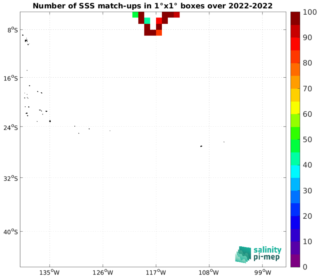
Figure 4: Number of SSS match-ups between Sairdrone SSS and the SMAP SSS L4 OI v2 - Monthly (IPRC) SSS product for the OTT zone Pi-MEP region over 1^\circ \times 1^\circ boxes and for the full satellite product period.
