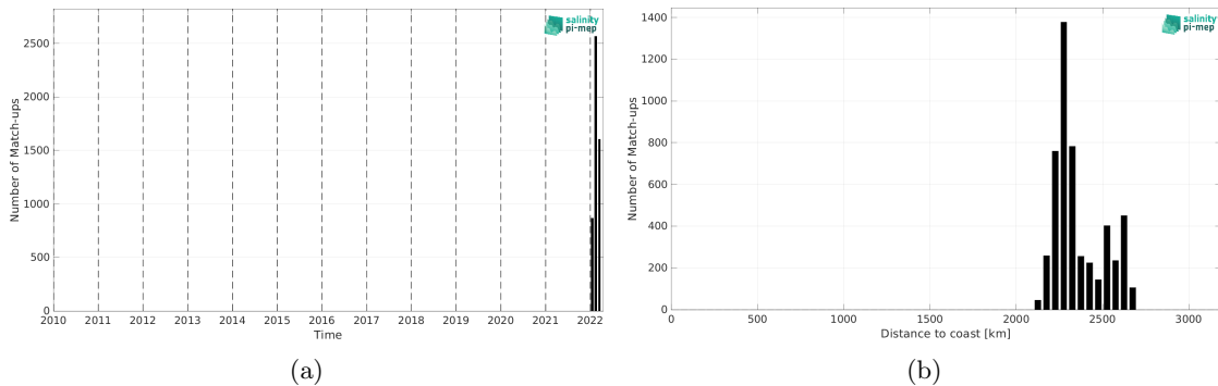
Figure 1: Number of match-ups between Saildrone and SMAP SSS L4 OI v2 - Monthly (IPRC) SSS as a function of time (a) and as function of the distance to coast (b) over the OTT zone Pi-MEP region and for the full satellite product period.
