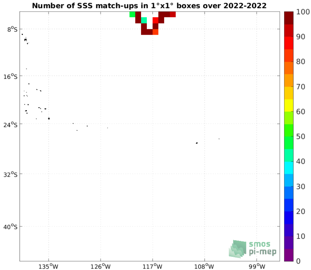
Figure 4: Number of SSS match-ups between Saildrone SSS and the SMAP SSS L4 OI v2 - Monthly (IPRC) SSS product for the OTT zone Pi-MEP region over 1^\circ \times 1^\circ boxes and for the full satellite product period.
