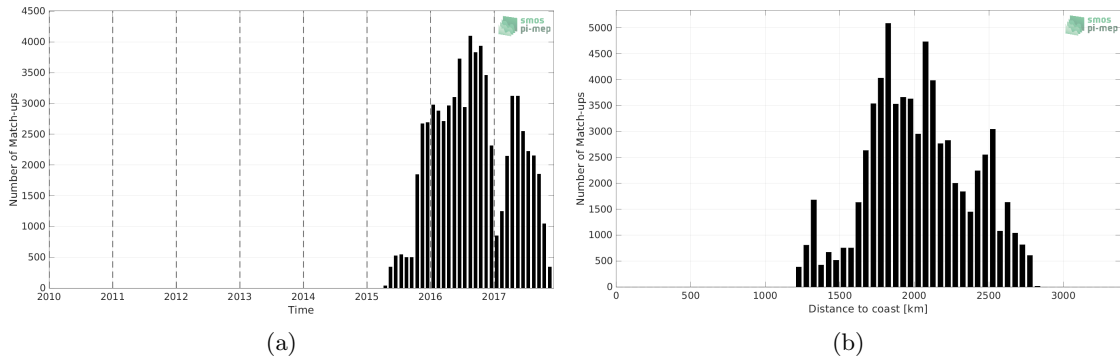
Figure 1: Number of match-ups between Surface drifters and SMAP SSS L4 OI v2 - Monthly (IPRC) SSS as a function of time (a) and as function of the distance to coast (b) over the OTT zone Pi-MEP region and for the full satellite product period.
