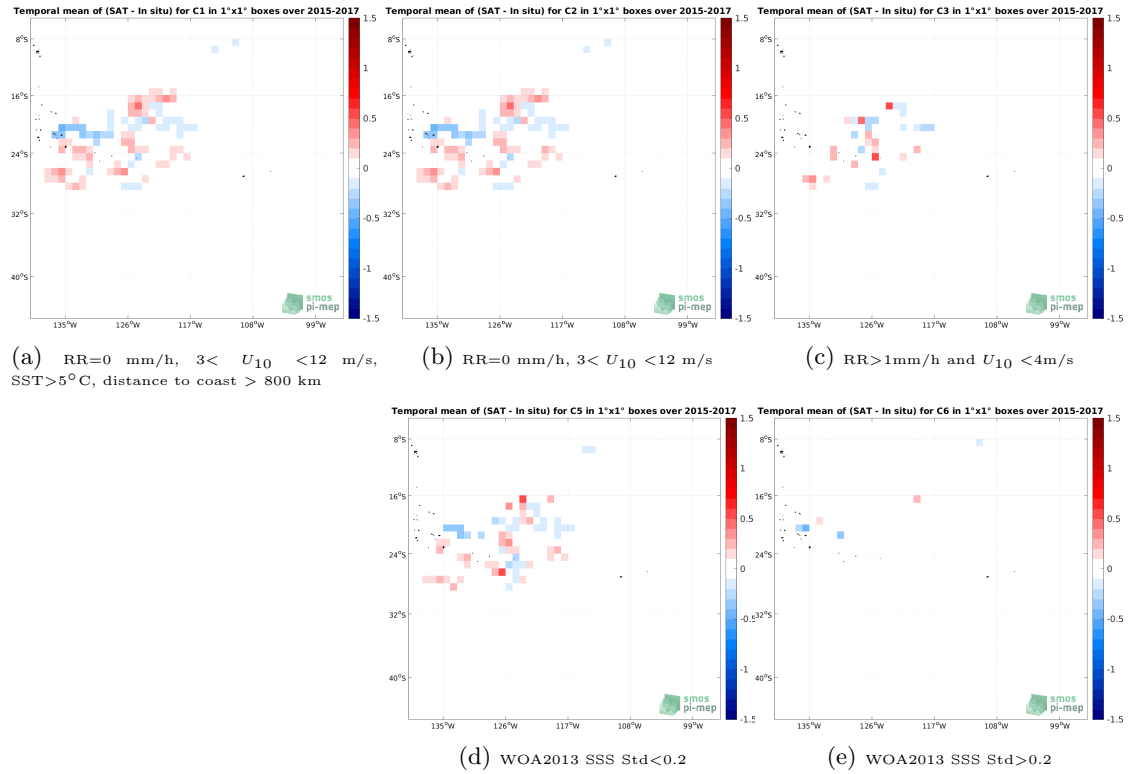
Figure 11: Temporal mean gridded over spatial boxes of size 1^\circ \times 1^\circ of \Delta SSS (SMAP SSS L4 OI v2 - Monthly (IPRC) - Surface drifters) for 5 different subdatasets corresponding to:RR=0 mm/h, 3 < U_{10} < 12 m/s, SST > 5^\circ\text{C} , distance to coast > 800 km (a), RR=0 mm/h, 3 < U_{10} < 12 m/s (b), RR > 1 mm/h and U_{10} < 4 m/s (c), WOA2013 SSS Std < 0.2 (d), WOA2013 SSS Std > 0.2 (e).
