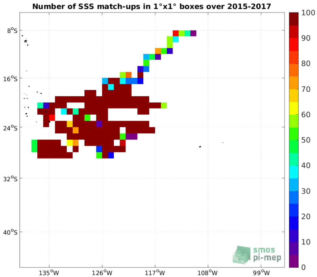
Figure 3: Number of SSS match-ups between Surface drifters SSS and the SMAP SSS L4 OI v2 - Monthly (IPRC) SSS product for the OTT zone Pi-MEP region over 1^\circ \times 1^\circ boxes and for the full satellite product period.
