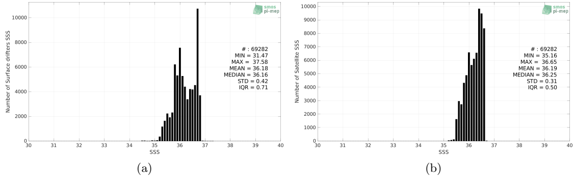
Figure 2: Histograms of SSS from Surface drifters (a) and SMAP SSS L4 OI v2 - Monthly (IPRC) (b) considering all match-up pairs per bins of 0.1 over the OTT zone Pi-MEP region and for the full satellite product period.
