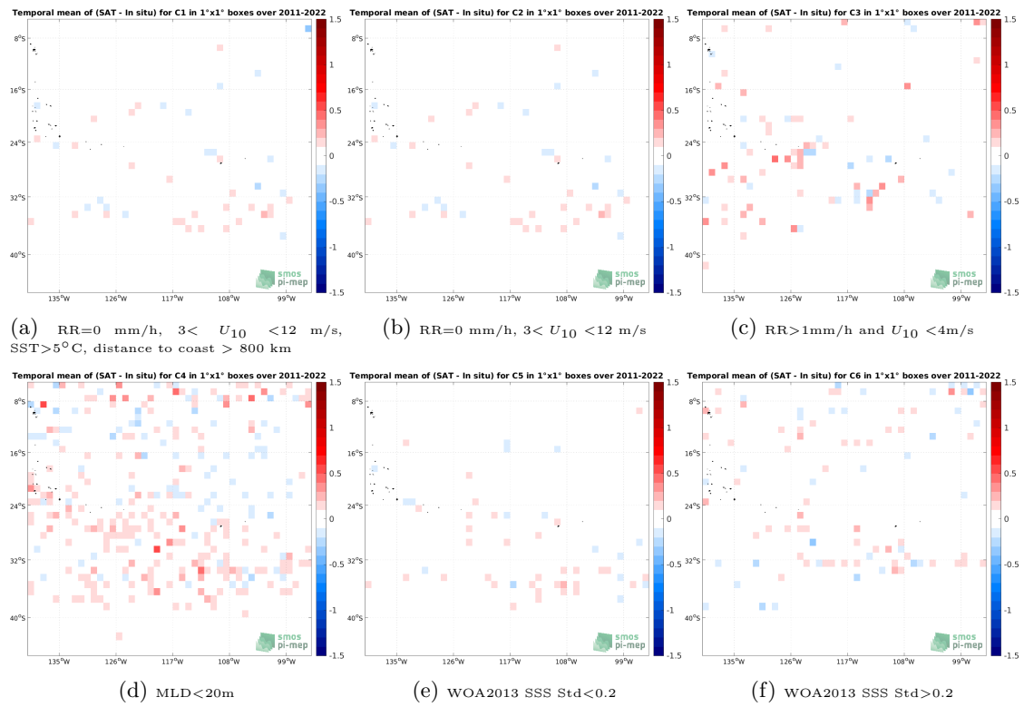
Figure 12: Temporal mean gridded over spatial boxes of size 1^\circ \times 1^\circ of \Delta SSS (SMAP SSS L4 OI v2 - Monthly (IPRC) - Argo) for 6 different subdatasets corresponding to:RR=0 mm/h, 3 < U_{10} < 12 m/s, SST >5^\circ\text{C} , distance to coast > 800 km (a), RR=0 mm/h, 3 < U_{10} < 12 m/s (b), RR >1 mm/h and U_{10} < 4 m/s (c),MLD <20 m (d),WOA2013 SSS Std <0.2 (e),WOA2013 SSS Std >0.2 (f).
