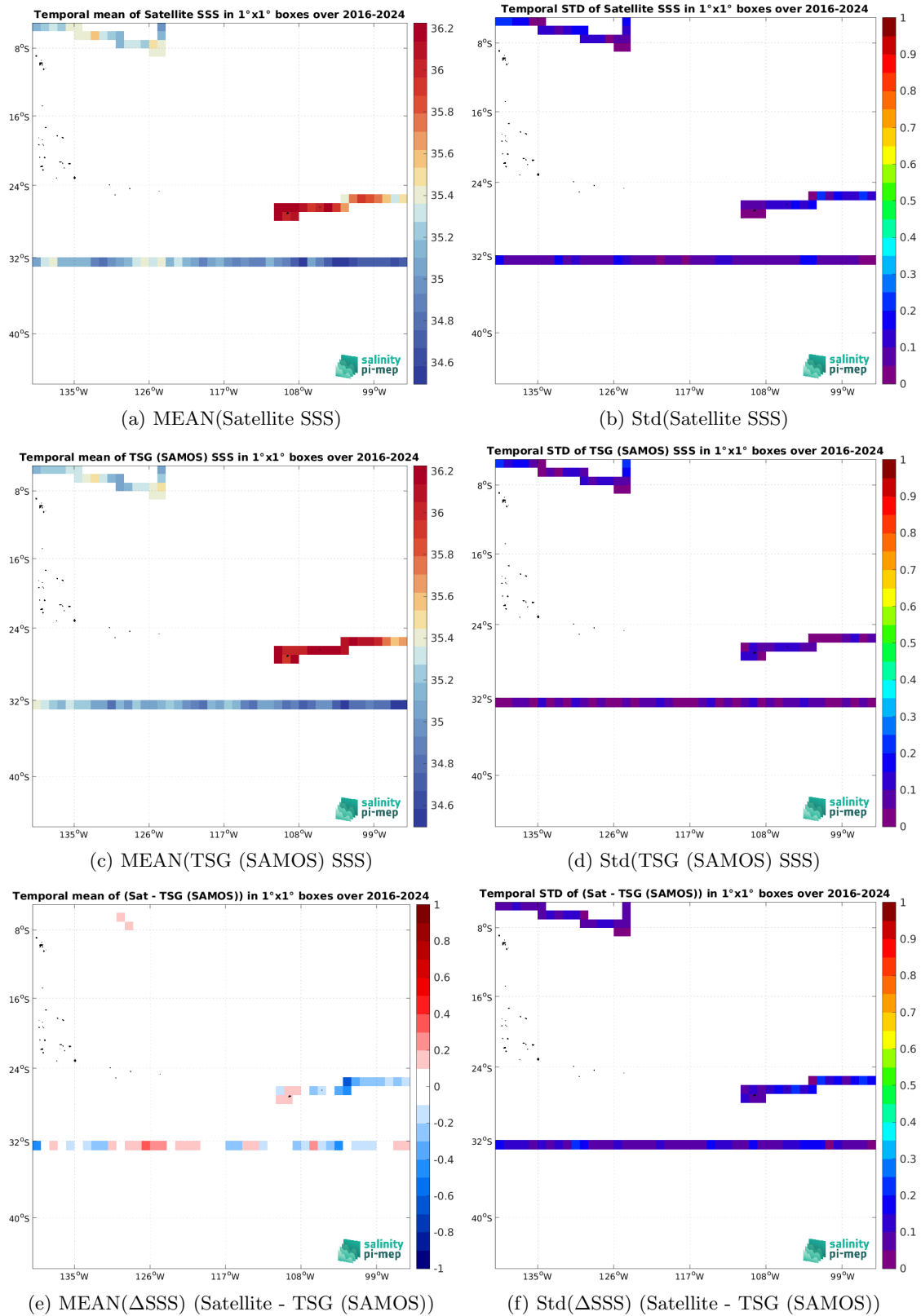
Figure 7: Temporal mean (left) and Std (right) of SSS from SMAP SSS L3 v6 - 8-Day running (RSS) (top), TSG (SAMOS) (middle), and of \Delta SSS (Satellite - TSG (SAMOS)). Only match-up pairs are used to generate these maps.
