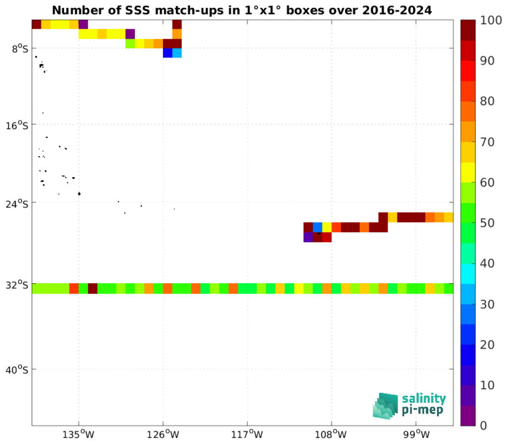
Figure 5: Number of SSS match-ups between TSG (SAMOS) SSS and the SMAP SSS L3 v6 - 8-Day running (RSS) SSS product for the OTT zone Pi-MEP region over 1°x1° boxes and for the full satellite product period.
