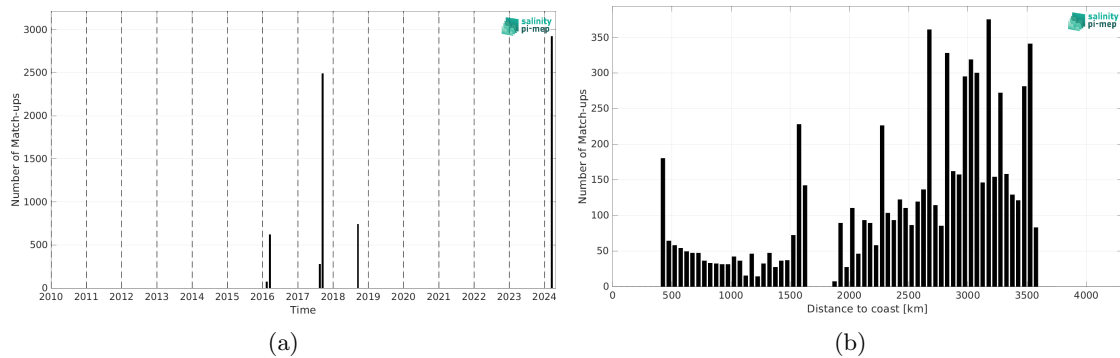
Figure 2: Number of match-ups between TSG (SAMOS) and SMAP SSS L3 v6 - 8-Day running (RSS) SSS as a function of time (a) and as function of the distance to coast (b) over the OTT zone Pi-MEP region and for the full satellite product period.
