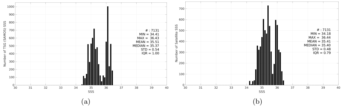
Figure 3: Histograms of SSS from TSG (SAMOS) (a) and SMAP SSS L3 v6 - 8-Day running (RSS) (b) considering all match-up pairs per bins of 0.1 over the OTT zone Pi-MEP region and for the full satellite product period.
