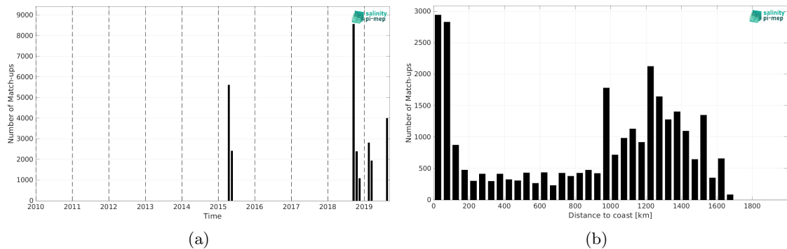
Figure 2: Number of match-ups between TSG (GOSUD-Research-vessel) and SMAP SSS L3 v6 - 8-Day running (RSS) SSS as a function of time (a) and as function of the distance to coast (b) over the OTT zone Pi-MEP region and for the full satellite product period.
