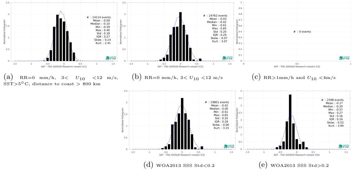
Figure 15: Normalized histogram of \Delta SSS (SMAP SSS L3 v6 - 8-Day running (RSS) - TSG (GOSUD-Research-vessel)) for 5 different subdatasets corresponding to: RR=0 mm/h, 3 < U_{10} < 12 m/s, SST>5°C, distance to coast > 800 km (a), RR=0 mm/h, 3 < U_{10} < 12 m/s (b), RR>1mm/h and U_{10} < 4 m/s (c), WOA2013 SSS Std<0.2 (d), WOA2013 SSS Std>0.2 (e).
