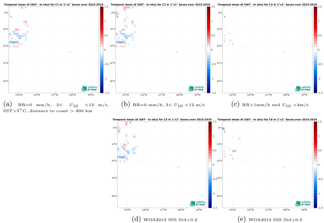
Figure 14: Temporal mean gridded over spatial boxes of size 1^\circ \times 1^\circ of \Delta SSS (SMAP SSS L3 v6 - 8-Day running (RSS) - TSG (GOSUD-Research-vessel)) for 5 different subdatasets corresponding to:RR=0 mm/h, 3 < U_{10} < 12 m/s, SST >5^\circ\text{C} , distance to coast > 800 km (a), RR=0 mm/h, 3 < U_{10} < 12 m/s (b), RR >1 mm/h and U_{10} < 4 m/s (c), WOA2013 SSS Std <0.2 (d), WOA2013 SSS Std >0.2 (e).
