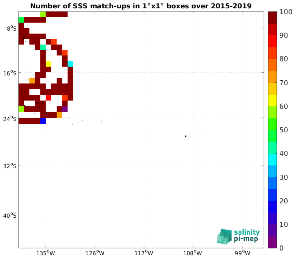
Figure 5: Number of SSS match-ups between TSG (GOSUD-Research-vessel) SSS and the SMAP SSS L3 v6 - 8-Day running (RSS) SSS product for the OTT zone Pi-MEP region over 1°x1° boxes and for the full satellite product period.
