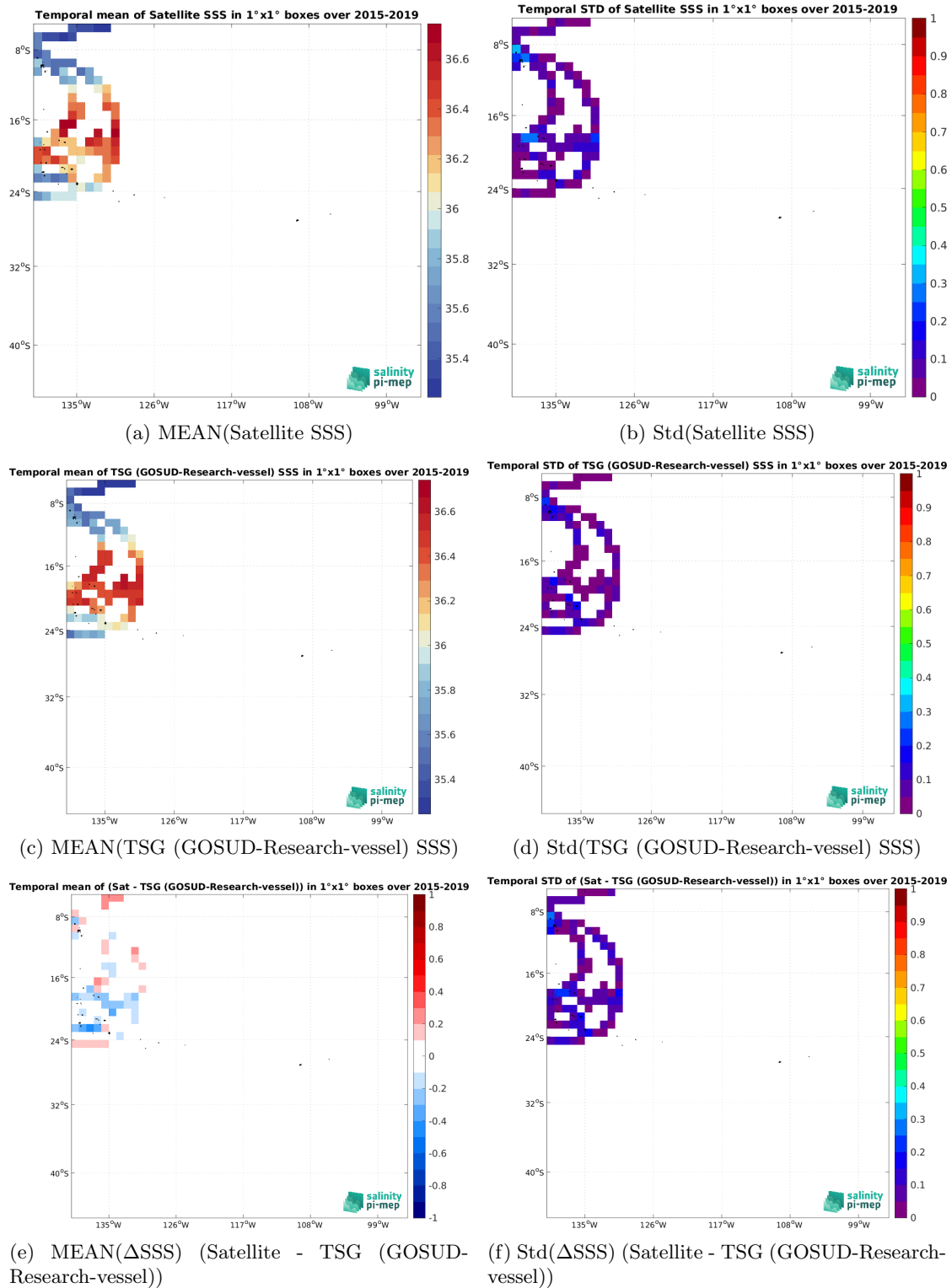
Figure 7: Temporal mean (left) and Std (right) of SSS from SMAP SSS L3 v6 - 8-Day running (RSS) (top), TSG (GOSUD-Research-vessel) (middle), and of \Delta SSS (Satellite - TSG (GOSUD-Research-vessel)). Only match-up pairs are used to generate these maps.
