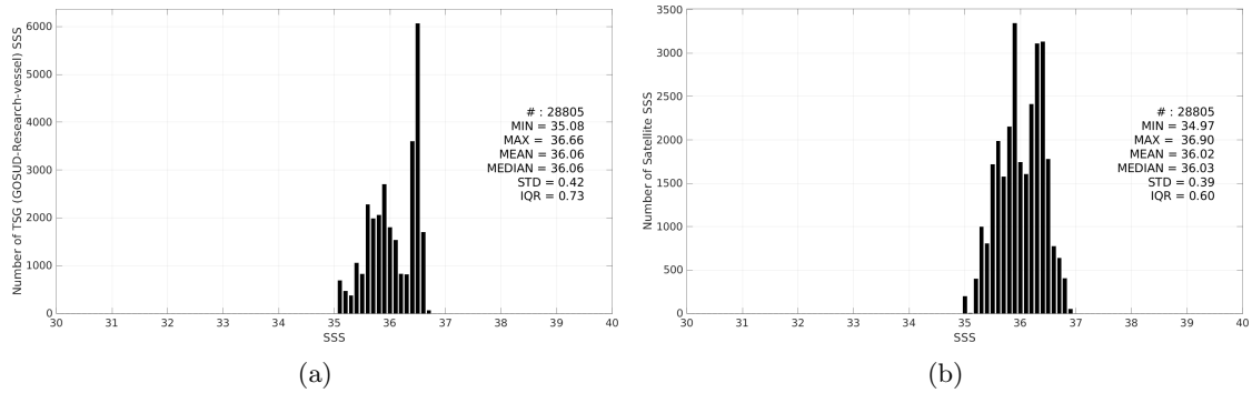
Figure 3: Histograms of SSS from TSG (GOSUD-Research-vessel) (a) and SMAP SSS L3 v6 - 8-Day running (RSS) (b) considering all match-up pairs per bins of 0.1 over the OTT zone Pi-MEP region and for the full satellite product period.
