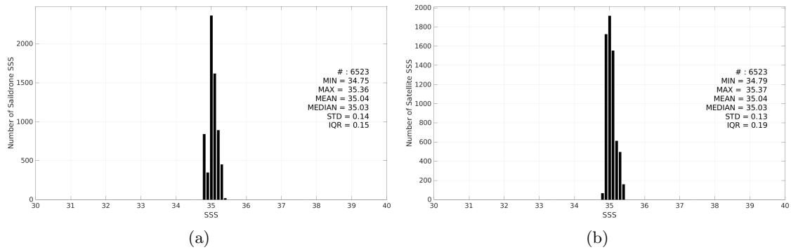
Figure 3: Histograms of SSS from Saildrone (a) and SMAP SSS L3 v6 - 8-Day running (RSS) (b) considering all match-up pairs per bins of 0.1 over the OTT zone Pi-MEP region and for the full satellite product period.
