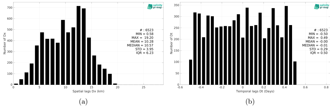
Figure 6: Histograms of the spatial (a) and temporal (b) lags between the location/time of the Sairdron measurement and the date of the corresponding SMAP SSS L3 v6 - 8-Day running (RSS) SSS pixel.
