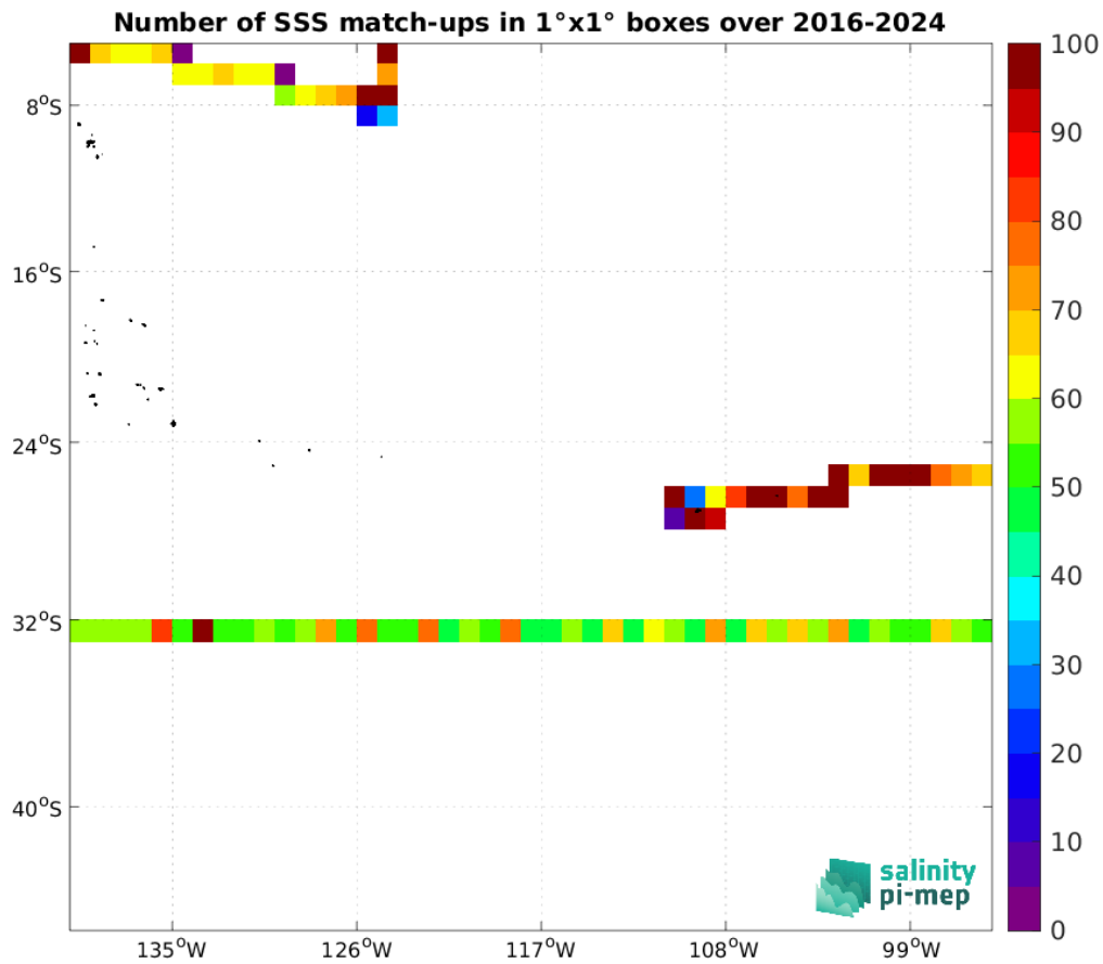
Figure 5: Number of SSS match-ups between TSG (SAMOS) SSS and the SMAP SSS L3 v6 - Monthly (RSS) SSS product for the OTT zone Pi-MEP region over 1°x1° boxes and for the full satellite product period.
