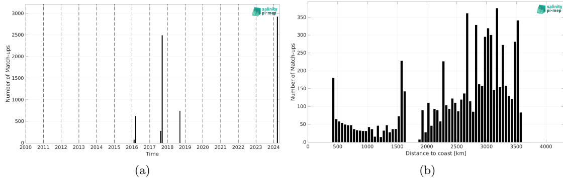
Figure 2: Number of match-ups between TSG (SAMOS) and SMAP SSS L3 v6 - Monthly (RSS) SSS as a function of time (a) and as function of the distance to coast (b) over the OTT zone Pi-MEP region and for the full satellite product period.
