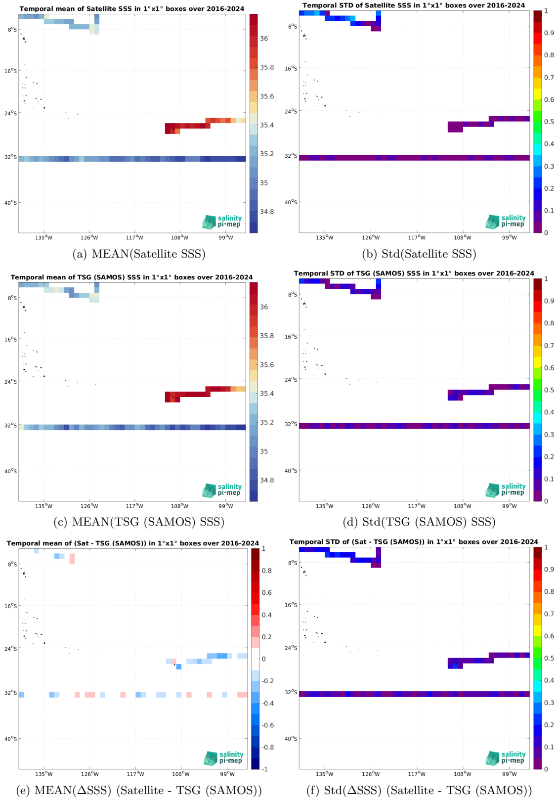
Figure 7: Temporal mean (left) and Std (right) of SSS from SMAP SSS L3 v6 - Monthly (RSS) (top), TSG (SAMOS) (middle), and of \Delta SSS (Satellite - TSG (SAMOS)). Only match-up pairs are used to generate these maps.
