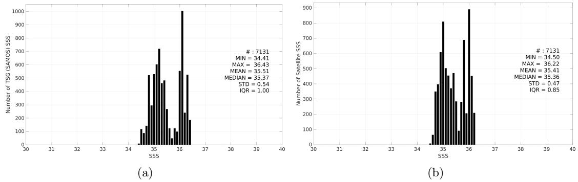
Figure 3: Histograms of SSS from TSG (SAMOS) (a) and SMAP SSS L3 v6 - Monthly (RSS) (b) considering all match-up pairs per bins of 0.1 over the OTT zone Pi-MEP region and for the full satellite product period.
