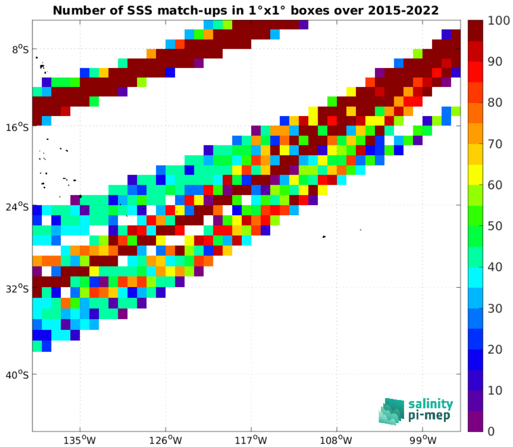
Figure 5: Number of SSS match-ups between TSG (LEGOS-DM) SSS and the SMAP SSS L3 v6 - Monthly (RSS) SSS product for the OTT zone Pi-MEP region over 1^\circ \times 1^\circ boxes and for the full satellite product period.
