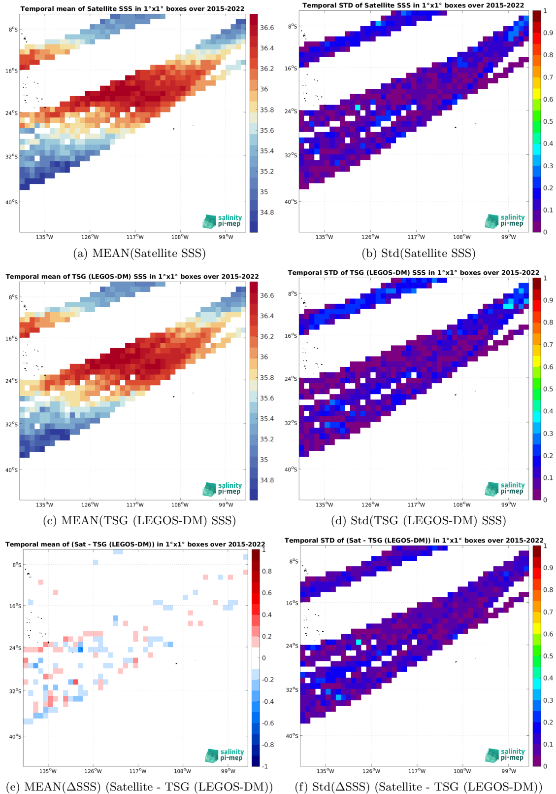
Figure 7: Temporal mean (left) and Std (right) of SSS from SMAP SSS L3 v6 - Monthly (RSS) (top), TSG (LEGOS-DM) (middle), and of \Delta SSS (Satellite - TSG (LEGOS-DM)). Only match-up pairs are used to generate these maps.
