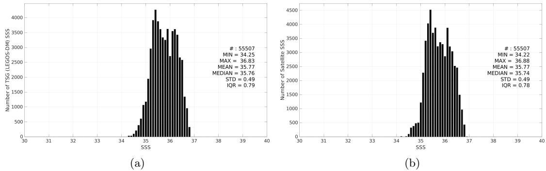
Figure 3: Histograms of SSS from TSG (LEGOS-DM) (a) and SMAP SSS L3 v6 - Monthly (RSS) (b) considering all match-up pairs per bins of 0.1 over the OTT zone Pi-MEP region and for the full satellite product period.
