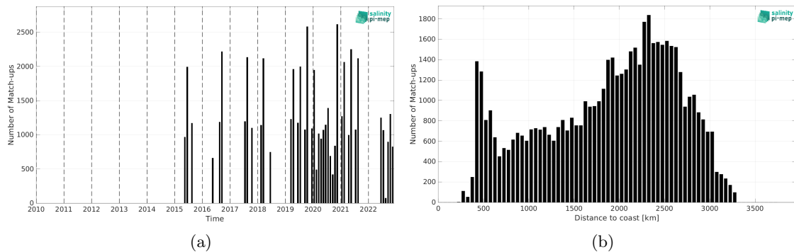
Figure 2: Number of match-ups between TSG (LEGOS-DM) and SMAP SSS L3 v6 - Monthly (RSS) SSS as a function of time (a) and as function of the distance to coast (b) over the OTT zone Pi-MEP region and for the full satellite product period.
