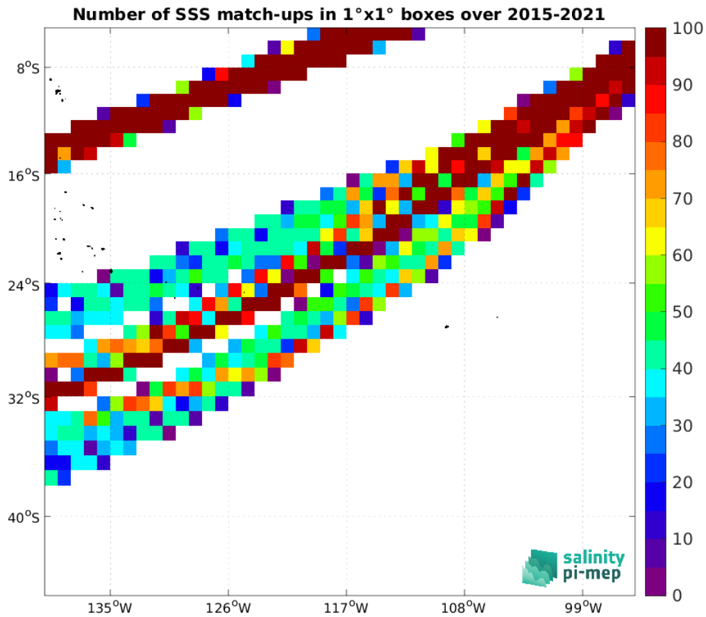
Figure 5: Number of SSS match-ups between TSG (LEGOS-DM) SSS and the SMAP SSS L3 v6 - Monthly (RSS) SSS product for the OTT zone Pi-MEP region over 1°x1° boxes and for the full satellite product period.
