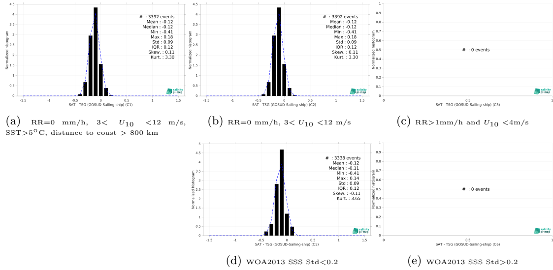
Figure 15: Normalized histogram of \Delta SSS (SMAP SSS L3 v6 - Monthly (RSS) - TSG (GOSUD-Sailing-ship)) for 5 different subdatasets corresponding to: RR=0 mm/h, 3 < U_{10} < 12 m/s, SST >5^{\circ}\text{C} , distance to coast > 800 km (a), RR=0 mm/h, 3 < U_{10} < 12 m/s (b), RR >1 mm/h and U_{10} < 4 m/s (c), WOA2013 SSS Std <0.2 (d), WOA2013 SSS Std >0.2 (e).
