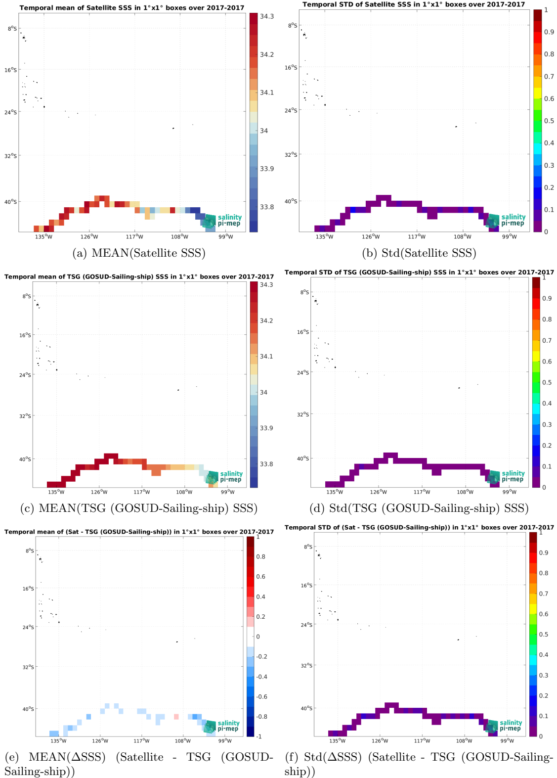
Figure 7: Temporal mean (left) and Std (right) of SSS from SMAP SSS L3 v6 - Monthly (RSS) (top), TSG (GOSUD-Sailing-ship) (middle), and of \Delta SSS (Satellite - TSG (GOSUD-Sailing-ship)). Only match-up pairs are used to generate these maps.
