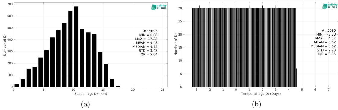
Figure 6: Histograms of the spatial (a) and temporal (b) lags between the location/time of the TSG (GOSUD-Sailing-ship) measurement and the date of the corresponding SMAP SSS L3 v6 - Monthly (RSS) SSS pixel.
