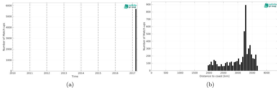
Figure 2: Number of match-ups between TSG (GOSUD-Sailing-ship) and SMAP SSS L3 v6 - Monthly (RSS) SSS as a function of time (a) and as function of the distance to coast (b) over the OTT zone Pi-MEP region and for the full satellite product period.
