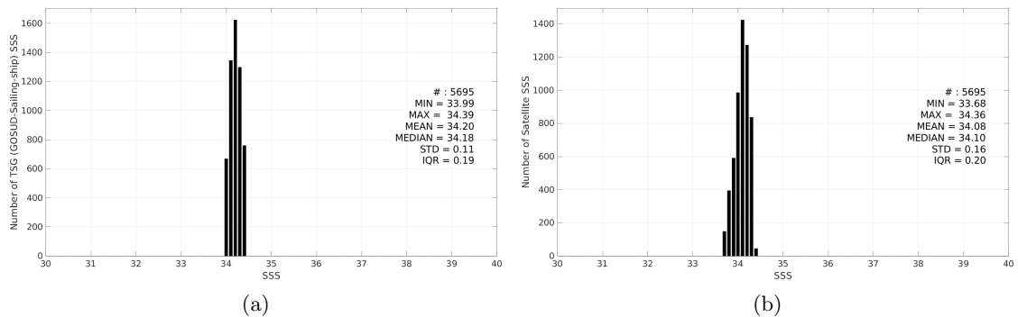
Figure 3: Histograms of SSS from TSG (GOSUD-Sailing-ship) (a) and SMAP SSS L3 v6 - Monthly (RSS) (b) considering all match-up pairs per bins of 0.1 over the OTT zone Pi-MEP region and for the full satellite product period.
