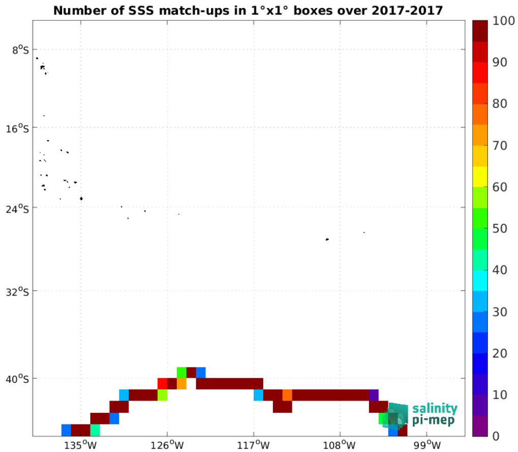
Figure 5: Number of SSS match-ups between TSG (GOSUD-Sailing-ship) SSS and the SMAP SSS L3 v6 - Monthly (RSS) SSS product for the OTT zone Pi-MEP region over 1°x1° boxes and for the full satellite product period.
