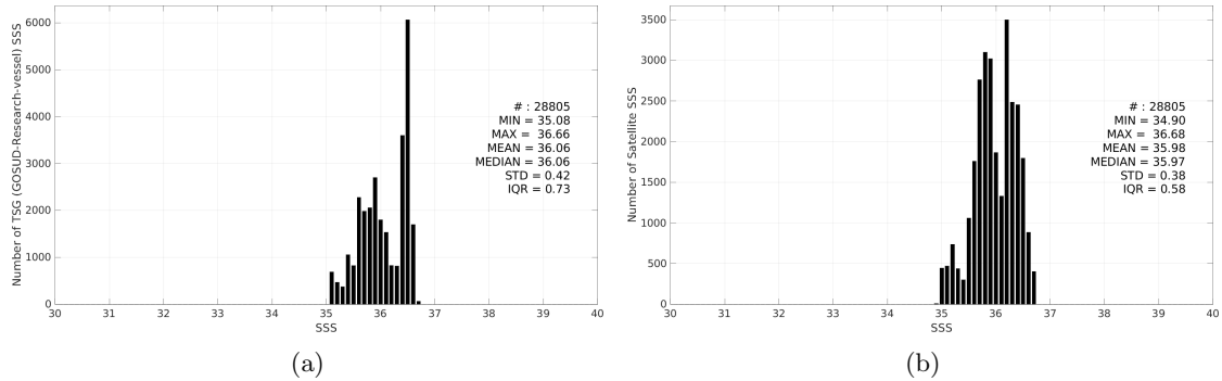
Figure 3: Histograms of SSS from TSG (GOSUD-Research-vessel) (a) and SMAP SSS L3 v6 - Monthly (RSS) (b) considering all match-up pairs per bins of 0.1 over the OTT zone Pi-MEP region and for the full satellite product period.
