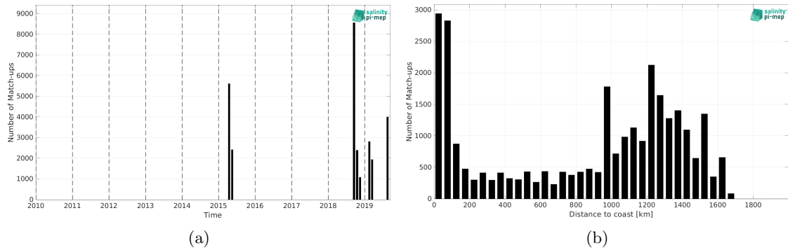
Figure 2: Number of match-ups between TSG (GOSUD-Research-vessel) and SMAP SSS L3 v6 - Monthly (RSS) SSS as a function of time (a) and as function of the distance to coast (b) over the OTT zone Pi-MEP region and for the full satellite product period.
