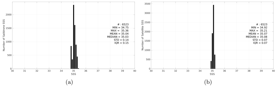
Figure 3: Histograms of SSS from Saildrone (a) and SMAP SSS L3 v6 - Monthly (RSS) (b) considering all match-up pairs per bins of 0.1 over the OTT zone Pi-MEP region and for the full satellite product period.
