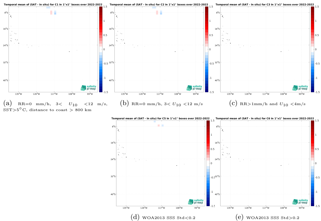
Figure 14: Temporal mean gridded over spatial boxes of size 1^\circ \times 1^\circ of \Delta SSS (SMAP SSS L3 v6 - Monthly (RSS) - Saildrone) for 5 different subdatasets corresponding to:RR=0 mm/h, 3 < U_{10} < 12 m/s, SST >5^\circ\text{C} , distance to coast > 800 km (a), RR=0 mm/h, 3 < U_{10} < 12 m/s (b), RR >1 mm/h and U_{10} < 4 m/s (c), WOA2013 SSS Std <0.2 (d), WOA2013 SSS Std >0.2 (e).
