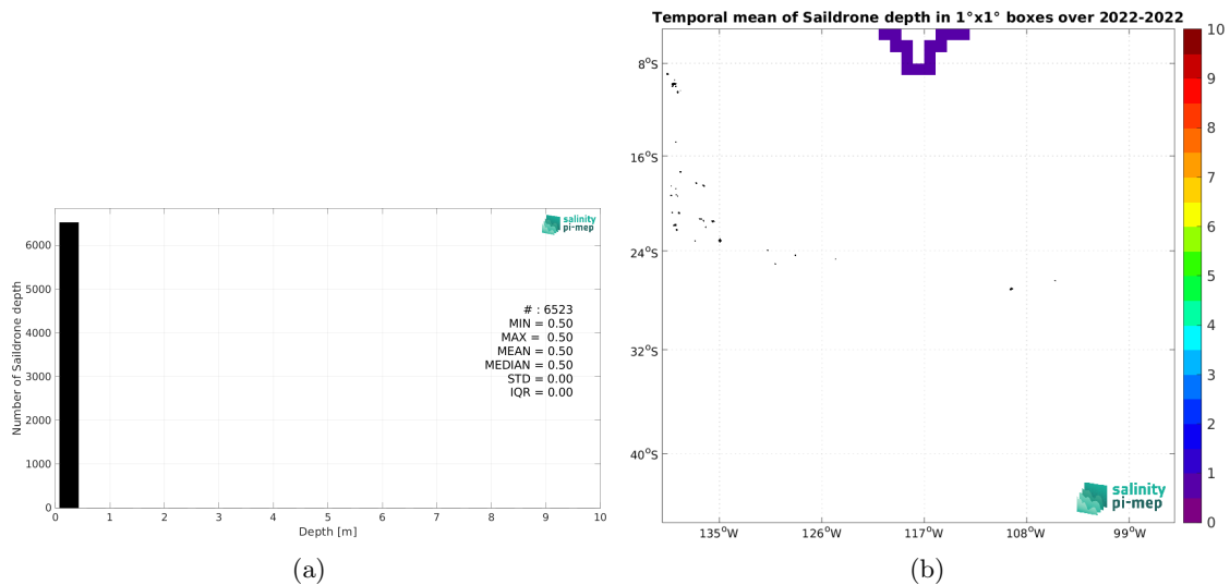
Figure 4: Histograms of the depth of the upper level SSS measurements from Saïdrone in the Match-up DataBase for the OTT zone Pi-MEP region (a) and temporal mean spatial distribution of pressure of the in situ SSS data over 1^\circ \times 1^\circ boxes and for the full satellite product period (b).
