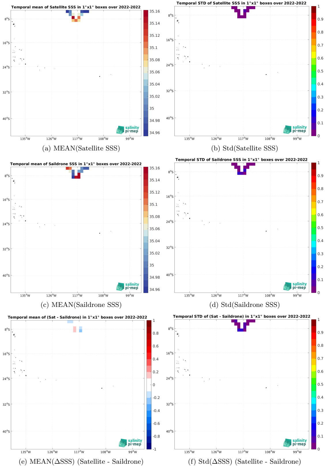
Figure 7: Temporal mean (left) and Std (right) of SSS from SMAP SSS L3 v6 - Monthly (RSS) (top), Saildrone (middle), and of \Delta SSS (Satellite - Saildrone). Only match-up pairs are used to generate these maps.
