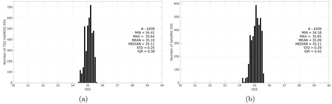
Figure 3: Histograms of SSS from TSG (SAMOS) (a) and SMAP SSS L3 v5.3 - 8-Day running (RSS) (b) considering all match-up pairs per bins of 0.1 over the OTT zone Pi-MEP region and for the full satellite product period.
