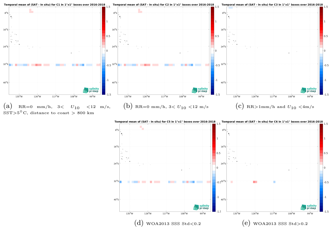
Figure 14: Temporal mean gridded over spatial boxes of size 1^\circ \times 1^\circ of \Delta SSS (SMAP SSS L3 v5.3 - 8-Day running (RSS) - TSG (SAMOS)) for 5 different subdatasets corresponding to: RR=0 mm/h, 3 < U_{10} < 12 m/s, SST > 5^\circ C , distance to coast > 800 km (a), RR=0 mm/h, 3 < U_{10} < 12 m/s (b), RR > 1 mm/h and U_{10} < 4 m/s (c), WOA2013 SSS Std < 0.2 (d), WOA2013 SSS Std > 0.2 (e).
