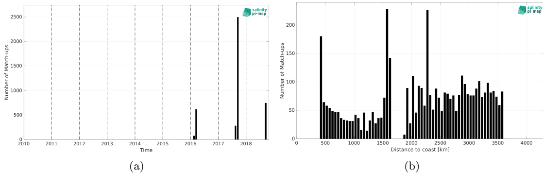
Figure 2: Number of match-ups between TSG (SAMOS) and SMAP SSS L3 v5.3 - 8-Day running (RSS) SSS as a function of time (a) and as function of the distance to coast (b) over the OTT zone Pi-MEP region and for the full satellite product period.
