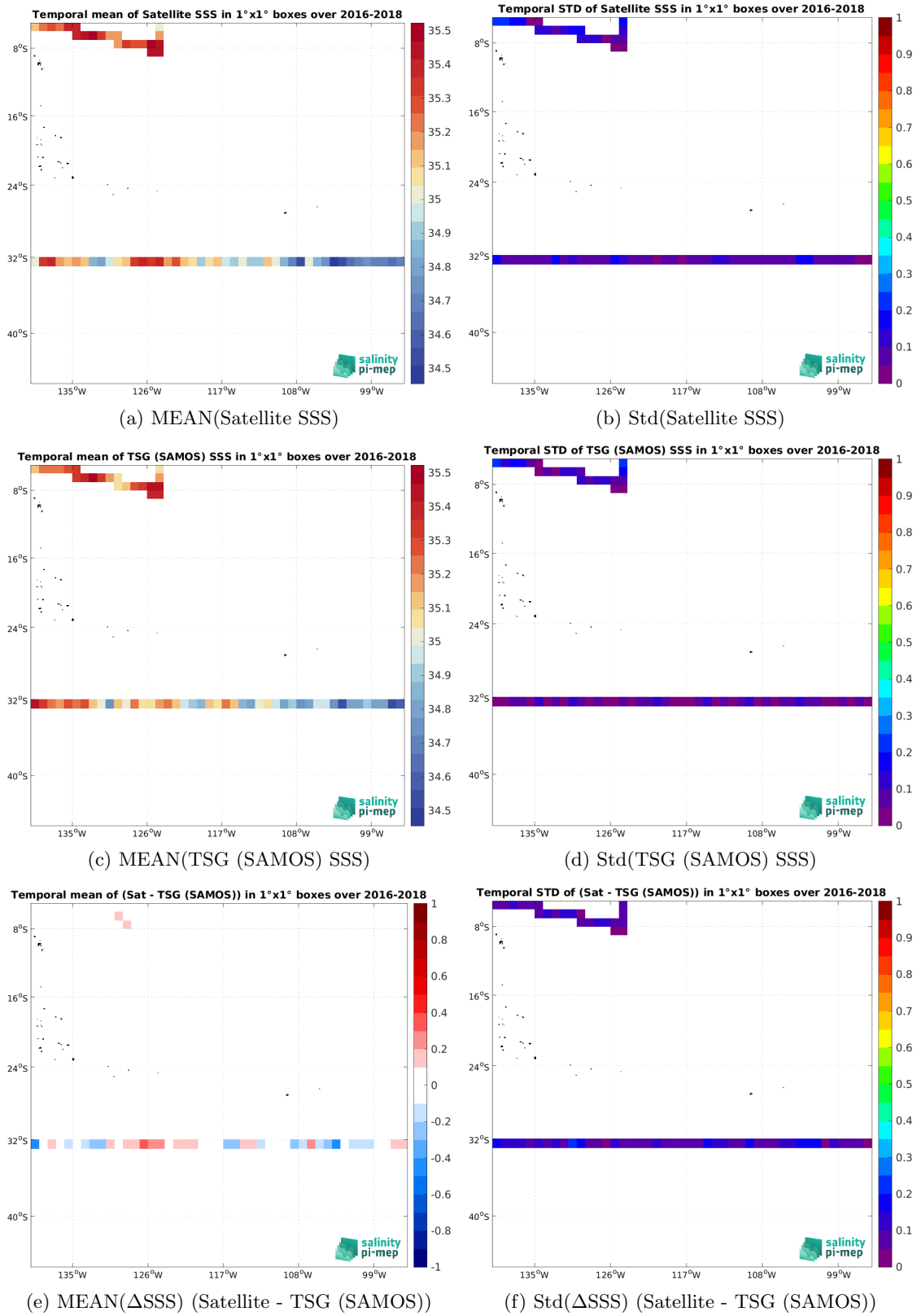
Figure 7: Temporal mean (left) and Std (right) of SSS from SMAP SSS L3 v5.3 - 8-Day running (RSS) (top), TSG (SAMOS) (middle), and of \Delta SSS (Satellite - TSG (SAMOS)). Only match-up pairs are used to generate these maps.
