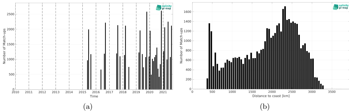
Figure 2: Number of match-ups between TSG (LEGOS-DM) and SMAP SSS L3 v5.3 - 8-Day running (RSS) SSS as a function of time (a) and as function of the distance to coast (b) over the OTT zone Pi-MEP region and for the full satellite product period.
