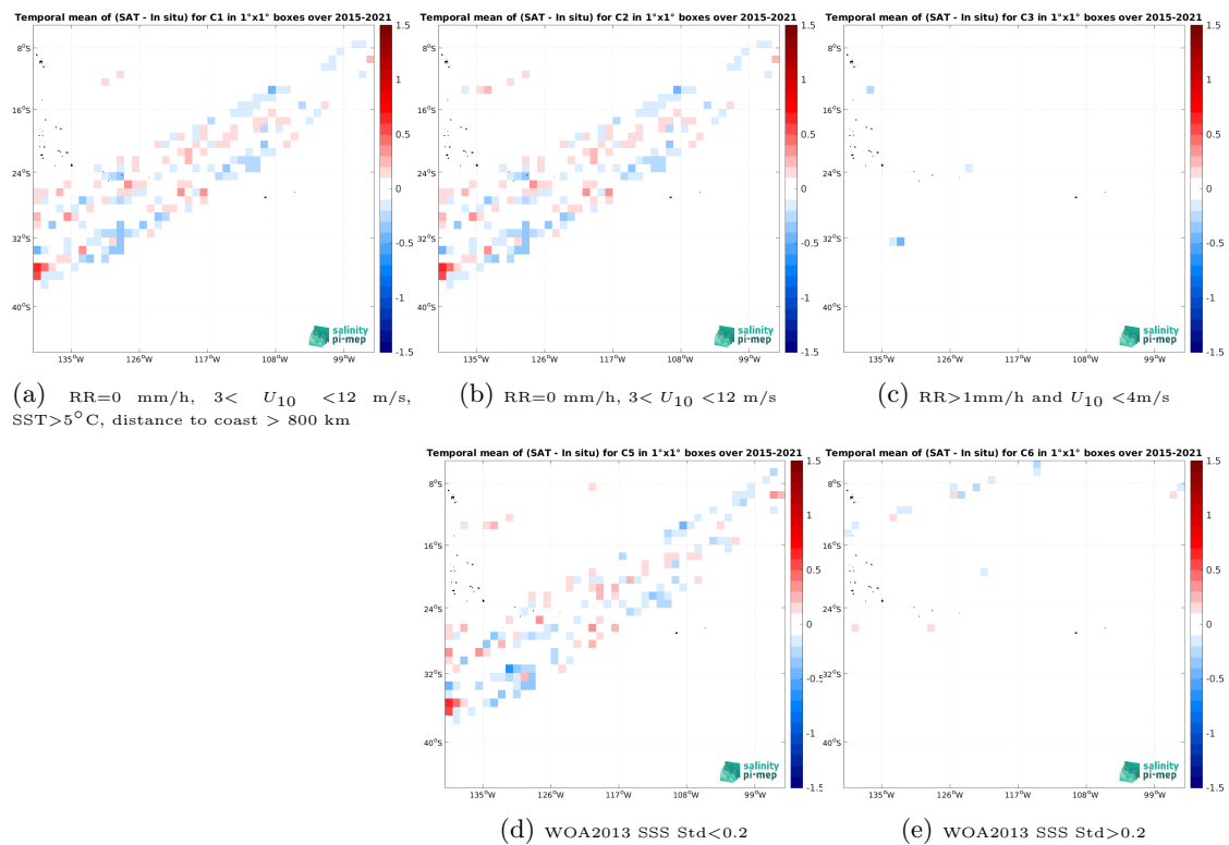
Figure 14: Temporal mean gridded over spatial boxes of size 1^\circ \times 1^\circ of \Delta\text{SSS} (SMAP SSS L3 v5.3 - 8-Day running (RSS) - TSG (LEGOS-DM)) for 5 different subdatasets corresponding to:RR=0 mm/h, 3 < U_{10} < 12 m/s, SST >5^\circ\text{C} , distance to coast > 800 km (a), RR=0 mm/h, 3 < U_{10} < 12 m/s (b), RR >1 mm/h and U_{10} < 4 m/s (c), WOA2013 SSS Std <0.2 (d), WOA2013 SSS Std >0.2 (e).
