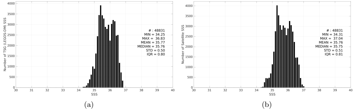
Figure 3: Histograms of SSS from TSG (LEGOS-DM) (a) and SMAP SSS L3 v5.3 - 8-Day running (RSS) (b) considering all match-up pairs per bins of 0.1 over the OTT zone Pi-MEP region and for the full satellite product period.
