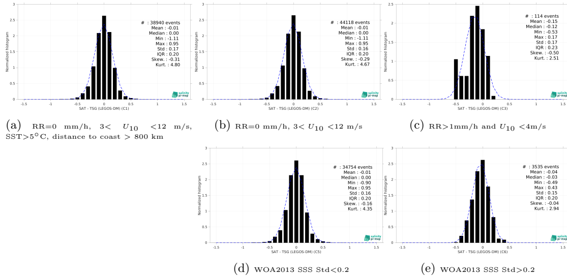
Figure 15: Normalized histogram of \Delta\text{SSS} (SMAP SSS L3 v5.3 - 8-Day running (RSS) - TSG (LEGOS-DM)) for 5 different subdatasets corresponding to: RR=0 mm/h, 3 < U_{10} < 12 m/s, SST>5°C, distance to coast > 800 km (a), RR=0 mm/h, 3 < U_{10} < 12 m/s (b), RR>1mm/h and U_{10} < 4 m/s (c), WOA2013 SSS Std<0.2 (d), WOA2013 SSS Std>0.2 (e).
