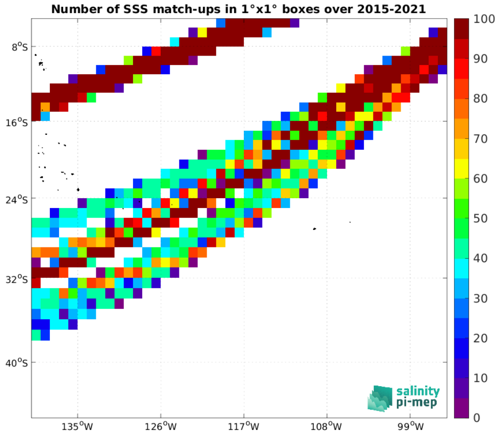
Figure 5: Number of SSS match-ups between TSG (LEGOS-DM) SSS and the SMAP SSS L3 v5.3 - 8-Day running (RSS) SSS product for the OTT zone Pi-MEP region over 1^\circ \times 1^\circ boxes and for the full satellite product period.
