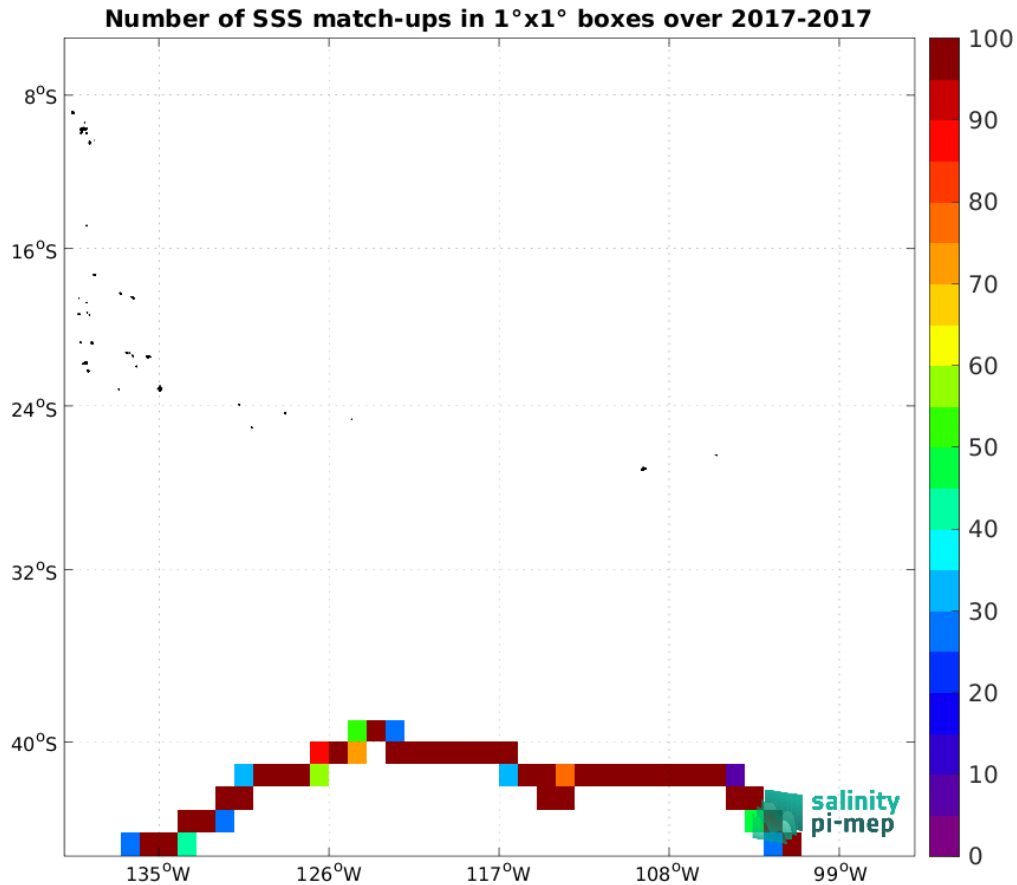
Figure 5: Number of SSS match-ups between TSG (GOSUD-Sailing-ship) SSS and the SMAP SSS L3 v5.3 - 8-Day running (RSS) SSS product for the OTT zone Pi-MEP region over 1^\circ \times 1^\circ boxes and for the full satellite product period.
