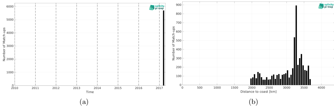
Figure 2: Number of match-ups between TSG (GOSUD-Sailing-ship) and SMAP SSS L3 v5.3 - 8-Day running (RSS) SSS as a function of time (a) and as function of the distance to coast (b) over the OTT zone Pi-MEP region and for the full satellite product period.
