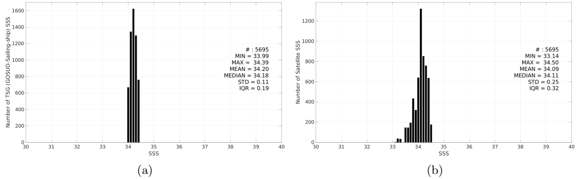
Figure 3: Histograms of SSS from TSG (GOSUD-Sailing-ship) (a) and SMAP SSS L3 v5.3 - 8-Day running (RSS) (b) considering all match-up pairs per bins of 0.1 over the OTT zone Pi-MEP region and for the full satellite product period.
