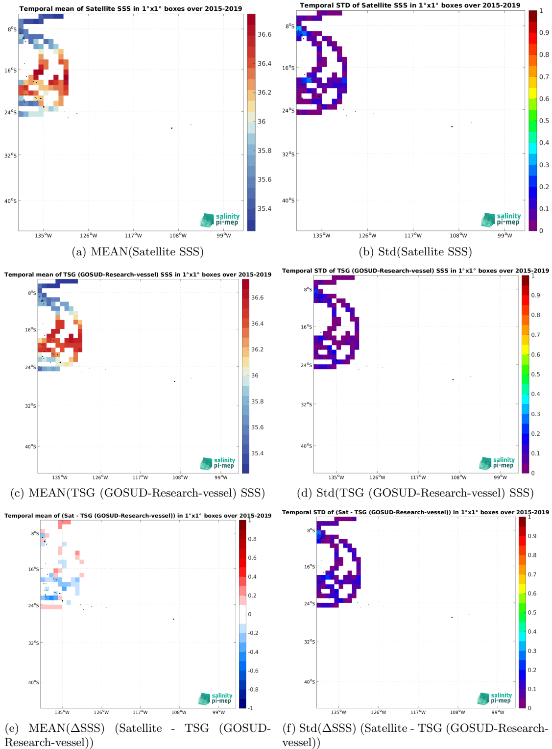
Figure 7: Temporal mean (left) and Std (right) of SSS from SMAP SSS L3 v5.3 - 8-Day running (RSS) (top), TSG (GOSUD-Research-vessel) (middle), and of \Delta SSS (Satellite - TSG (GOSUD-Research-vessel)). Only match-up pairs are used to generate these maps.
