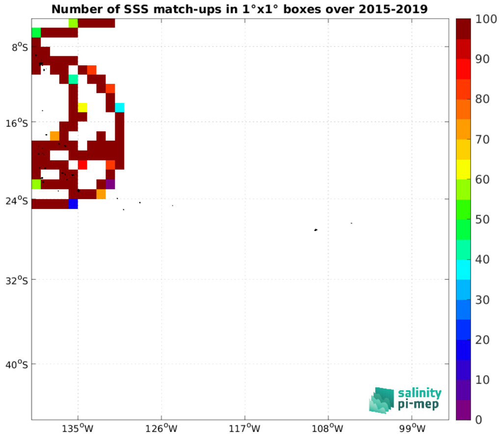
Figure 5: Number of SSS match-ups between TSG (GOSUD-Research-vessel) SSS and the SMAP SSS L3 v5.3 - 8-Day running (RSS) SSS product for the OTT zone Pi-MEP region over 1^\circ \times 1^\circ boxes and for the full satellite product period.
