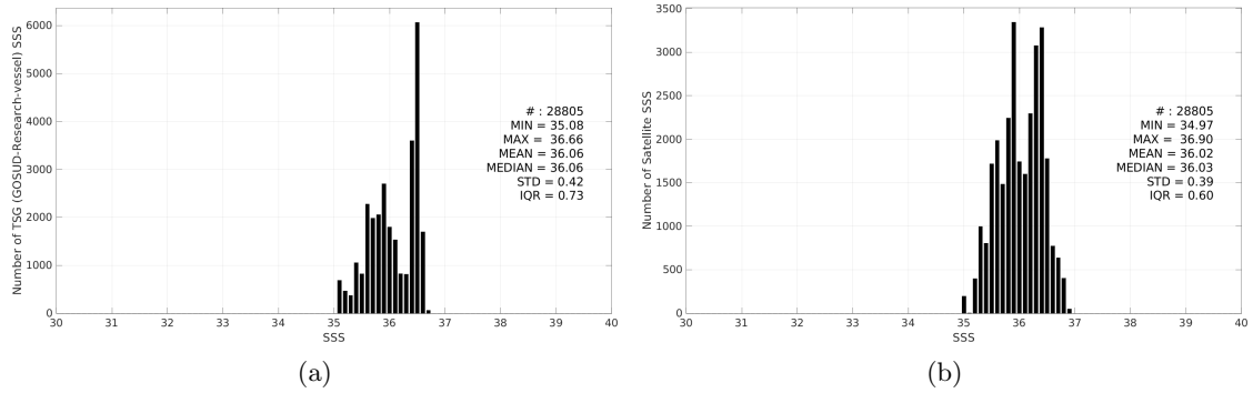
Figure 3: Histograms of SSS from TSG (GOSUD-Research-vessel) (a) and SMAP SSS L3 v5.3 - 8-Day running (RSS) (b) considering all match-up pairs per bins of 0.1 over the OTT zone Pi-MEP region and for the full satellite product period.
