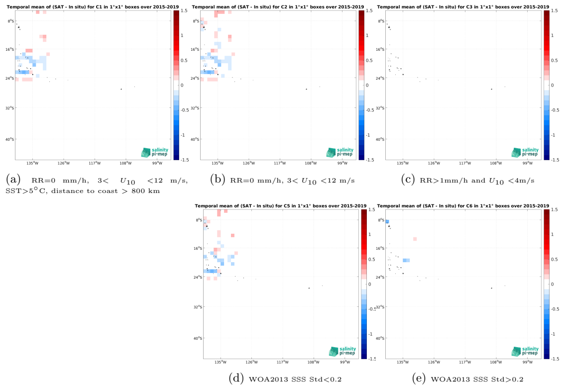
Figure 14: Temporal mean gridded over spatial boxes of size 1^\circ \times 1^\circ of \Delta SSS (SMAP SSS L3 v5.3 - 8-Day running (RSS) - TSG (GOSUD-Research-vessel)) for 5 different subdatasets corresponding to:RR=0 mm/h, 3 < U_{10} < 12 m/s, SST >5^\circ\text{C} , distance to coast > 800 km (a), RR=0 mm/h, 3 < U_{10} < 12 m/s (b), RR >1 mm/h and U_{10} < 4 m/s (c), WOA2013 SSS Std <0.2 (d), WOA2013 SSS Std >0.2 (e).
