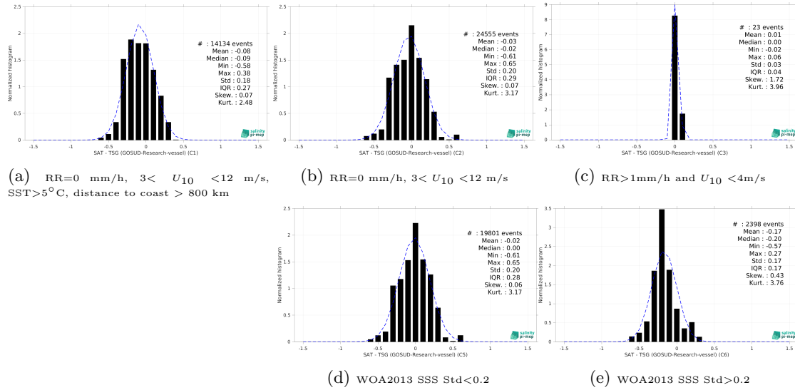
Figure 15: Normalized histogram of \Delta\text{SSS} (SMAP SSS L3 v5.3 - 8-Day running (RSS) - TSG (GOSUD-Research-vessel)) for 5 different subdatasets corresponding to: RR=0 mm/h, 3 < U_{10} < 12 m/s, SST > 5^\circ\text{C} , distance to coast > 800 km (a), RR=0 mm/h, 3 < U_{10} < 12 m/s (b), RR > 1\text{mm/h} and U_{10} < 4\text{m/s} (c), WOA2013 SSS Std < 0.2 (d), WOA2013 SSS Std > 0.2 (e).
