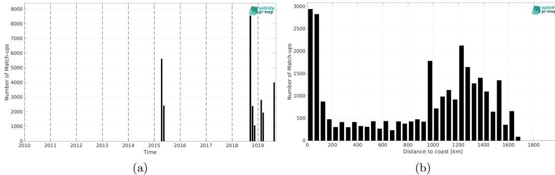
Figure 2: Number of match-ups between TSG (GOSUD-Research-vessel) and SMAP SSS L3 v5.3 - 8-Day running (RSS) SSS as a function of time (a) and as function of the distance to coast (b) over the OTT zone Pi-MEP region and for the full satellite product period.
