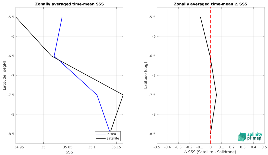
Figure 9: Left panel: Zonal mean SSS from SMAP SSS L3 v5.3 - 8-Day running (RSS) satellite product (black) and from Saildrone (blue). Right panel: Zonal mean of \Delta SSS (Satellite - Saildrone) for all the collected Pi-MEP match-up pairs estimated over the full satellite product period.
