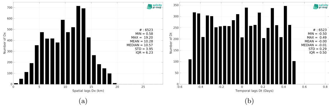
Figure 6: Histograms of the spatial (a) and temporal (b) lags between the location/time of the Saildrone measurement and the date of the corresponding SMAP SSS L3 v5.3 - 8-Day running (RSS) SSS pixel.
