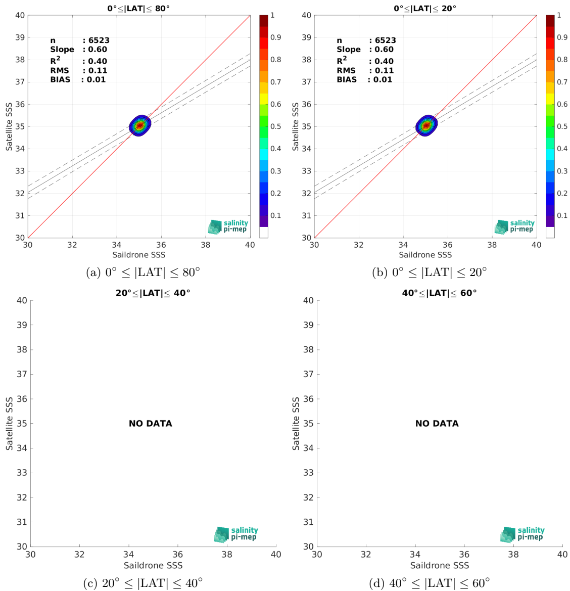
Figure 10: Contour maps of the concentration of SMAP SSS L3 v5.3 - 8-Day running (RSS) SSS (y-axis) versus Saildrone SSS (x-axis) at match-up pairs for different latitude bands. For each plot, the red line shows x=y . The black thin and dashed lines indicate a linear fit through the data cloud and the \pm 95\% confidence levels, respectively. The number match-up pairs n , the slope and R^2 coefficient of the linear fit, the root mean square (RMS) and the mean bias between satellite and in situ data are indicated for each latitude band in each plots.
