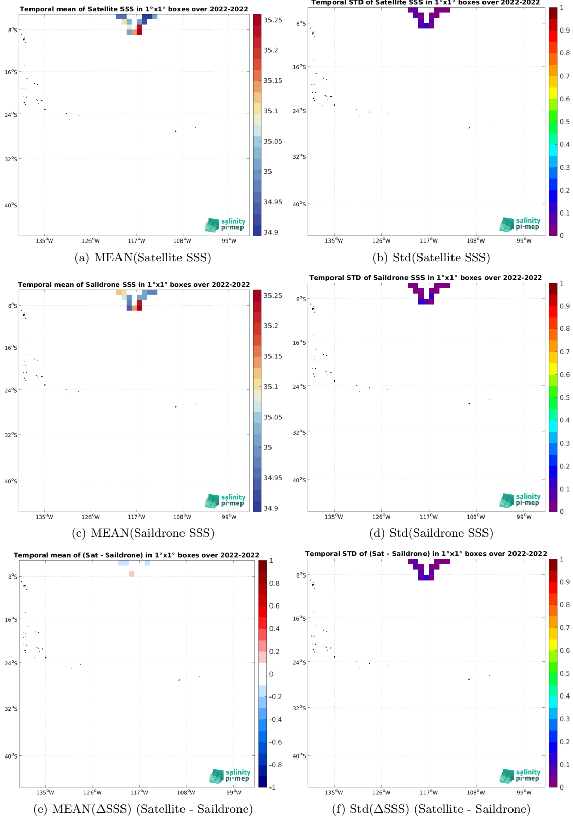
Figure 7: Temporal mean (left) and Std (right) of SSS from SMAP SSS L3 v5.3 - 8-Day running (RSS) (top), Saildrone (middle), and of \Delta SSS (Satellite - Saildrone). Only match-up pairs are used to generate these maps.
