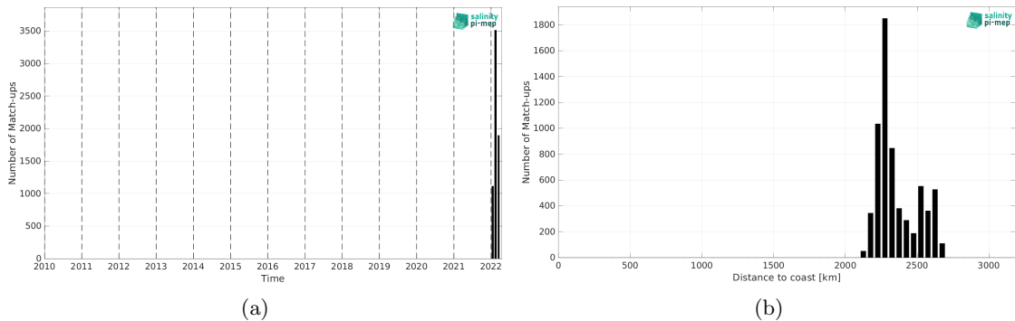
Figure 2: Number of match-ups between Saildrone and SMAP SSS L3 v5.3 - 8-Day running (RSS) SSS as a function of time (a) and as function of the distance to coast (b) over the OTT zone Pi-MEP region and for the full satellite product period.
