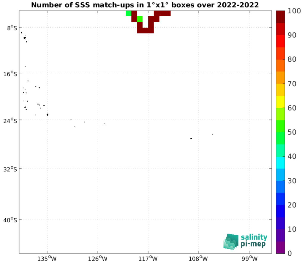
Figure 5: Number of SSS match-ups between Saifdrone SSS and the SMAP SSS L3 v5.3 - 8-Day running (RSS) SSS product for the OTT zone Pi-MEP region over 1^\circ \times 1^\circ boxes and for the full satellite product period.
