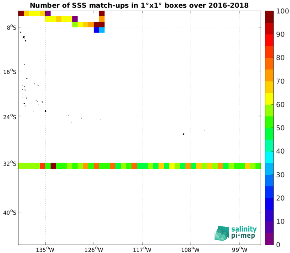
Figure 5: Number of SSS match-ups between TSG (SAMOS) SSS and the SMAP SSS L3 v5.3 - Monthly (RSS) SSS product for the OTT zone Pi-MEP region over 1^\circ \times 1^\circ boxes and for the full satellite product period.
