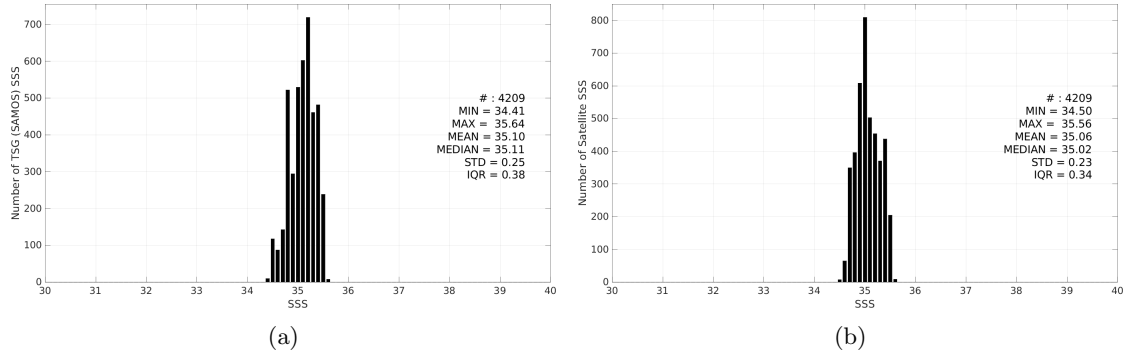
Figure 3: Histograms of SSS from TSG (SAMOS) (a) and SMAP SSS L3 v5.3 - Monthly (RSS) (b) considering all match-up pairs per bins of 0.1 over the OTT zone Pi-MEP region and for the full satellite product period.
