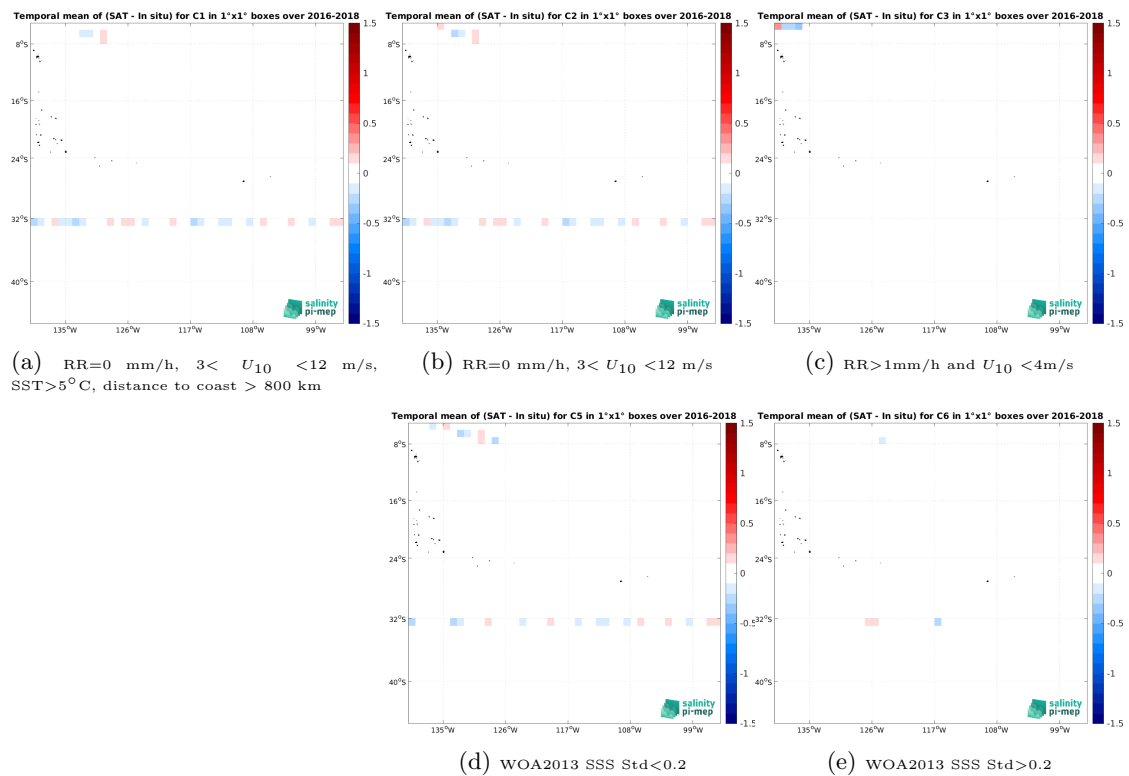
Figure 14: Temporal mean gridded over spatial boxes of size 1^\circ \times 1^\circ of \Delta SSS (SMAP SSS L3 v5.3 - Monthly (RSS) - TSG (SAMOS)) for 5 different subdatasets corresponding to: RR=0 mm/h, 3 < U_{10} < 12 m/s, SST > 5^\circ C , distance to coast > 800 km (a), RR=0 mm/h, 3 < U_{10} < 12 m/s (b), RR > 1 mm/h and U_{10} < 4 m/s (c), WOA2013 SSS Std < 0.2 (d), WOA2013 SSS Std > 0.2 (e).
