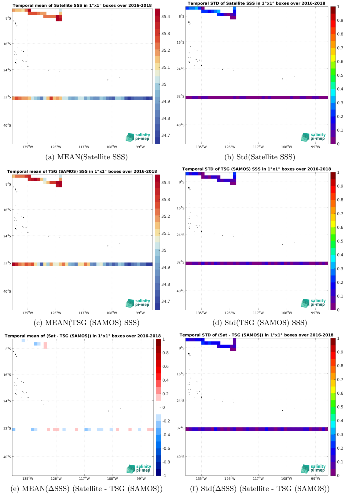
Figure 7: Temporal mean (left) and Std (right) of SSS from SMAP SSS L3 v5.3 - Monthly (RSS) (top), TSG (SAMOS) (middle), and of \Delta SSS (Satellite - TSG (SAMOS)). Only match-up pairs are used to generate these maps.
