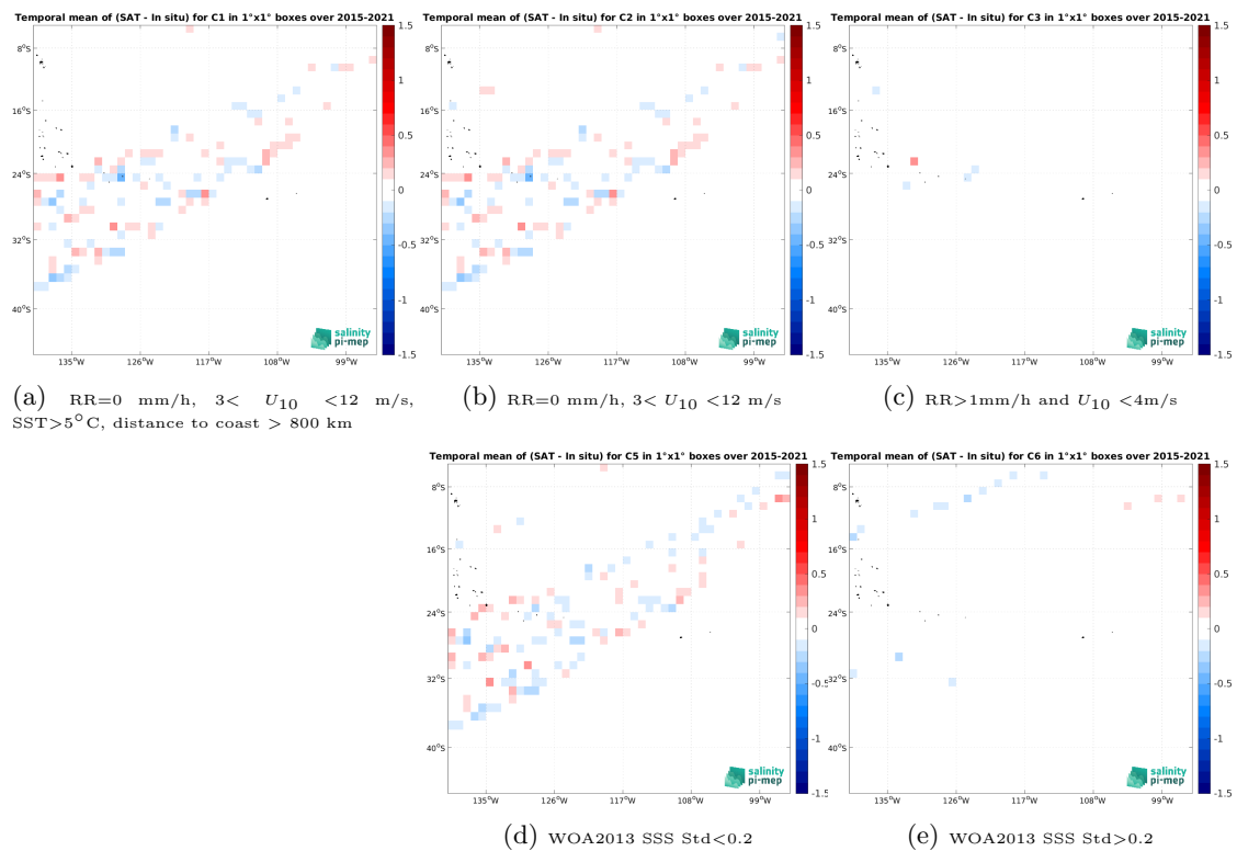
Figure 14: Temporal mean gridded over spatial boxes of size 1^\circ \times 1^\circ of \Delta SSS (SMAP SSS L3 v5.3 - Monthly (RSS) - TSG (LEGOS-DM)) for 5 different subdatasets corresponding to:RR=0 mm/h, 3 < U_{10} < 12 m/s, SST >5^\circ\text{C} , distance to coast > 800 km (a), RR=0 mm/h, 3 < U_{10} < 12 m/s (b), RR >1 mm/h and U_{10} < 4 m/s (c), WOA2013 SSS Std <0.2 (d), WOA2013 SSS Std >0.2 (e).
