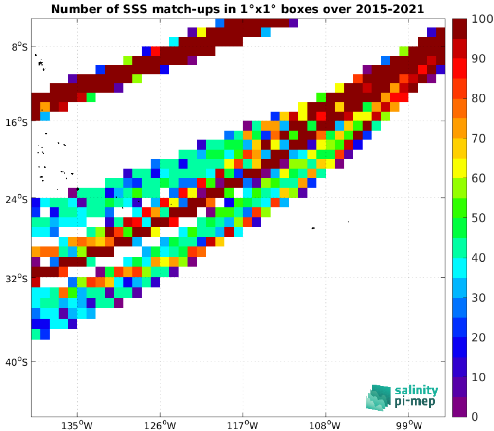
Figure 5: Number of SSS match-ups between TSG (LEGOS-DM) SSS and the SMAP SSS L3 v5.3 - Monthly (RSS) SSS product for the OTT zone Pi-MEP region over 1^\circ \times 1^\circ boxes and for the full satellite product period.
