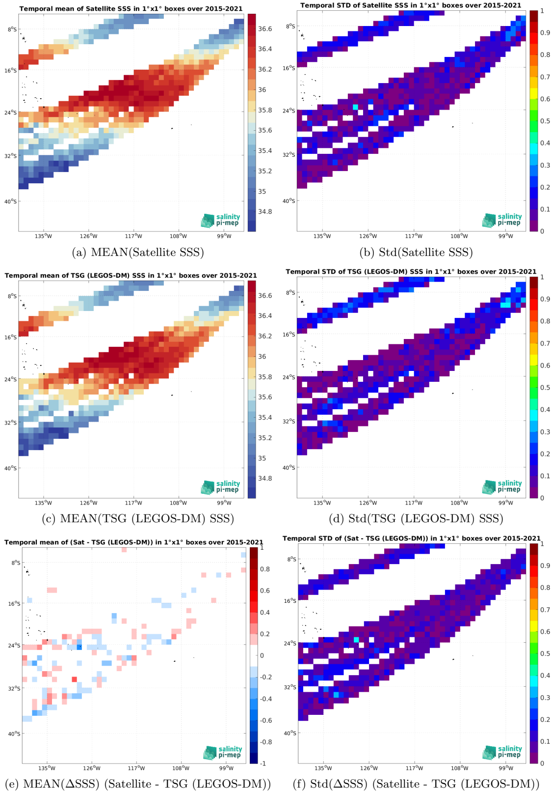
Figure 7: Temporal mean (left) and Std (right) of SSS from SMAP SSS L3 v5.3 - Monthly (RSS) (top), TSG (LEGOS-DM) (middle), and of \Delta SSS (Satellite - TSG (LEGOS-DM)). Only match-up pairs are used to generate these maps.
