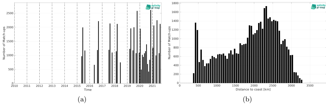
Figure 2: Number of match-ups between TSG (LEGOS-DM) and SMAP SSS L3 v5.3 - Monthly (RSS) SSS as a function of time (a) and as function of the distance to coast (b) over the OTT zone Pi-MEP region and for the full satellite product period.
