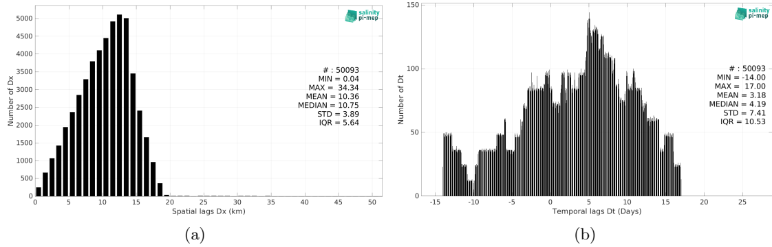
Figure 6: Histograms of the spatial (a) and temporal (b) lags between the location/time of the TSG (LEGOS-DM) measurement and the date of the corresponding SMAP SSS L3 v5.3 - Monthly (RSS) SSS pixel.
