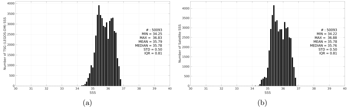
Figure 3: Histograms of SSS from TSG (LEGOS-DM) (a) and SMAP SSS L3 v5.3 - Monthly (RSS) (b) considering all match-up pairs per bins of 0.1 over the OTT zone Pi-MEP region and for the full satellite product period.
