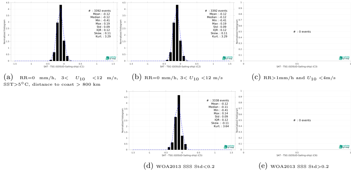
Figure 15: Normalized histogram of \Delta\text{SSS} (SMAP SSS L3 v5.3 - Monthly (RSS) - TSG (GOSUD-Sailing-ship)) for 5 different subdatasets corresponding to: RR=0 mm/h, 3 < U_{10} < 12 m/s, SST > 5^\circ\text{C} , distance to coast > 800 km (a), RR=0 mm/h, 3 < U_{10} < 12 m/s (b), RR > 1\text{mm/h} and U_{10} < 4\text{m/s} (c), WOA2013 SSS \text{Std} < 0.2 (d), WOA2013 SSS \text{Std} > 0.2 (e).
