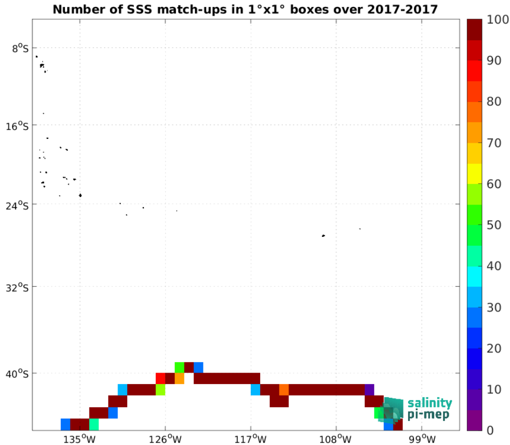
Figure 5: Number of SSS match-ups between TSG (GOSUD-Sailing-ship) SSS and the SMAP SSS L3 v5.3 - Monthly (RSS) SSS product for the OTT zone Pi-MEP region over 1^\circ \times 1^\circ boxes and for the full satellite product period.
