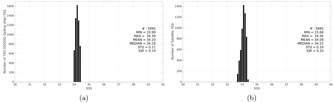
Figure 3: Histograms of SSS from TSG (GOSUD-Sailing-ship) (a) and SMAP SSS L3 v5.3 - Monthly (RSS) (b) considering all match-up pairs per bins of 0.1 over the OTT zone Pi-MEP region and for the full satellite product period.
