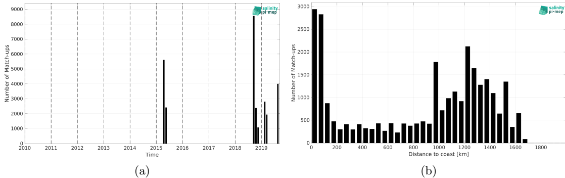
Figure 2: Number of match-ups between TSG (GOSUD-Research-vessel) and SMAP SSS L3 v5.3 - Monthly (RSS) SSS as a function of time (a) and as function of the distance to coast (b) over the OTT zone Pi-MEP region and for the full satellite product period.
