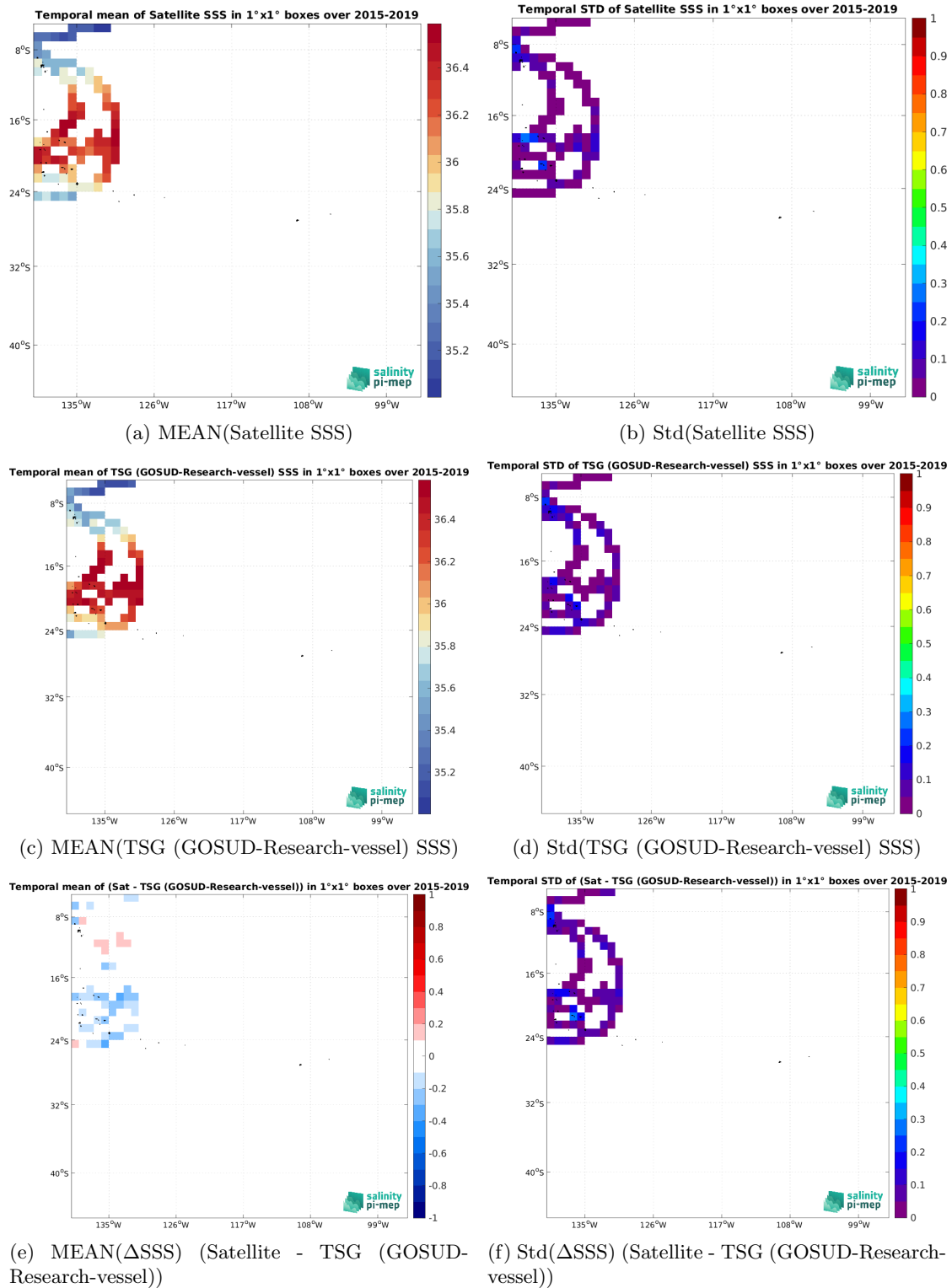
Figure 7: Temporal mean (left) and Std (right) of SSS from SMAP SSS L3 v5.3 - Monthly (RSS) (top), TSG (GOSUD-Research-vessel) (middle), and of \Delta SSS (Satellite - TSG (GOSUD-Research-vessel)). Only match-up pairs are used to generate these maps.
