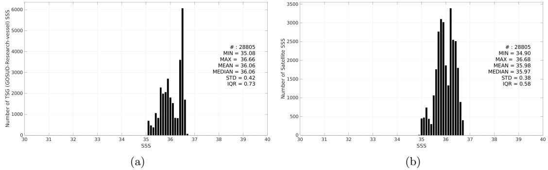
Figure 3: Histograms of SSS from TSG (GOSUD-Research-vessel) (a) and SMAP SSS L3 v5.3 - Monthly (RSS) (b) considering all match-up pairs per bins of 0.1 over the OTT zone Pi-MEP region and for the full satellite product period.
