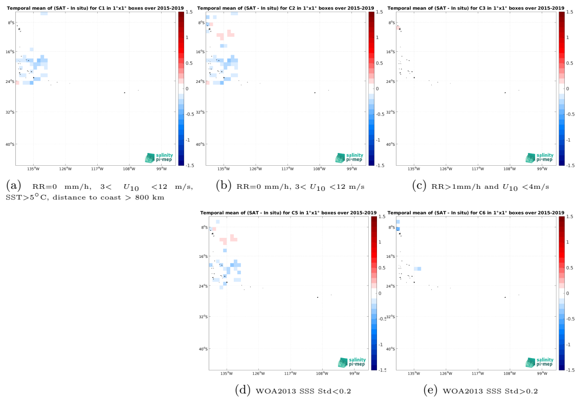
Figure 14: Temporal mean gridded over spatial boxes of size 1^\circ \times 1^\circ of \Delta SSS (SMAP SSS L3 v5.3 - Monthly (RSS) - TSG (GOSUD-Research-vessel)) for 5 different subdatasets corresponding to:RR=0 mm/h, 3 < U_{10} < 12 m/s, SST >5^\circ\text{C} , distance to coast > 800 km (a), RR=0 mm/h, 3 < U_{10} < 12 m/s (b), RR >1 mm/h and U_{10} < 4 m/s (c), WOA2013 SSS Std <0.2 (d), WOA2013 SSS Std >0.2 (e).
