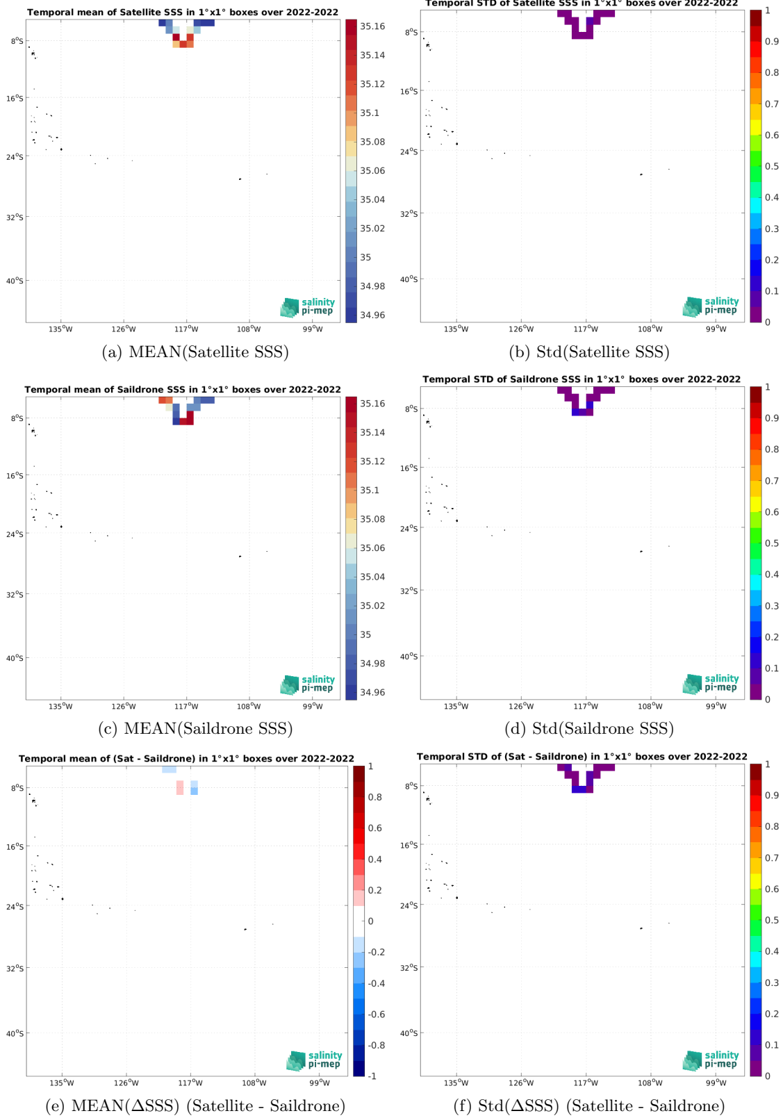
Figure 7: Temporal mean (left) and Std (right) of SSS from SMAP SSS L3 v5.3 - Monthly (RSS) (top), Saildrone (middle), and of \Delta SSS (Satellite - Saildrone). Only match-up pairs are used to generate these maps.
