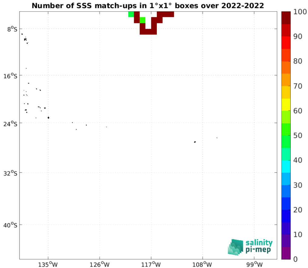
Figure 5: Number of SSS match-ups between Saildrone SSS and the SMAP SSS L3 v5.3 - Monthly (RSS) SSS product for the OTT zone Pi-MEP region over 1^\circ \times 1^\circ boxes and for the full satellite product period.
