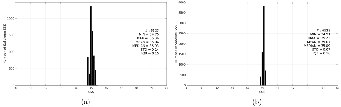
Figure 3: Histograms of SSS from Saildrone (a) and SMAP SSS L3 v5.3 - Monthly (RSS) (b) considering all match-up pairs per bins of 0.1 over the OTT zone Pi-MEP region and for the full satellite product period.
