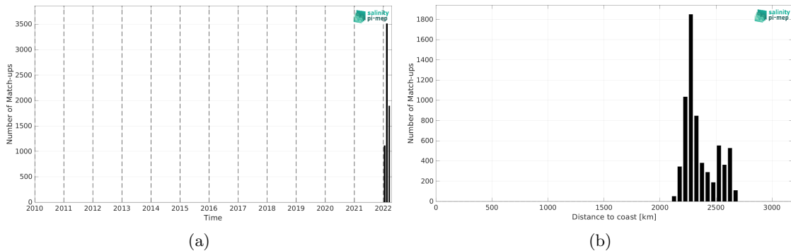
Figure 2: Number of match-ups between Saildrone and SMAP SSS L3 v5.3 - Monthly (RSS) SSS as a function of time (a) and as function of the distance to coast (b) over the OTT zone Pi-MEP region and for the full satellite product period.
