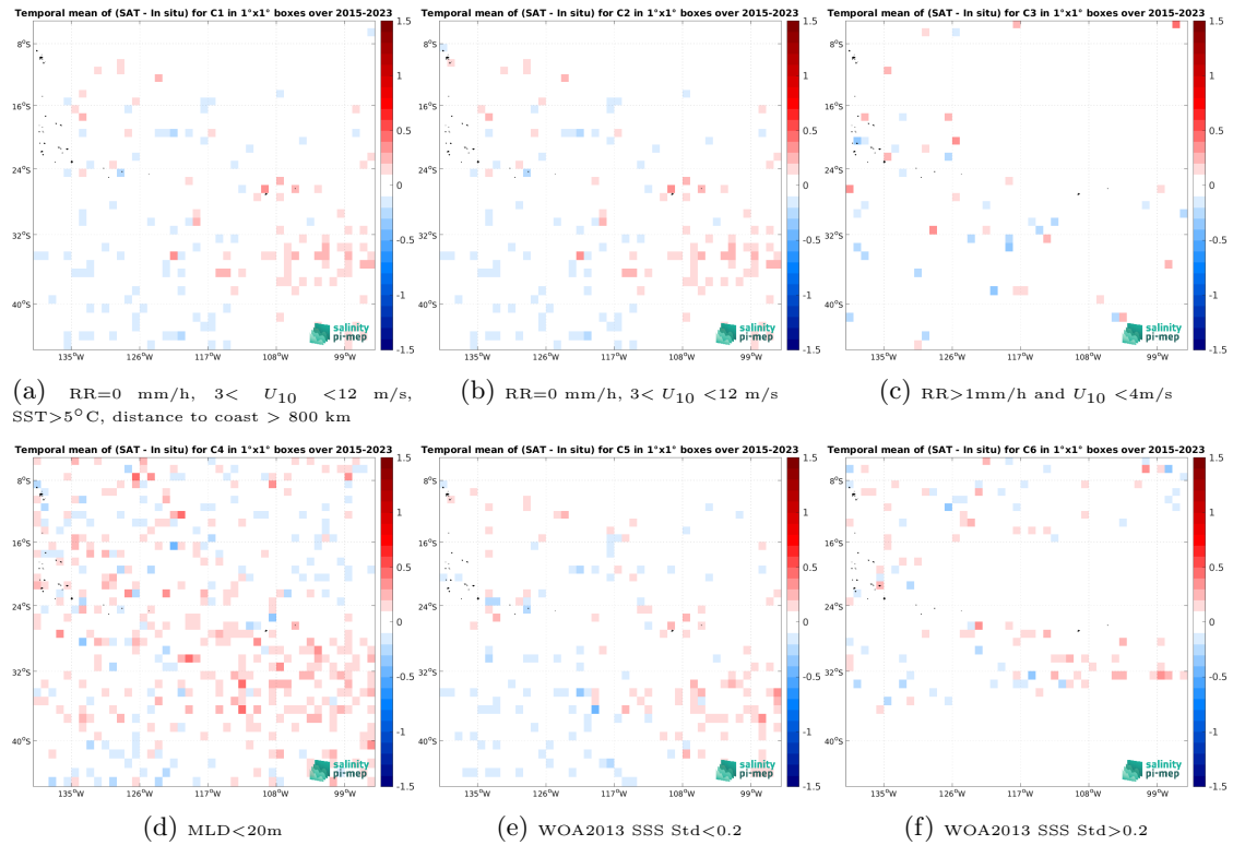
Figure 14: Temporal mean gridded over spatial boxes of size 1^\circ \times 1^\circ of \Delta SSS (SMAP SSS L3 v5.3 - Monthly (RSS) - Argo) for 6 different subdatasets corresponding to: RR=0 mm/h, 3 < U_{10} < 12 m/s, SST > 5^\circ C , distance to coast > 800 km (a), RR=0 mm/h, 3 < U_{10} < 12 m/s (b), RR > 1 mm/h and U_{10} < 4 m/s (c), MLD < 20 m (d), WOA2013 SSS Std < 0.2 (e), WOA2013 SSS Std > 0.2 (f).
