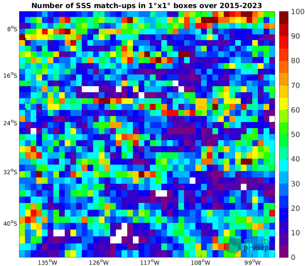
Figure 5: Number of SSS match-ups between Argo SSS and the SMAP SSS L3 v5.3 - Monthly (RSS) SSS product for the OTT zone Pi-MEP region over 1^\circ \times 1^\circ boxes and for the full satellite product period.
