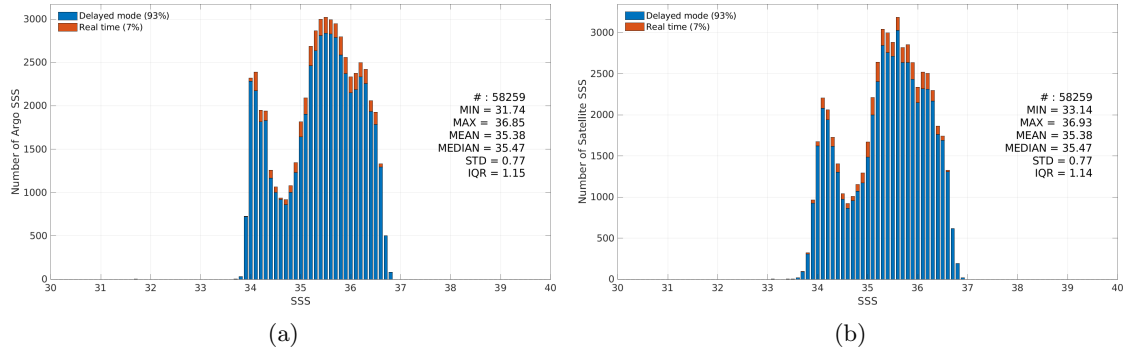
Figure 3: Histograms of SSS from Argo (a) and SMAP SSS L3 v5.3 - Monthly (RSS) (b) considering all match-up pairs per bins of 0.1 over the OTT zone Pi-MEP region and for the full satellite product period.
