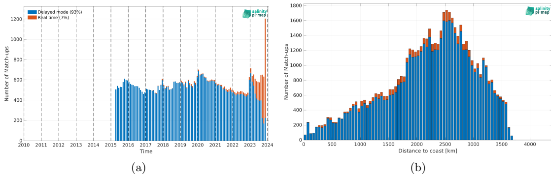
Figure 2: Number of match-ups between Argo and SMAP SSS L3 v5.3 - Monthly (RSS) SSS as a function of time (a) and as function of the distance to coast (b) over the OTT zone Pi-MEP region and for the full satellite product period.
