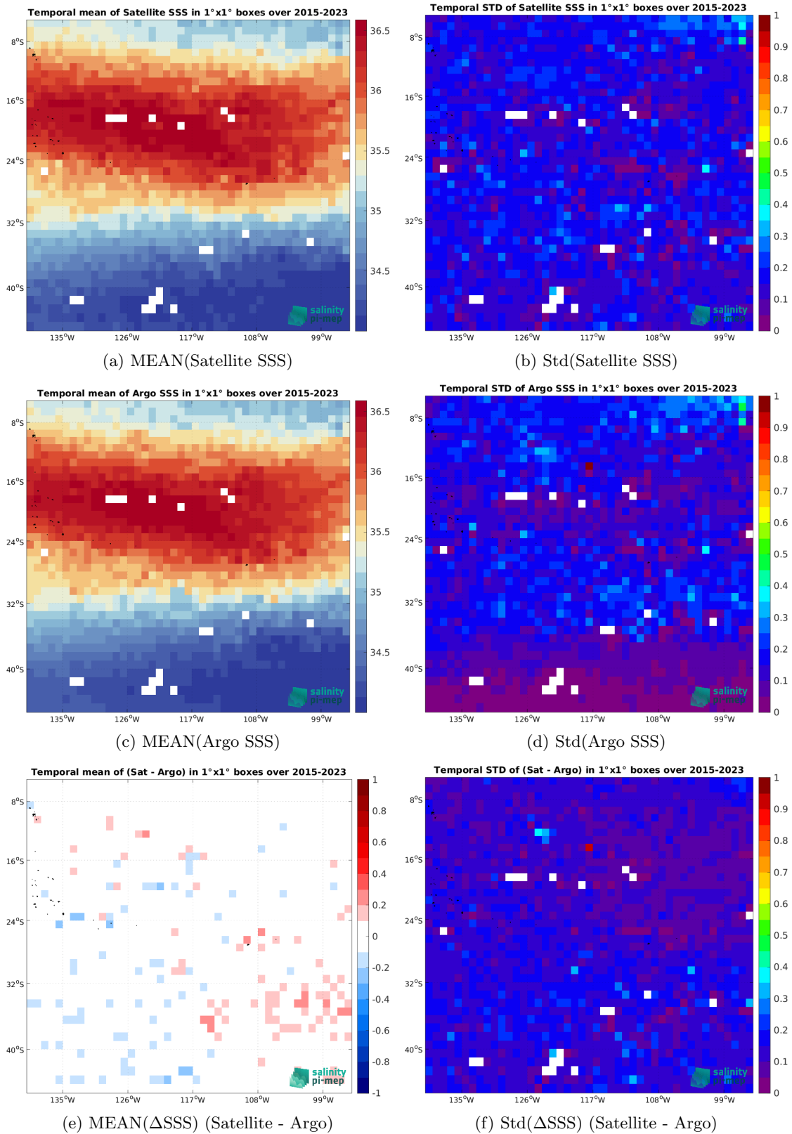
Figure 7: Temporal mean (left) and Std (right) of SSS from SMAP SSS L3 v5.3 - Monthly (RSS) (top), Argo (middle), and of \Delta SSS (Satellite - Argo). Only match-up pairs are used to generate these maps.
