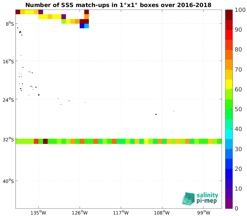
Figure 4: Number of SSS match-ups between TSG (SAMOS) SSS and the SMAP SSS L3 v5 - 8-Day running (RSS) SSS product for the OTT zone Pi-MEP region over 1°x1° boxes and for the full satellite product period.
