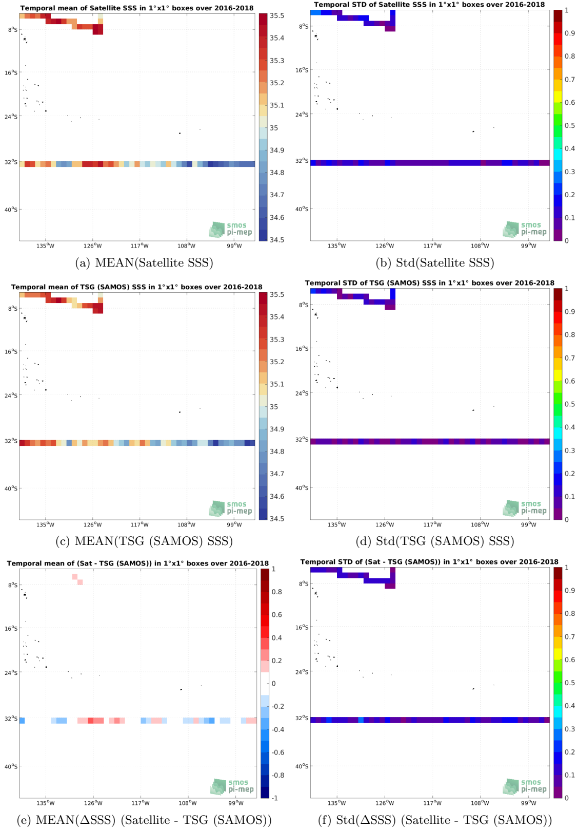
Figure 6: Temporal mean (left) and Std (right) of SSS from SMAP SSS L3 v5 - 8-Day running (RSS) (top), TSG (SAMOS) (middle), and of \Delta SSS (Satellite - TSG (SAMOS)). Only match-up pairs are used to generate these maps.
