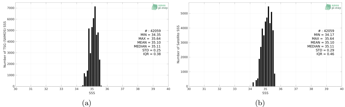
Figure 2: Histograms of SSS from TSG (SAMOS) (a) and SMAP SSS L3 v5 - 8-Day running (RSS) (b) considering all match-up pairs per bins of 0.1 over the OTT zone Pi-MEP region and for the full satellite product period.
