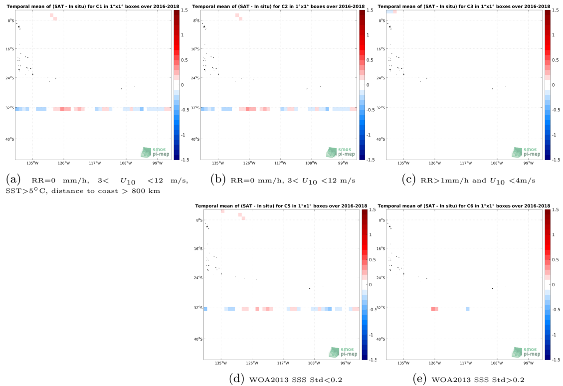
Figure 12: Temporal mean gridded over spatial boxes of size 1^\circ \times 1^\circ of \Delta SSS (SMAP SSS L3 v5 - 8-Day running (RSS) - TSG (SAMOS)) for 5 different subdatasets corresponding to: RR=0 mm/h, 3 < U_{10} < 12 m/s, SST > 5^\circ C , distance to coast > 800 km (a), RR=0 mm/h, 3 < U_{10} < 12 m/s (b), RR > 1 mm/h and U_{10} < 4 m/s (c), WOA2013 SSS Std < 0.2 (d), WOA2013 SSS Std > 0.2 (e).
