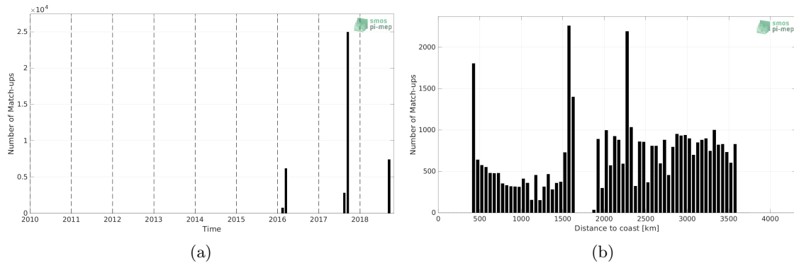
Figure 1: Number of match-ups between TSG (SAMOS) and SMAP SSS L3 v5 - 8-Day running (RSS) SSS as a function of time (a) and as function of the distance to coast (b) over the OTT zone Pi-MEP region and for the full satellite product period.
