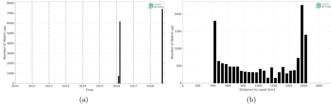
Figure 1: Number of match-ups between TSG (SAMOS) and SMAP SSS L3 v5 - 8-Day running (RSS) SSS as a function of time (a) and as function of the distance to coast (b) over the OTT zone Pi-MEP region and for the full satellite product period.
