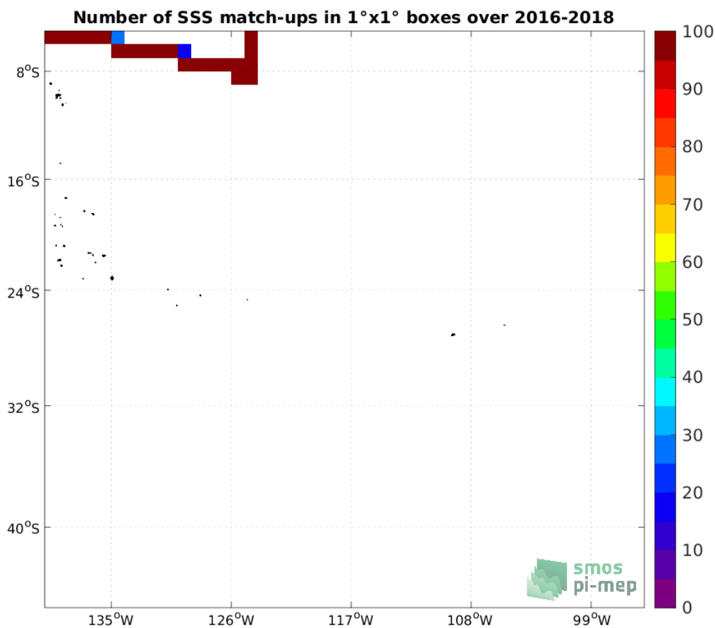
Figure 4: Number of SSS match-ups between TSG (SAMOS) SSS and the SMAP SSS L3 v5 - 8-Day running (RSS) SSS product for the OTT zone Pi-MEP region over 1°×1° boxes and for the full satellite product period.
