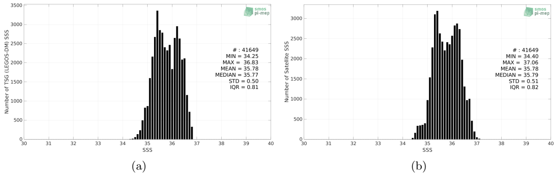
Figure 2: Histograms of SSS from TSG (LEGOS-DM) (a) and SMAP SSS L3 v5 - 8-Day running (RSS) (b) considering all match-up pairs per bins of 0.1 over the OTT zone Pi-MEP region and for the full satellite product period.
