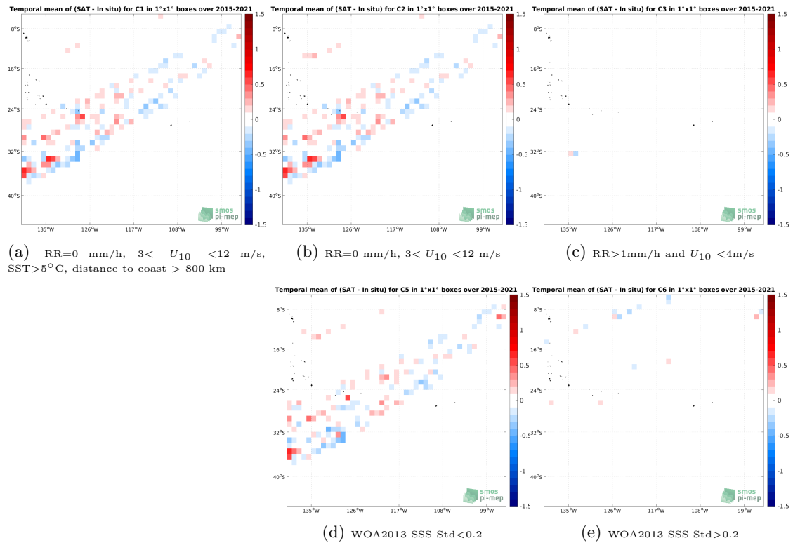
Figure 12: Temporal mean gridded over spatial boxes of size 1^\circ \times 1^\circ of \Delta SSS (SMAP SSS L3 v5 - 8-Day running (RSS) - TSG (LEGOS-DM)) for 5 different subdatasets corresponding to: RR=0 mm/h, 3 < U_{10} < 12 m/s, SST > 5^\circ C , distance to coast > 800 km (a), RR=0 mm/h, 3 < U_{10} < 12 m/s (b), RR > 1 mm/h and U_{10} < 4 m/s (c), WOA2013 SSS Std < 0.2 (d), WOA2013 SSS Std > 0.2 (e).
