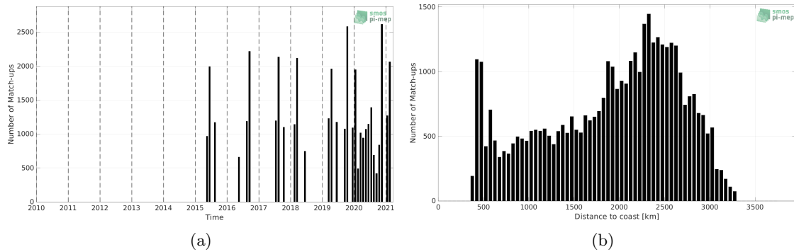
Figure 1: Number of match-ups between TSG (LEGOS-DM) and SMAP SSS L3 v5 - 8-Day running (RSS) SSS as a function of time (a) and as function of the distance to coast (b) over the OTT zone Pi-MEP region and for the full satellite product period.
