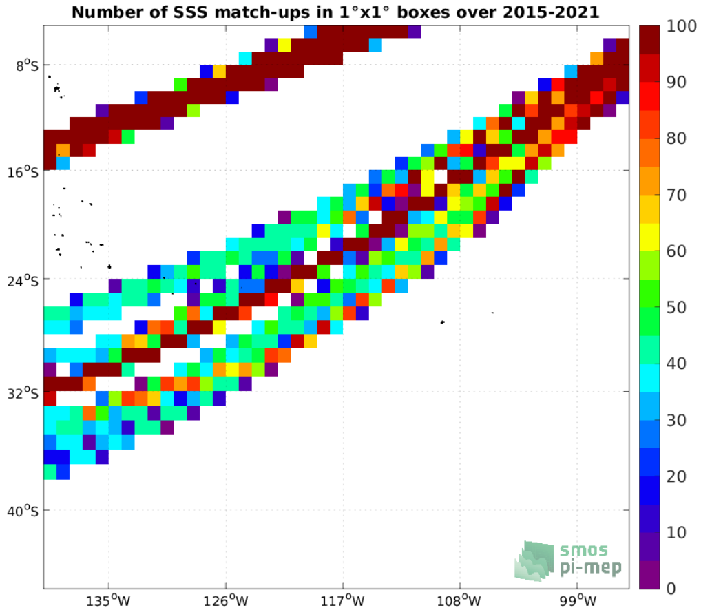
Figure 4: Number of SSS match-ups between TSG (LEGOS-DM) SSS and the SMAP SSS L3 v5 - 8-Day running (RSS) SSS product for the OTT zone Pi-MEP region over 1°×1° boxes and for the full satellite product period.
