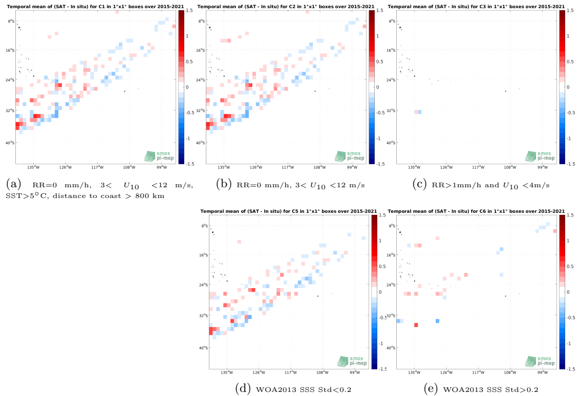
Figure 12: Temporal mean gridded over spatial boxes of size 1^\circ \times 1^\circ of \Delta SSS (SMAP SSS L3 v5 - 8-Day running (RSS) - TSG (LEGOS-DM)) for 5 different subdatasets corresponding to:RR=0 mm/h, 3 < U_{10} < 12 m/s, SST >5^\circ C, distance to coast > 800 km (a), RR=0 mm/h, 3 < U_{10} < 12 m/s (b), RR >1 mm/h and U_{10} < 4 m/s (c), WOA2013 SSS Std <0.2 (d), WOA2013 SSS Std >0.2 (e).
