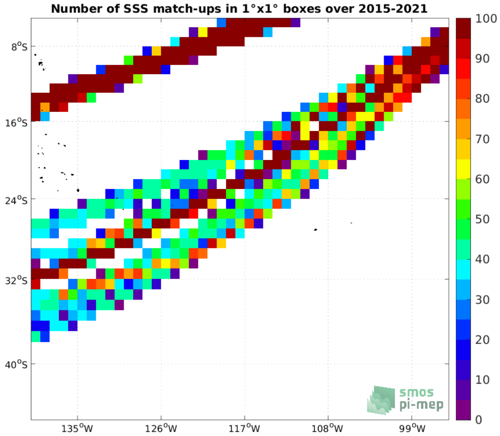
Figure 4: Number of SSS match-ups between TSG (LEGOS-DM) SSS and the SMAP SSS L3 v5 - 8-Day running (RSS) SSS product for the OTT zone Pi-MEP region over 1^\circ \times 1^\circ boxes and for the full satellite product period.
