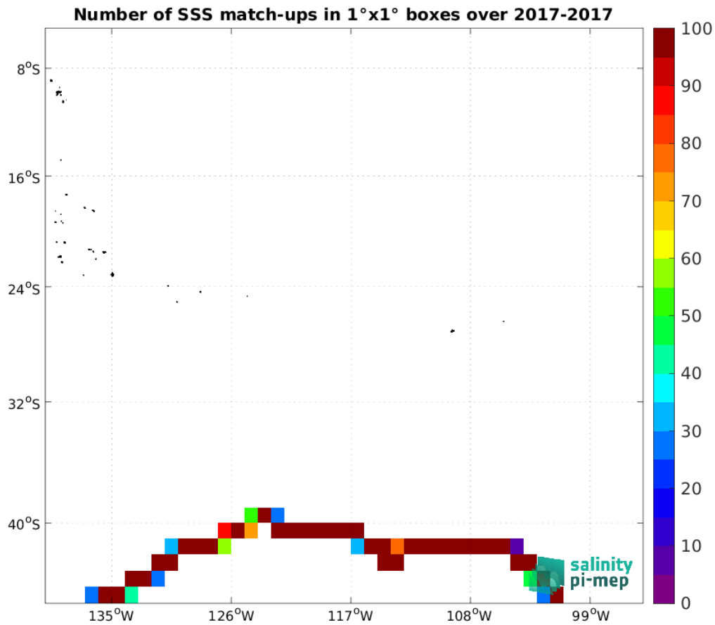
Figure 4: Number of SSS match-ups between TSG (GOSUD-Sailing-ship) SSS and the SMAP SSS L3 v5 - 8-Day running (RSS) SSS product for the OTT zone Pi-MEP region over 1°x1° boxes and for the full satellite product period.
