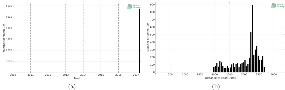
Figure 1: Number of match-ups between TSG (GOSUD-Sailing-ship) and SMAP SSS L3 v5 - 8-Day running (RSS) SSS as a function of time (a) and as function of the distance to coast (b) over the OTT zone Pi-MEP region and for the full satellite product period.
