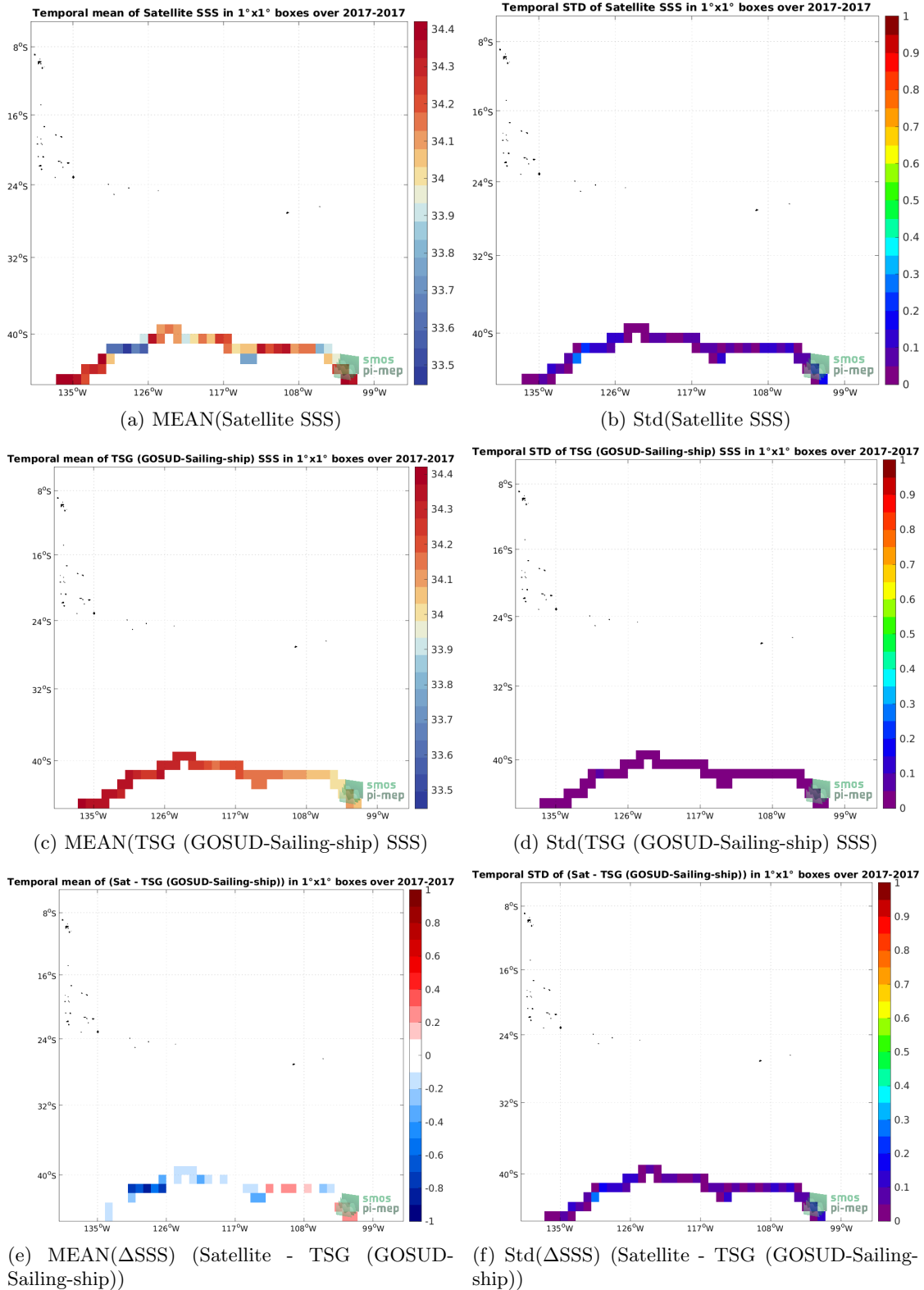
Figure 6: Temporal mean (left) and Std (right) of SSS from SMAP SSS L3 v5 - 8-Day running (RSS) (top), TSG (GOSUD-Sailing-ship) (middle), and of \Delta SSS (Satellite - TSG (GOSUD-Sailing-ship)). Only match-up pairs are used to generate these maps.
