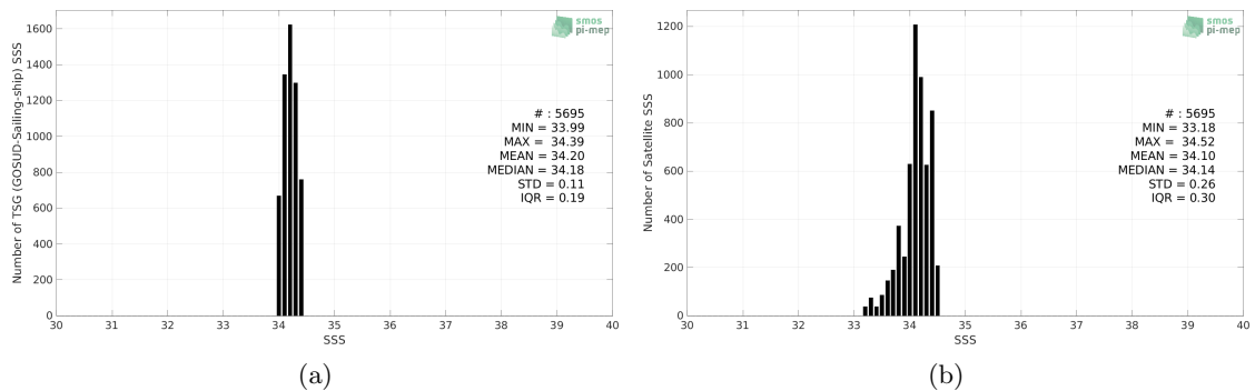
Figure 2: Histograms of SSS from TSG (GOSUD-Sailing-ship) (a) and SMAP SSS L3 v5 - 8-Day running (RSS) (b) considering all match-up pairs per bins of 0.1 over the OTT zone Pi-MEP region and for the full satellite product period.
