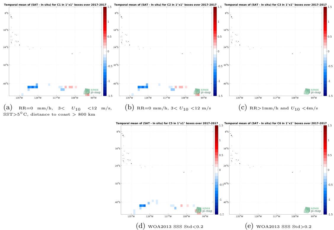
Figure 12: Temporal mean gridded over spatial boxes of size 1^\circ \times 1^\circ of \Delta SSS (SMAP SSS L3 v5 - 8-Day running (RSS) - TSG (GOSUD-Sailing-ship)) for 5 different subdatasets corresponding to:RR=0 mm/h, 3 < U_{10} < 12 m/s, SST >5^\circ C, distance to coast > 800 km (a), RR=0 mm/h, 3 < U_{10} < 12 m/s (b), RR >1 mm/h and U_{10} < 4 m/s (c), WOA2013 SSS Std <0.2 (d), WOA2013 SSS Std >0.2 (e).
