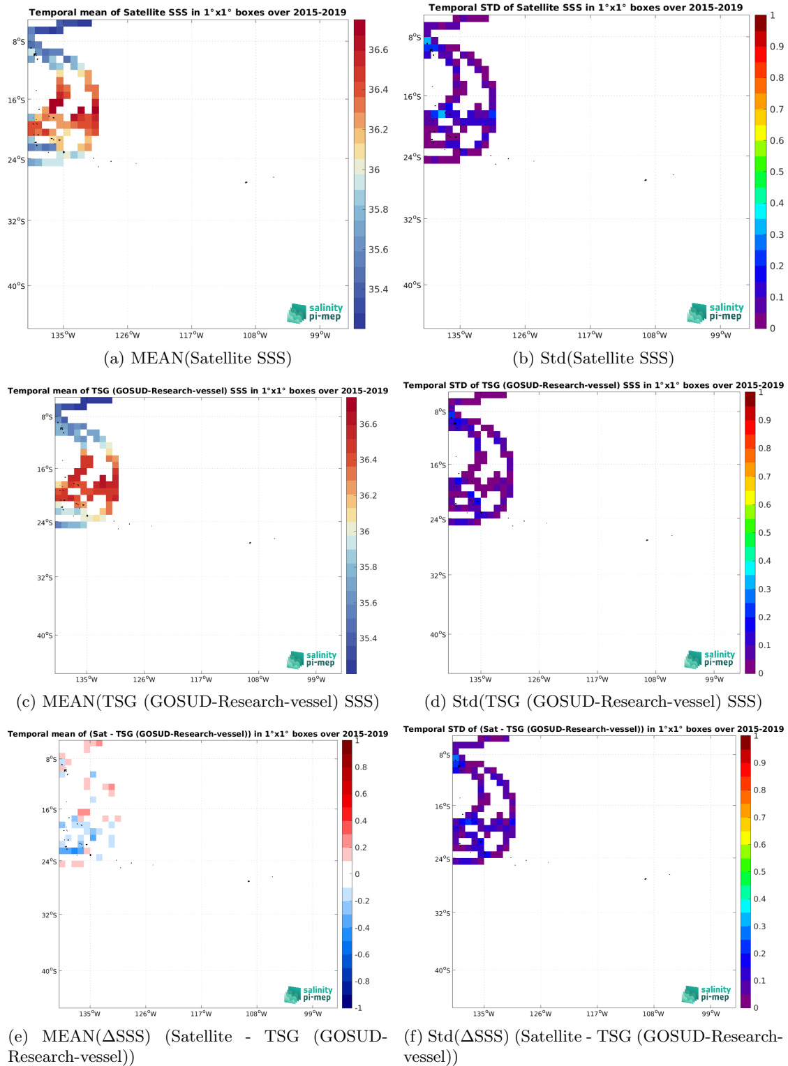
Figure 6: Temporal mean (left) and Std (right) of SSS from SMAP SSS L3 v5 - 8-Day running (RSS) (top), TSG (GOSUD-Research-vessel) (middle), and of \Delta SSS (Satellite - TSG (GOSUD-Research-vessel)). Only match-up pairs are used to generate these maps.
