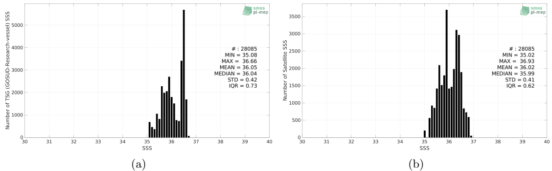
Figure 2: Histograms of SSS from TSG (GOSUD-Research-vessel) (a) and SMAP SSS L3 v5 - 8-Day running (RSS) (b) considering all match-up pairs per bins of 0.1 over the OTT zone Pi-MEP region and for the full satellite product period.
