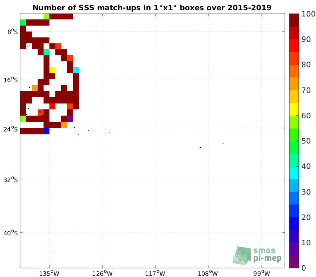
Figure 4: Number of SSS match-ups between TSG (GOSUD-Research-vessel) SSS and the SMAP SSS L3 v5 - 8-Day running (RSS) SSS product for the OTT zone Pi-MEP region over 1°x1° boxes and for the full satellite product period.
