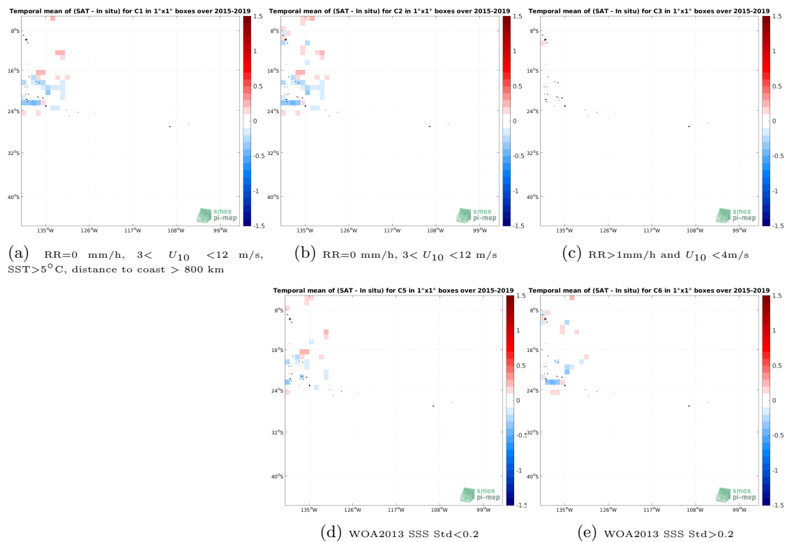
Figure 12: Temporal mean gridded over spatial boxes of size 1^\circ \times 1^\circ of \Delta SSS (SMAP SSS L3 v5 - 8-Day running (RSS) - TSG (GOSUD-Research-vessel)) for 5 different subdatasets corresponding to:RR=0 mm/h, 3 < U_{10} < 12 m/s, SST >5^\circ\text{C} , distance to coast > 800 km (a), RR=0 mm/h, 3 < U_{10} < 12 m/s (b), RR >1 mm/h and U_{10} < 4 m/s (c), WOA2013 SSS Std <0.2 (d), WOA2013 SSS Std >0.2 (e).
