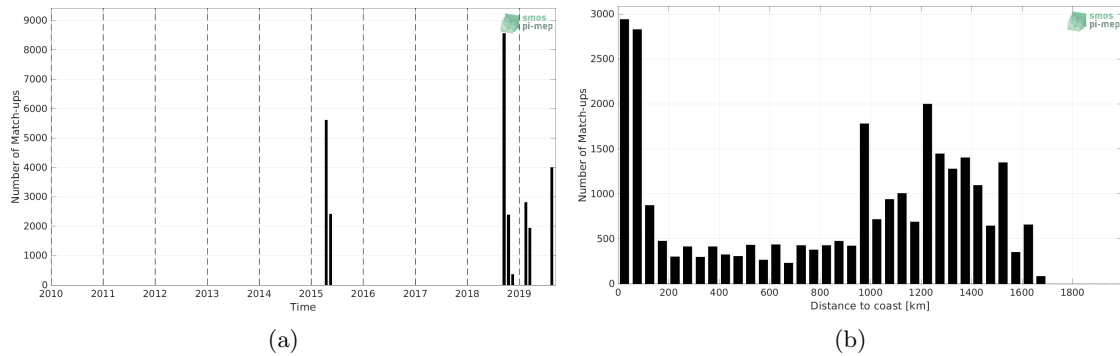
Figure 1: Number of match-ups between TSG (GOSUD-Research-vessel) and SMAP SSS L3 v5 - 8-Day running (RSS) SSS as a function of time (a) and as function of the distance to coast (b) over the OTT zone Pi-MEP region and for the full satellite product period.
