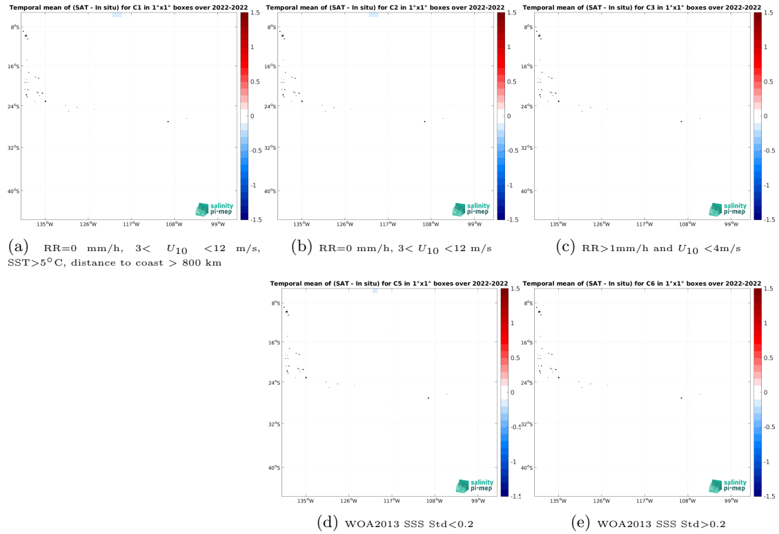
Figure 12: Temporal mean gridded over spatial boxes of size 1^\circ \times 1^\circ of \Delta SSS (SMAP SSS L3 v5 - 8-Day running (RSS) - Sairdrone) for 5 different subdatasets corresponding to: RR=0 mm/h, 3 < U_{10} < 12 m/s, SST > 5^\circ C , distance to coast > 800 km (a), RR=0 mm/h, 3 < U_{10} < 12 m/s (b), RR > 1 mm/h and U_{10} < 4 m/s (c), WOA2013 SSS Std < 0.2 (d), WOA2013 SSS Std > 0.2 (e).
