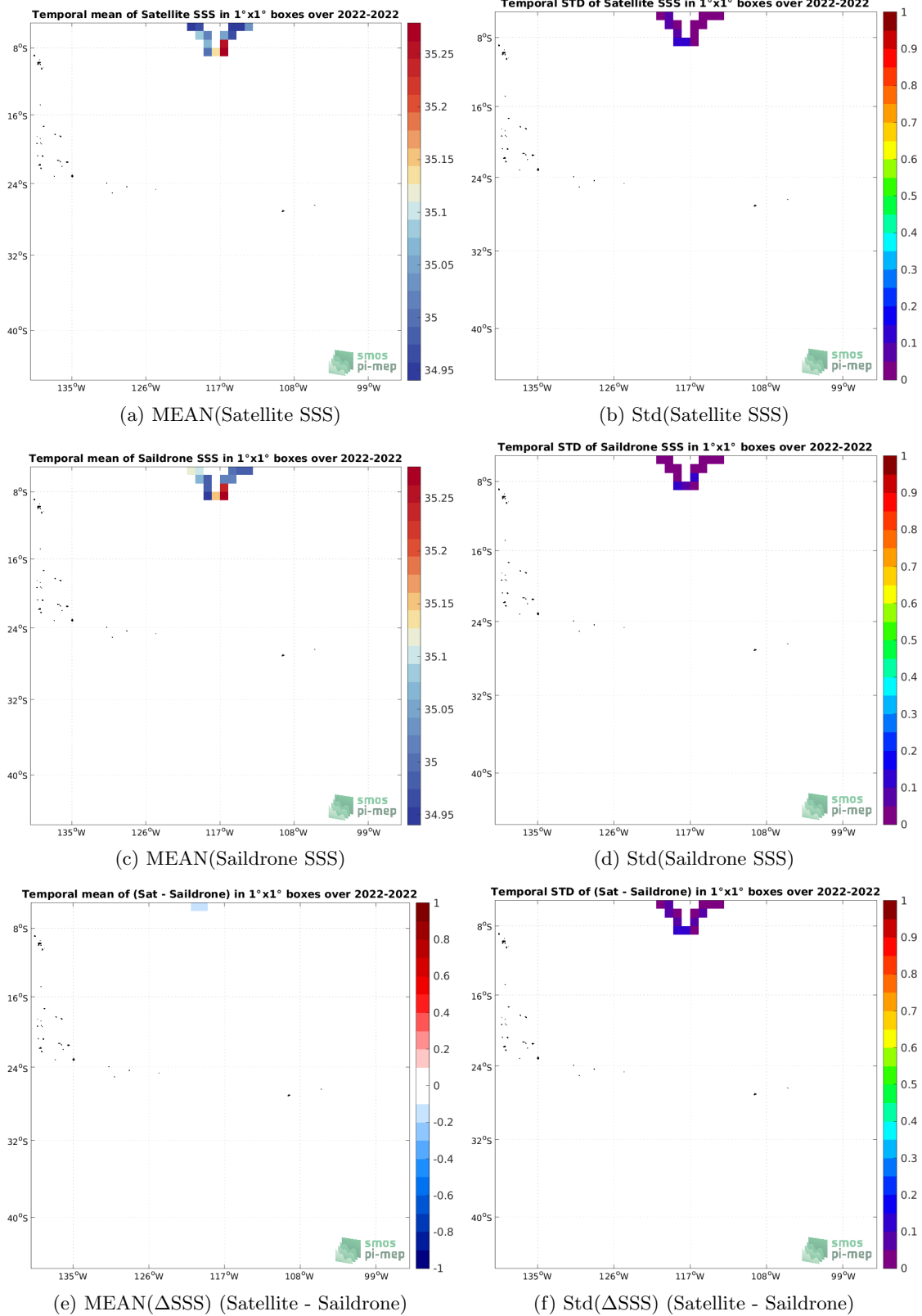
Figure 6: Temporal mean (left) and Std (right) of SSS from SMAP SSS L3 v5 - 8-Day running (RSS) (top), Saildrone (middle), and of \Delta SSS (Satellite - Saildrone). Only match-up pairs are used to generate these maps.
