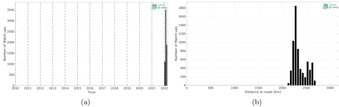
Figure 1: Number of match-ups between Saildrone and SMAP SSS L3 v5 - 8-Day running (RSS) SSS as a function of time (a) and as function of the distance to coast (b) over the OTT zone Pi-MEP region and for the full satellite product period.
