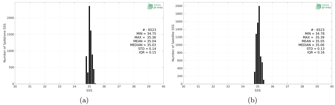
Figure 2: Histograms of SSS from Saildrone (a) and SMAP SSS L3 v5 - 8-Day running (RSS) (b) considering all match-up pairs per bins of 0.1 over the OTT zone Pi-MEP region and for the full satellite product period.
