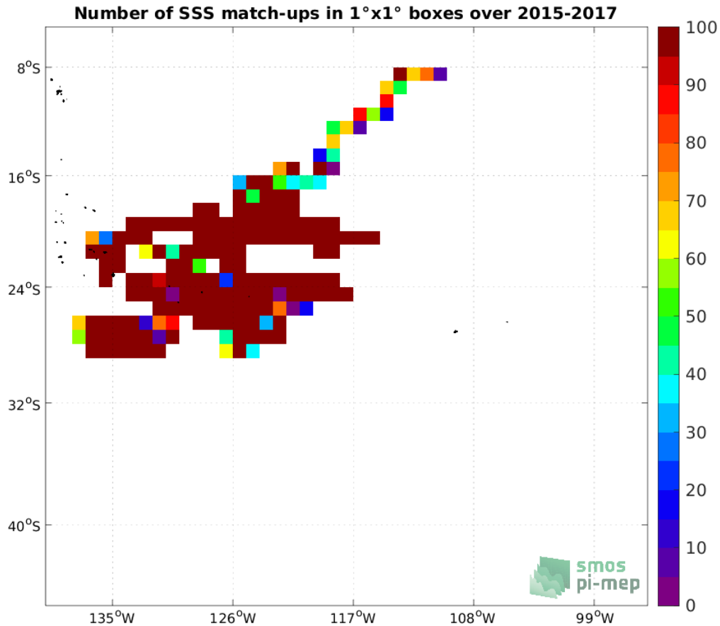
Figure 3: Number of SSS match-ups between Surface drifters SSS and the SMAP SSS L3 v5 - 8-Day running (RSS) SSS product for the OTT zone Pi-MEP region over 1^\circ \times 1^\circ boxes and for the full satellite product period.
