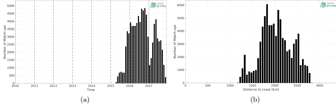
Figure 1: Number of match-ups between Surface drifters and SMAP SSS L3 v5 - 8-Day running (RSS) SSS as a function of time (a) and as function of the distance to coast (b) over the OTT zone Pi-MEP region and for the full satellite product period.
