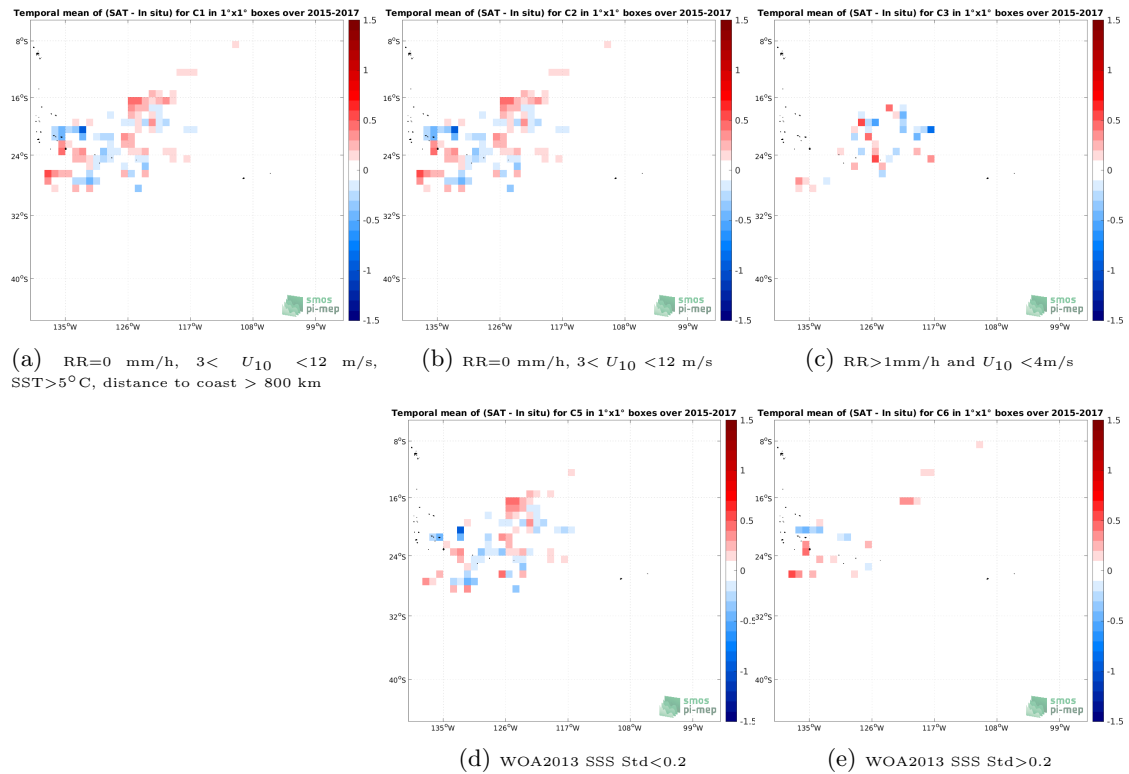
Figure 11: Temporal mean gridded over spatial boxes of size 1^\circ \times 1^\circ of \Delta SSS (SMAP SSS L3 v5 - 8-Day running (RSS) - Surface drifters) for 5 different subdatasets corresponding to:RR=0 mm/h, 3 < U_{10} < 12 m/s, SST >5^\circ C, distance to coast > 800 km (a), RR=0 mm/h, 3 < U_{10} < 12 m/s (b), RR >1 mm/h and U_{10} < 4 m/s (c), WOA2013 SSS Std <0.2 (d), WOA2013 SSS Std >0.2 (e).
