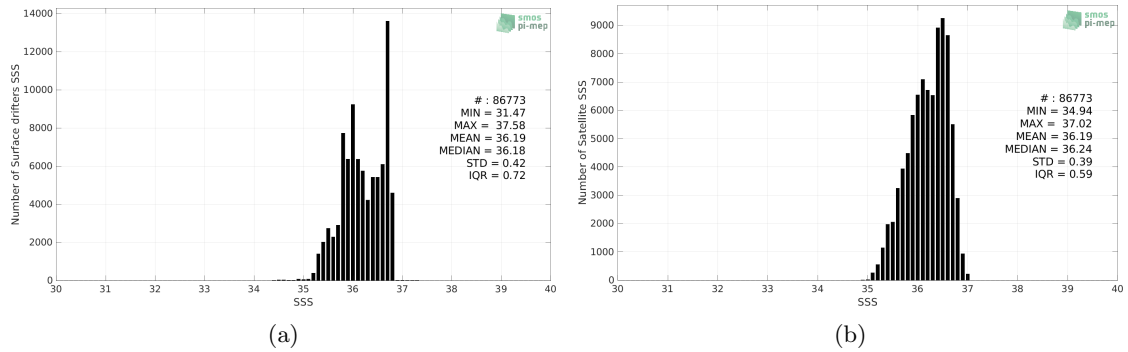
Figure 2: Histograms of SSS from Surface drifters (a) and SMAP SSS L3 v5 - 8-Day running (RSS) (b) considering all match-up pairs per bins of 0.1 over the OTT zone Pi-MEP region and for the full satellite product period.
