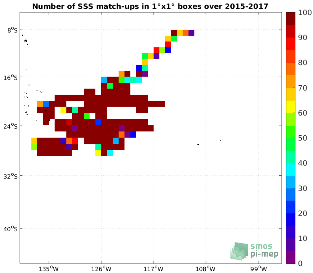
Figure 3: Number of SSS match-ups between Surface drifters SSS and the SMAP SSS L3 v5 - 8-Day running (RSS) SSS product for the OTT zone Pi-MEP region over 1°x1° boxes and for the full satellite product period.
