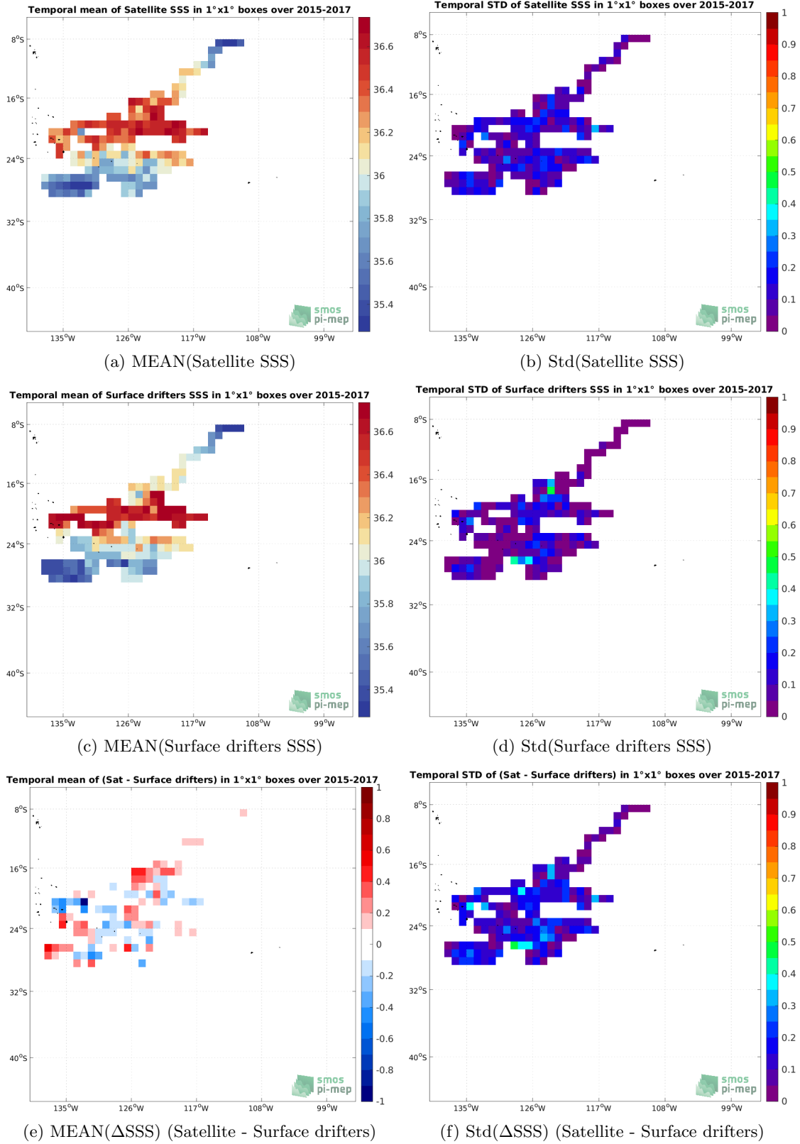
Figure 5: Temporal mean (left) and Std (right), of SSS from SMAP SSS L3 v5 - 8-Day running (RSS) (top), Surface drifters (middle), and of \Delta SSS (Satellite - Surface drifters). Only match-up pairs are used to generate these maps.
