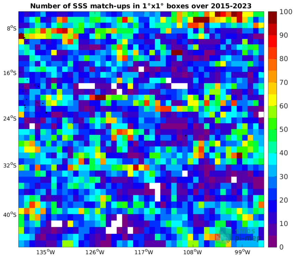
Figure 4: Number of SSS match-ups between Argo SSS and the SMAP SSS L3 v5 - 8-Day running (RSS) SSS product for the OTT zone Pi-MEP region over 1°x1° boxes and for the full satellite product period.
