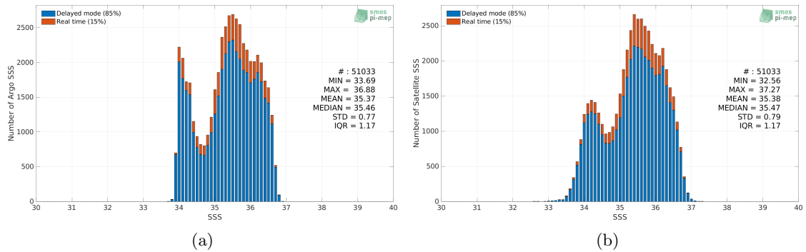
Figure 2: Histograms of SSS from Argo (a) and SMAP SSS L3 v5 - 8-Day running (RSS) (b) considering all match-up pairs per bins of 0.1 over the OTT zone Pi-MEP region and for the full satellite product period.
