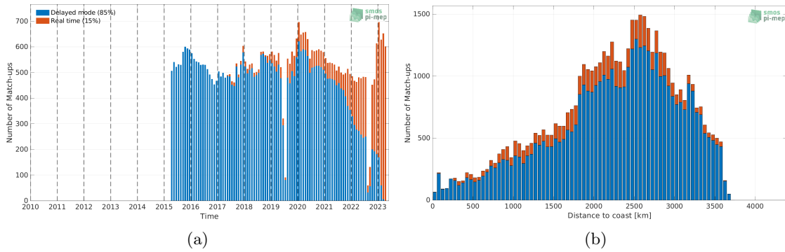
Figure 1: Number of match-ups between Argo and SMAP SSS L3 v5 - 8-Day running (RSS) SSS as a function of time (a) and as function of the distance to coast (b) over the OTT zone Pi-MEP region and for the full satellite product period.
