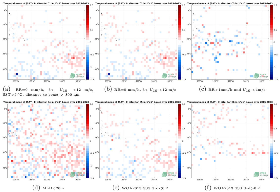
Figure 12: Temporal mean gridded over spatial boxes of size 1^\circ \times 1^\circ of \Delta SSS (SMAP SSS L3 v5 - 8-Day running (RSS) - Argo) for 6 different subdatasets corresponding to:RR=0 mm/h, 3 < U_{10} < 12 m/s, SST >5^\circ C, distance to coast > 800 km (a), RR=0 mm/h, 3 < U_{10} < 12 m/s (b), RR >1 mm/h and U_{10} < 4 m/s (c),MLD <20 m (d),WOA2013 SSS Std <0.2 (e),WOA2013 SSS Std >0.2 (f).
