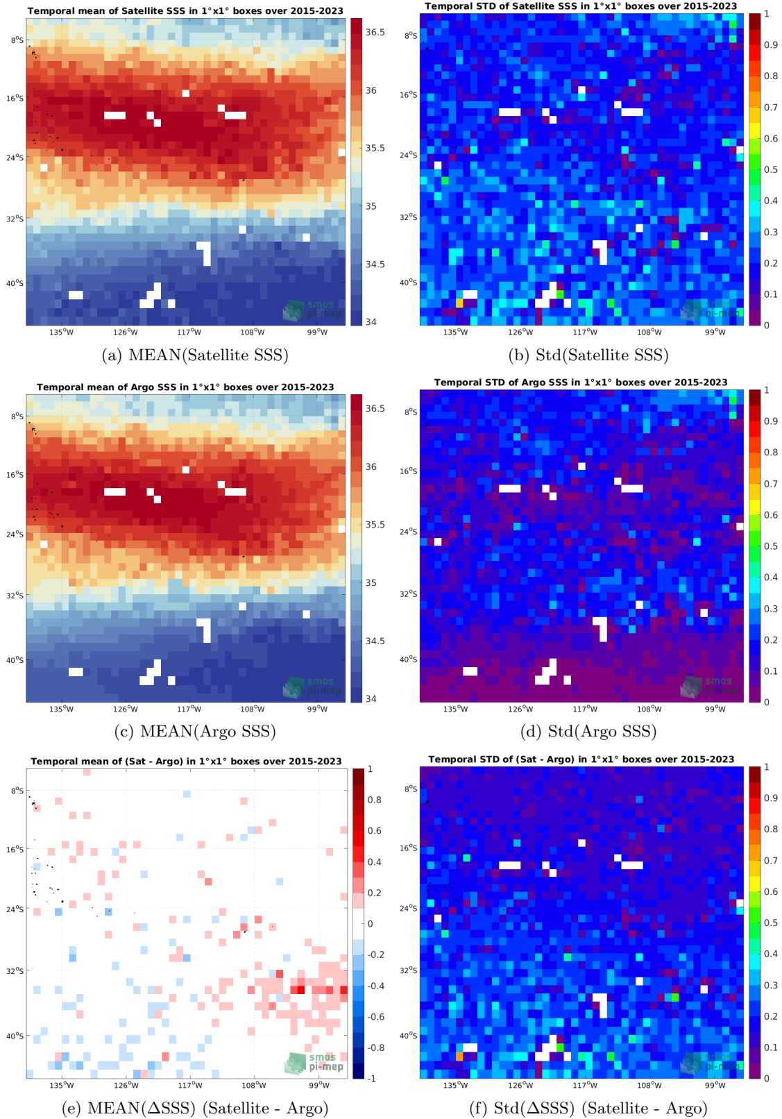
Figure 6: Temporal mean (left) and Std (right) of SSS from SMAP SSS L3 v5 - 8-Day running (RSS) (top), Argo (middle), and of \Delta SSS (Satellite - Argo). Only match-up pairs are used to generate these maps.
