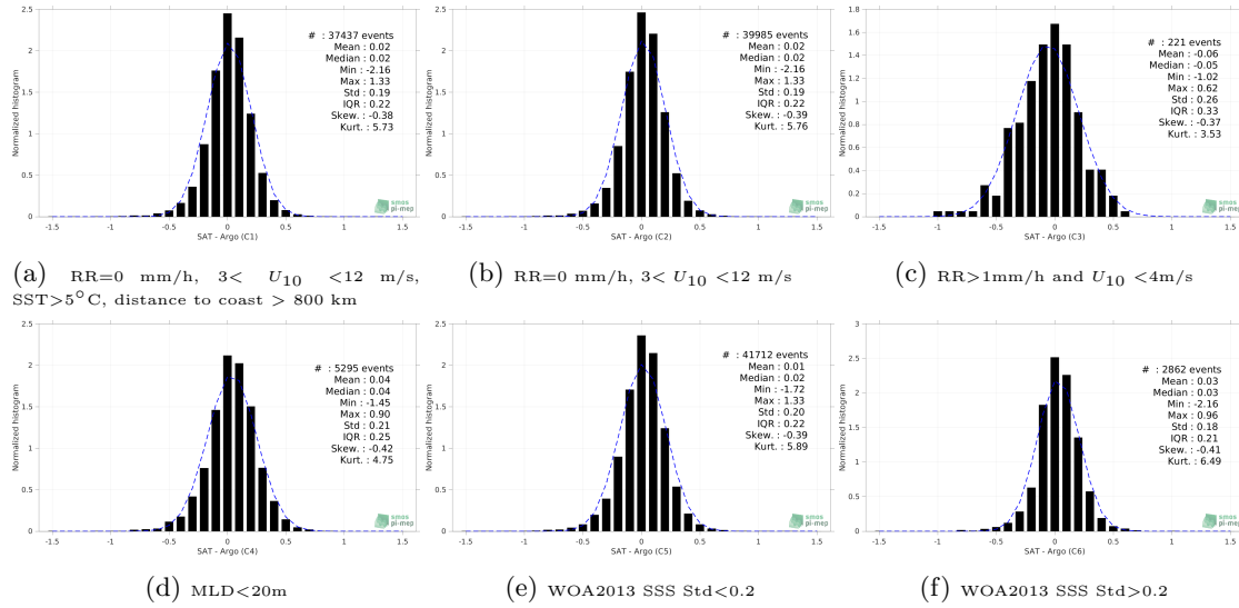
Figure 13: Normalized histogram of \Delta SSS (SMAP SSS L3 v5 - 8-Day running (RSS) - Argo) for 6 different subdatasets corresponding to: RR=0 mm/h, 3 < U_{10} < 12 m/s, SST > 5°C, distance to coast > 800 km (a), RR=0 mm/h, 3 < U_{10} < 12 m/s (b), RR > 1mm/h and U_{10} < 4 m/s (c), MLD < 20m (d), WOA2013 SSS Std < 0.2 (e), WOA2013 SSS Std > 0.2 (f).
