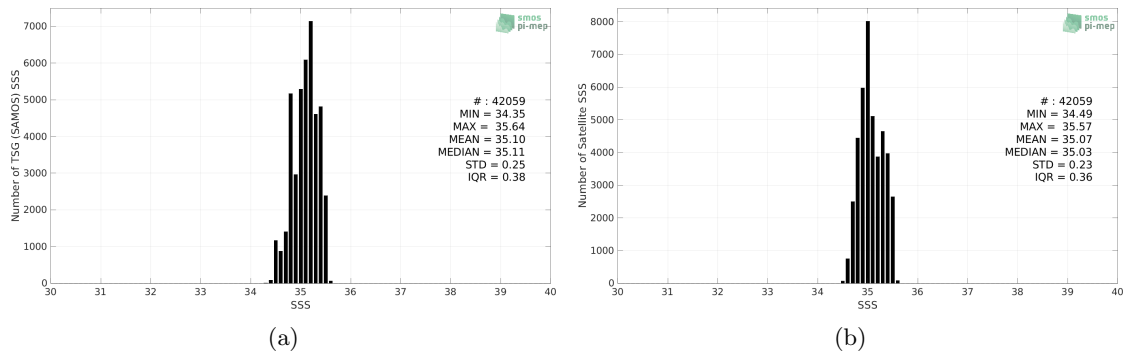
Figure 2: Histograms of SSS from TSG (SAMOS) (a) and SMAP SSS L3 v5 - Monthly (RSS) (b) considering all match-up pairs per bins of 0.1 over the OTT zone Pi-MEP region and for the full satellite product period.
