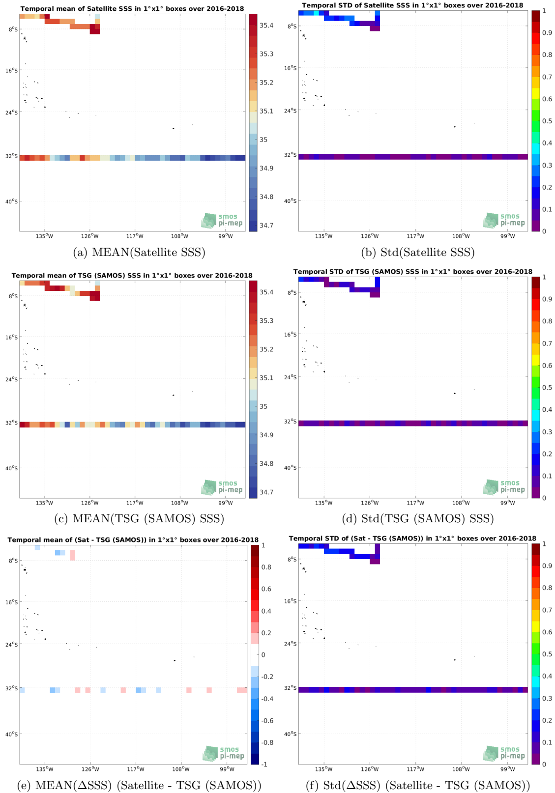
Figure 6: Temporal mean (left) and Std (right) of SSS from SMAP SSS L3 v5 - Monthly (RSS) (top), TSG (SAMOS) (middle), and of \Delta SSS (Satellite - TSG (SAMOS)). Only match-up pairs are used to generate these maps.
