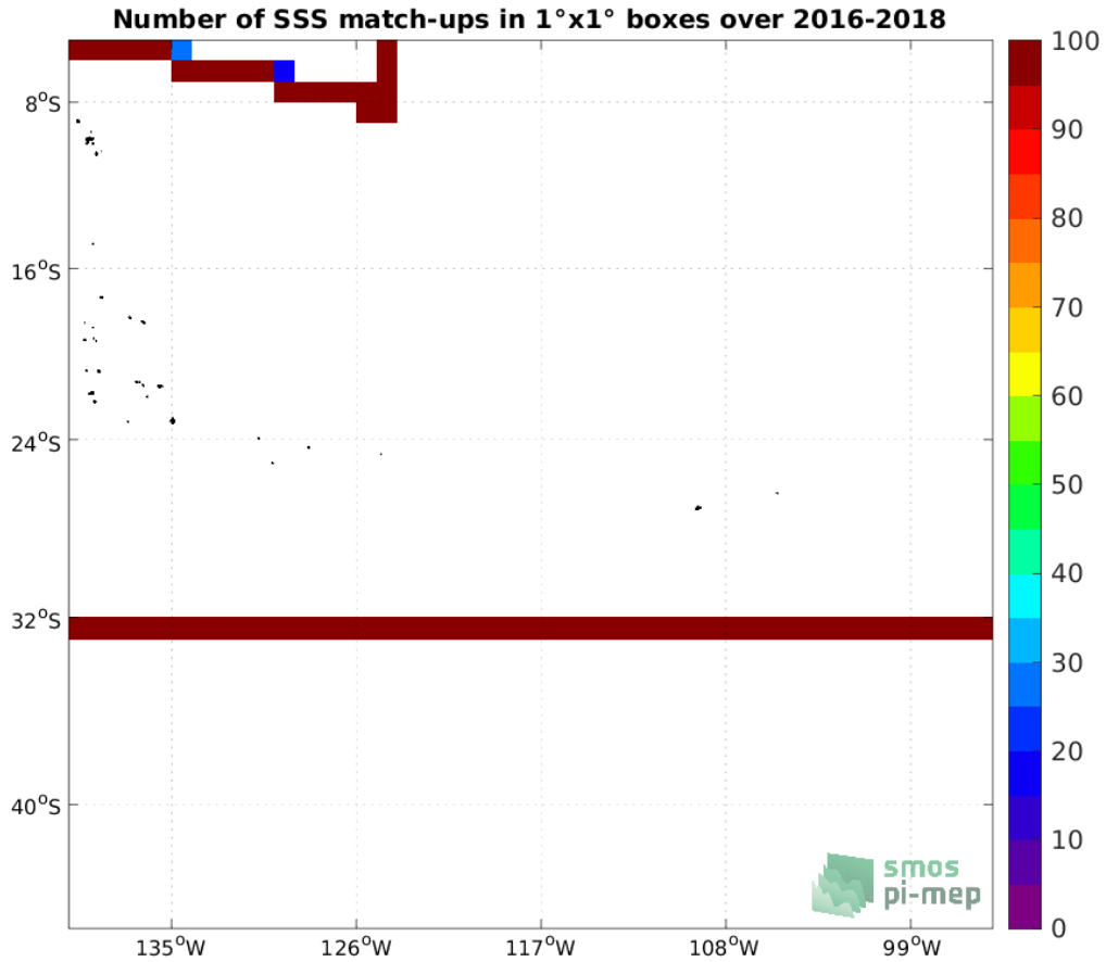
Figure 4: Number of SSS match-ups between TSG (SAMOS) SSS and the SMAP SSS L3 v5 - Monthly (RSS) SSS product for the OTT zone Pi-MEP region over 1^\circ \times 1^\circ boxes and for the full satellite product period.
