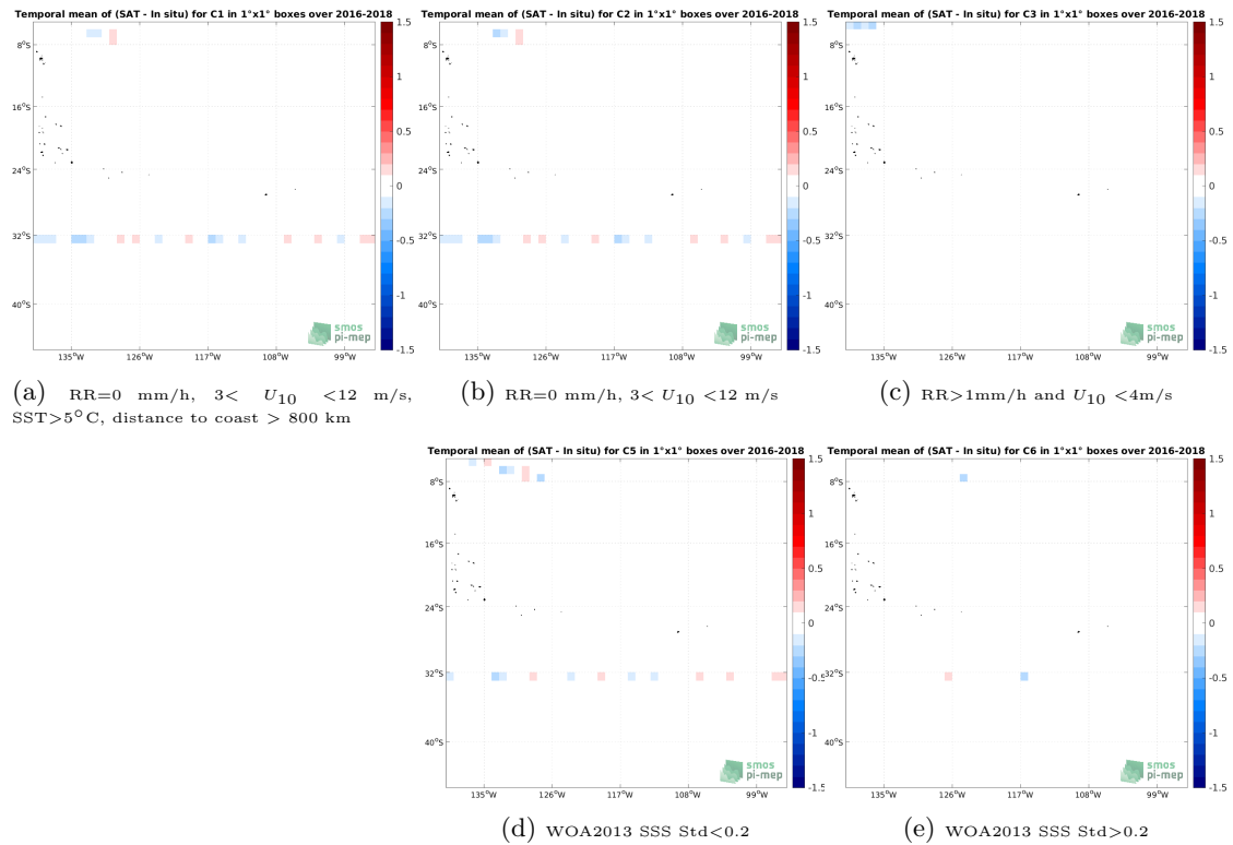
Figure 12: Temporal mean gridded over spatial boxes of size 1^\circ \times 1^\circ of \Delta SSS (SMAP SSS L3 v5 - Monthly (RSS) - TSG (SAMOS)) for 5 different subdatasets corresponding to: RR=0 mm/h, 3 < U_{10} < 12 m/s, SST > 5^\circ C , distance to coast > 800 km (a), RR=0 mm/h, 3 < U_{10} < 12 m/s (b), RR > 1 mm/h and U_{10} < 4 m/s (c), WOA2013 SSS Std < 0.2 (d), WOA2013 SSS Std > 0.2 (e).
