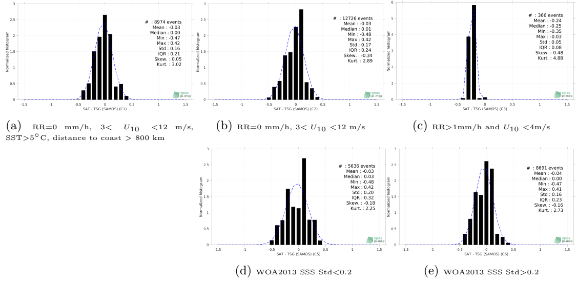
Figure 13: Normalized histogram of \Delta\text{SSS} (SMAP SSS L3 v5 - Monthly (RSS) - TSG (SAMOS)) for 5 different subdatasets corresponding to: RR=0 mm/h, 3 < U_{10} < 12 m/s, SST>5°C, distance to coast > 800 km (a), RR=0 mm/h, 3 < U_{10} < 12 m/s (b), RR>1mm/h and U_{10} < 4 m/s (c), WOA2013 SSS Std<0.2 (d), WOA2013 SSS Std>0.2 (e).
